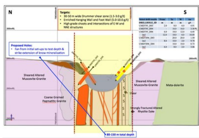
Fig. 4 Drummer Toy proposed drill holes with current conceptual cross section (CNW Group/Essex Minerals Inc)
