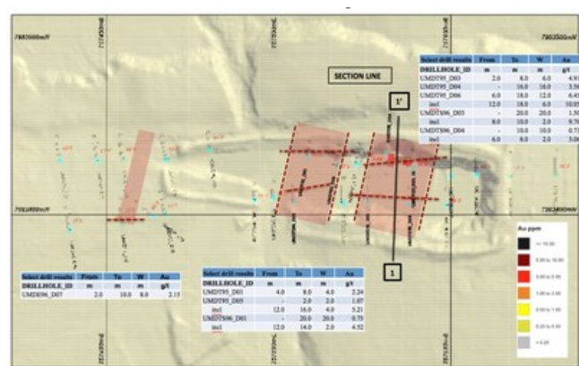
Fig. 3 Drummer Toy pit with historic drill locations and select results (CNW Group/Essex Minerals Inc)
