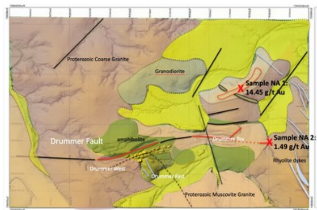
Fig. 1 Magnetic lines, eastern Drummer Fault - with sample locations (CNW Group/Essex Minerals Inc)
