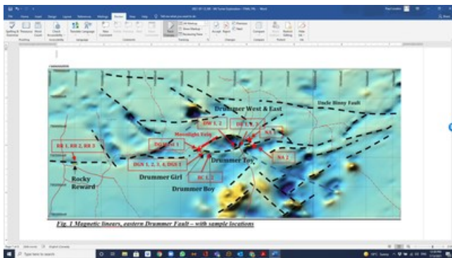
Fig. 1 Magnetic lines, eastern Drummer Fault - with sample locations (CNW Group/Essex Minerals Inc)
