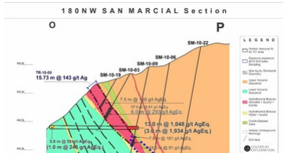
Figure 2: San Marcial Cross Section O-P (CNW Group/Goldplay Exploration Ltd)
