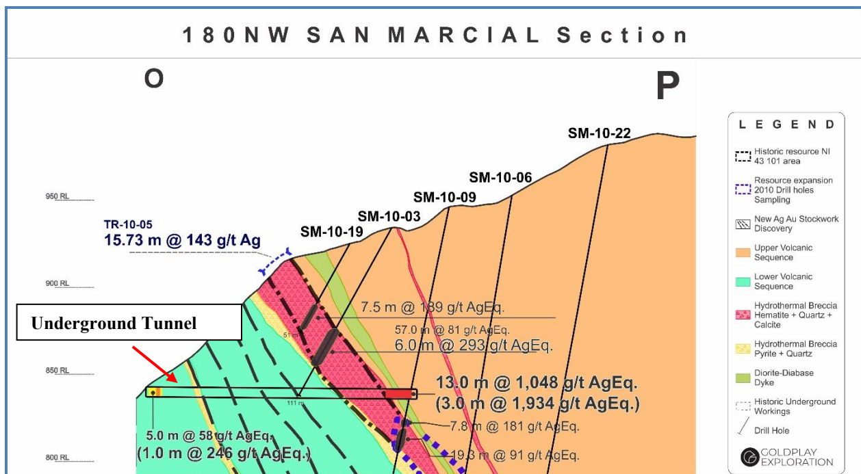
Figure 2: San Marcial Cross Section O-P
