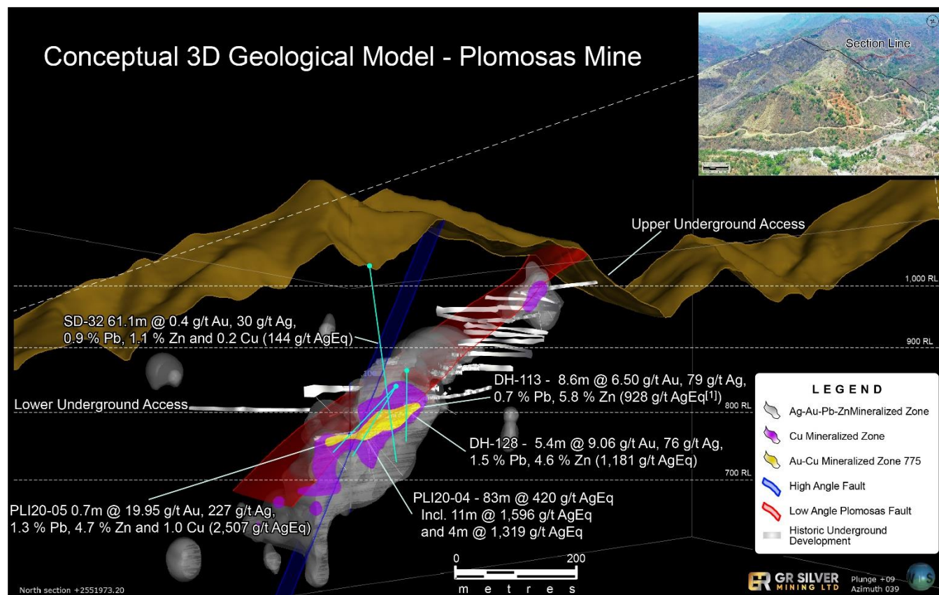
Figure 1: Location Map - 3D Image of the Plomosas Mine Area Drilling Location
