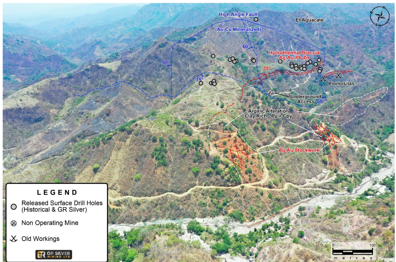
Figure 2: Drone Image Plomositas Mine – Local Geology Showing Argillic Altered (Clay-rich) Zones
