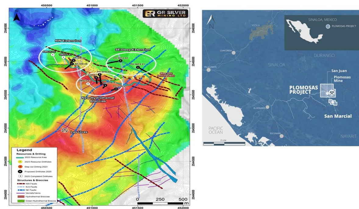
Figure 1 – Chargeability Geophysical Anomaly and Drilling Targets – Associated Faults
