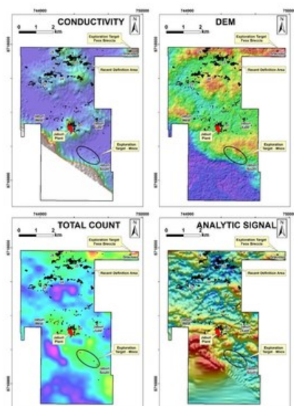
Figure 2: Clockwise from top left: HeliTEM Conductivity Grid, Digital Elevation Model, Analytic Signal Magnetics and Total Count Radiometrics. Manganese occurrences in mapping and preproduction. (CNW Group/Meridian Mining S.E.)
