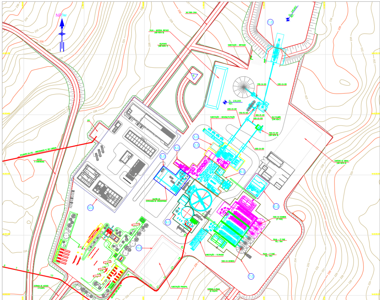
Figure 5: Cabaçal process plant layout
