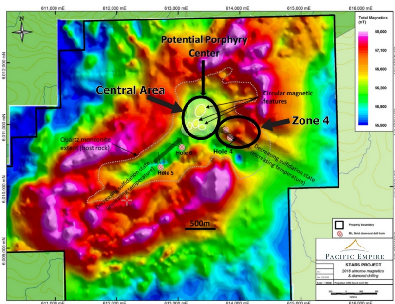
Figure 1: 2018 Partner-Funded Diamond Drilling and Airborne Magnetics at the Stars Copper Property
