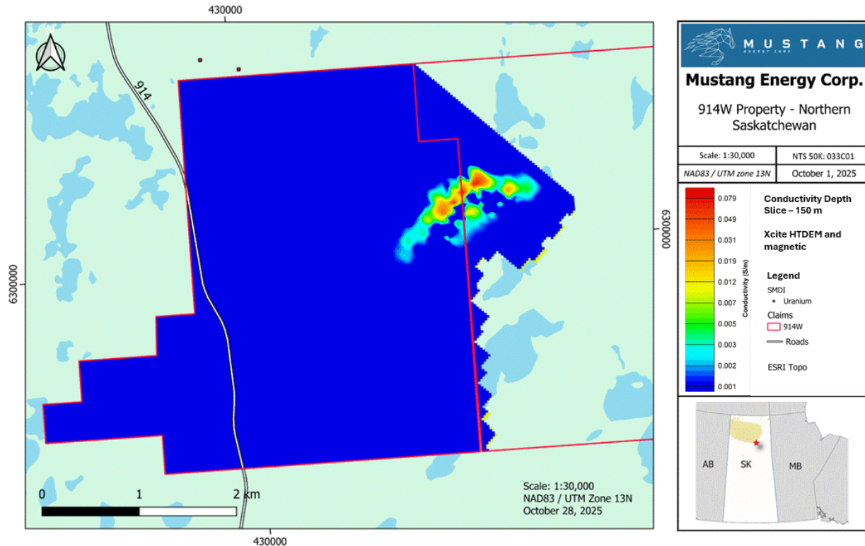
Figure 2: Airborne HTDEM survey over 914W project showing EM responses from conductivity depth slice at 150 m showing a high response along the east-central portion of the 914W block.
