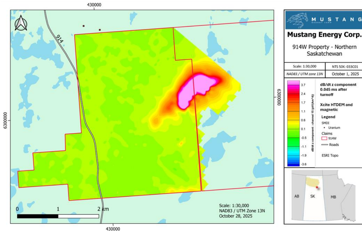
Figure 1: Airborne HTDEM survey over 914W project showing time channels 0.045 ms with strong, high-amplitude EM responses along the east-central portion of the 914W block.
