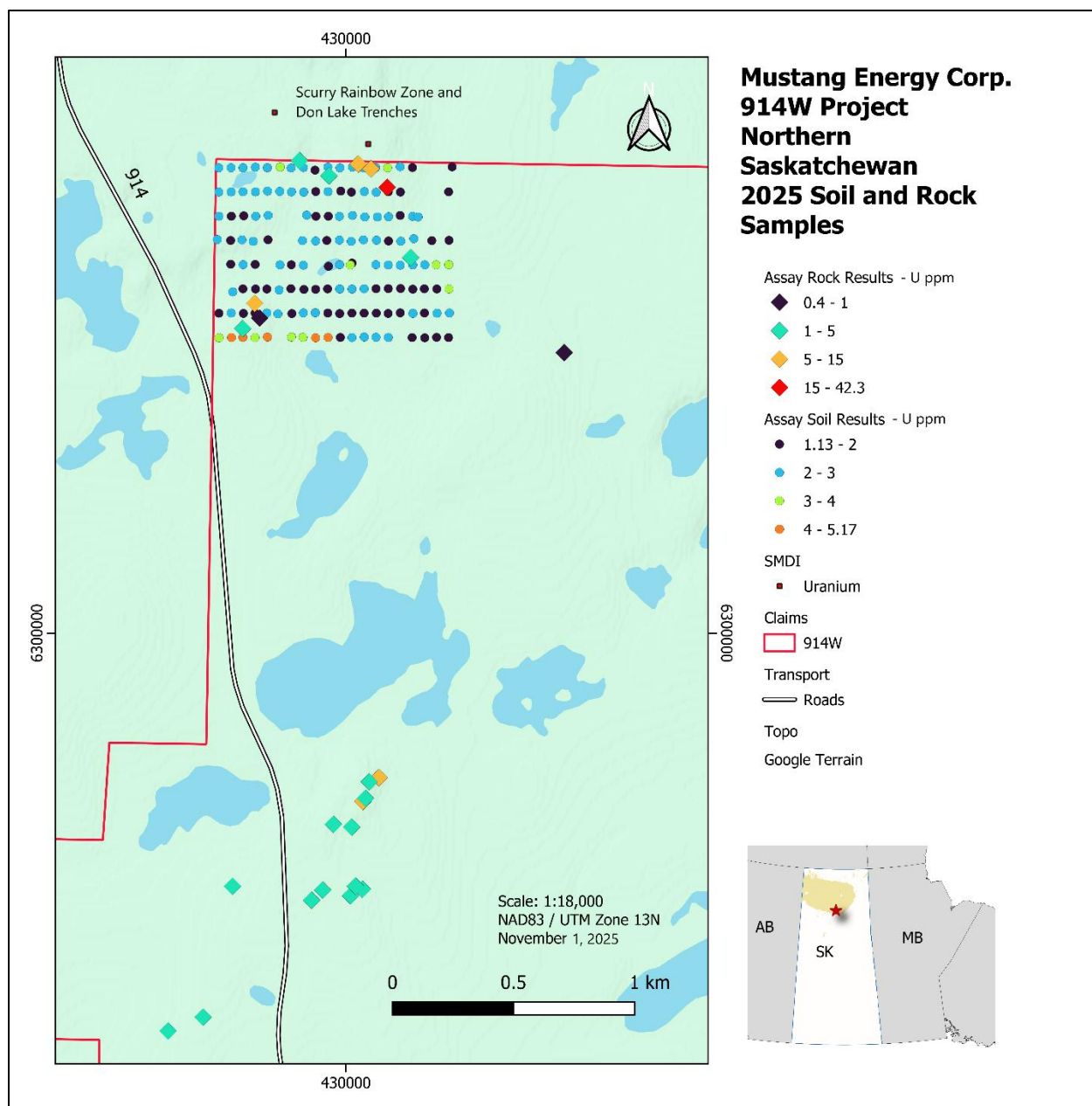
Figure 3: 2025 914W Project soil and rock sample assay results – U ppm
