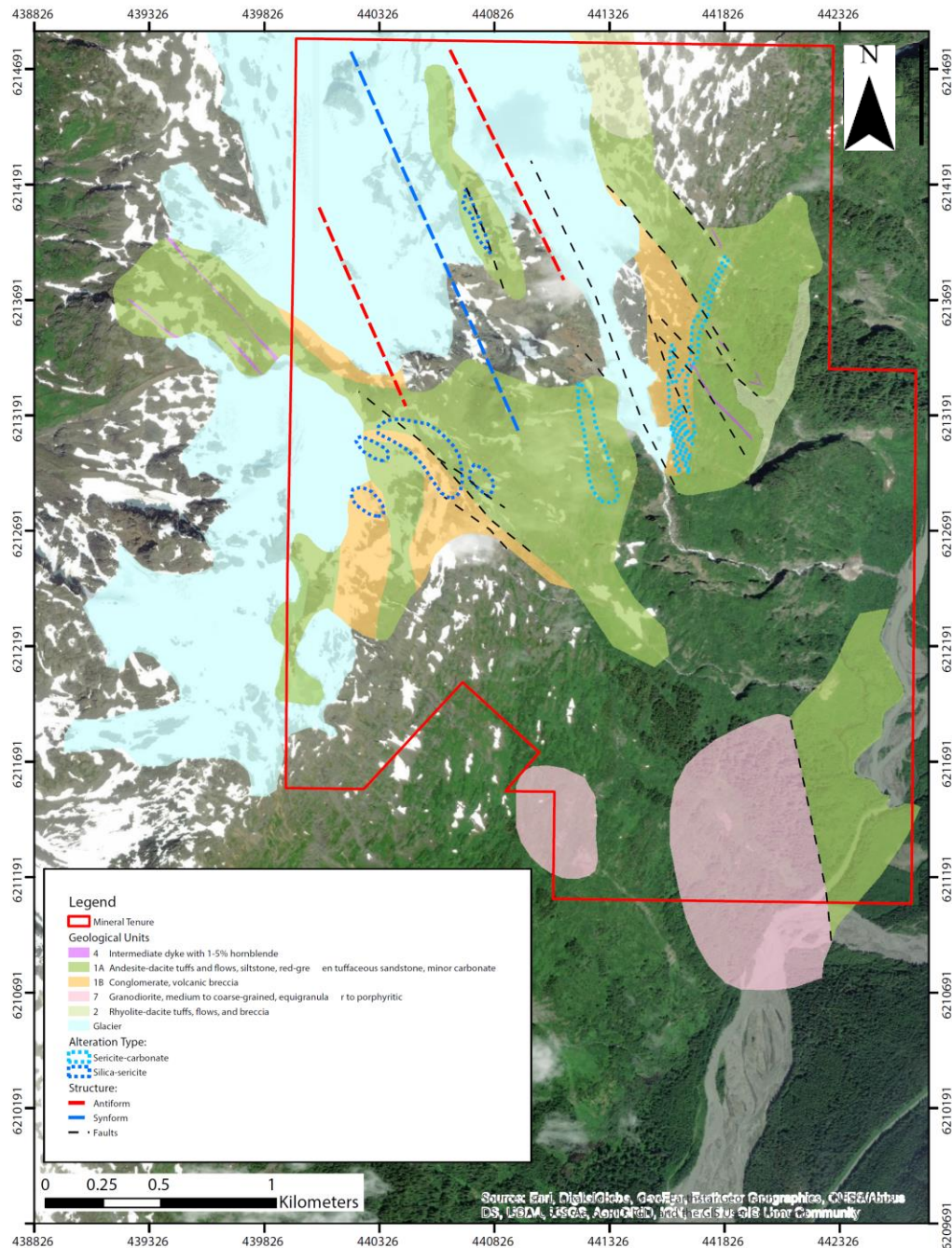
Figure 7-2: Interpreted property geology of the MC property showing approximated lithological contacts of the Unuk River (Units 1), Betty Creek Formation (Unit 2), Portland Canal Dykes (4), Texas Creek Granodiorite (Unit 7). Map data compiled from assessment reports by Kikauka (1990, 2000, 2003). 1:20000 scale.
