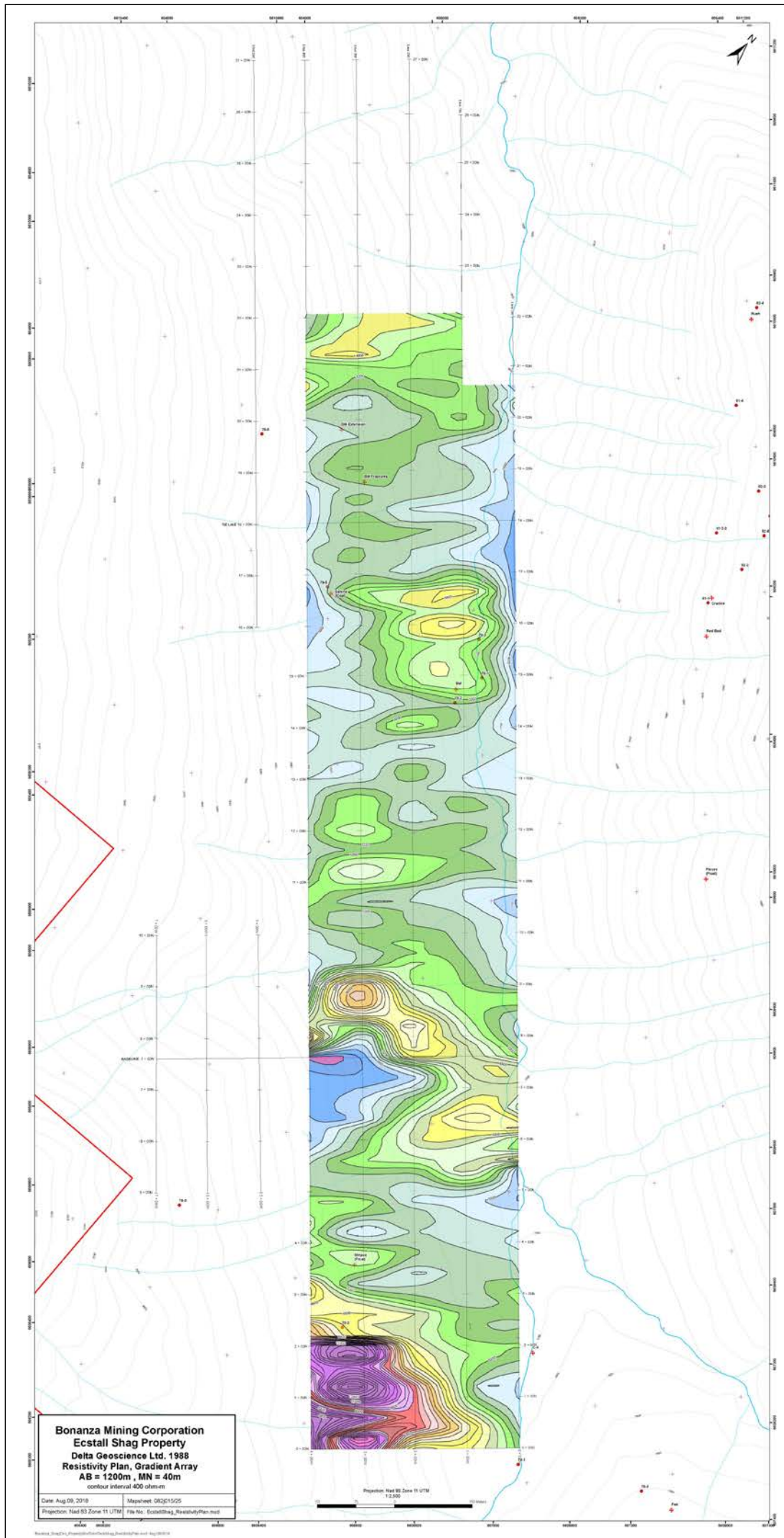
Figure 9-2 Resistivity Plan, Gradient Array
