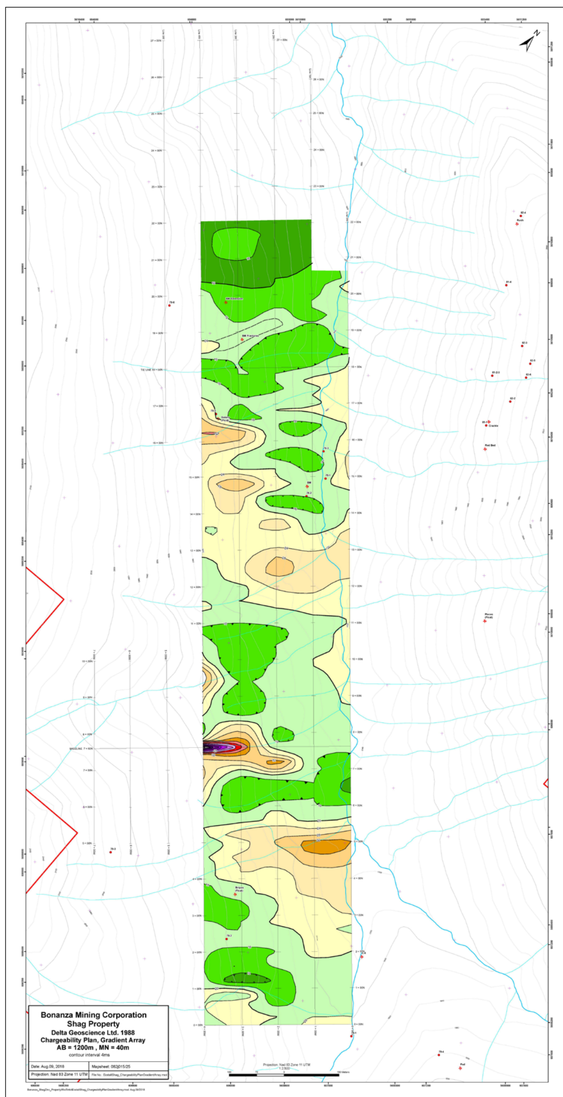
Figure 9-1 Chargeability Plan, Gradient Array
