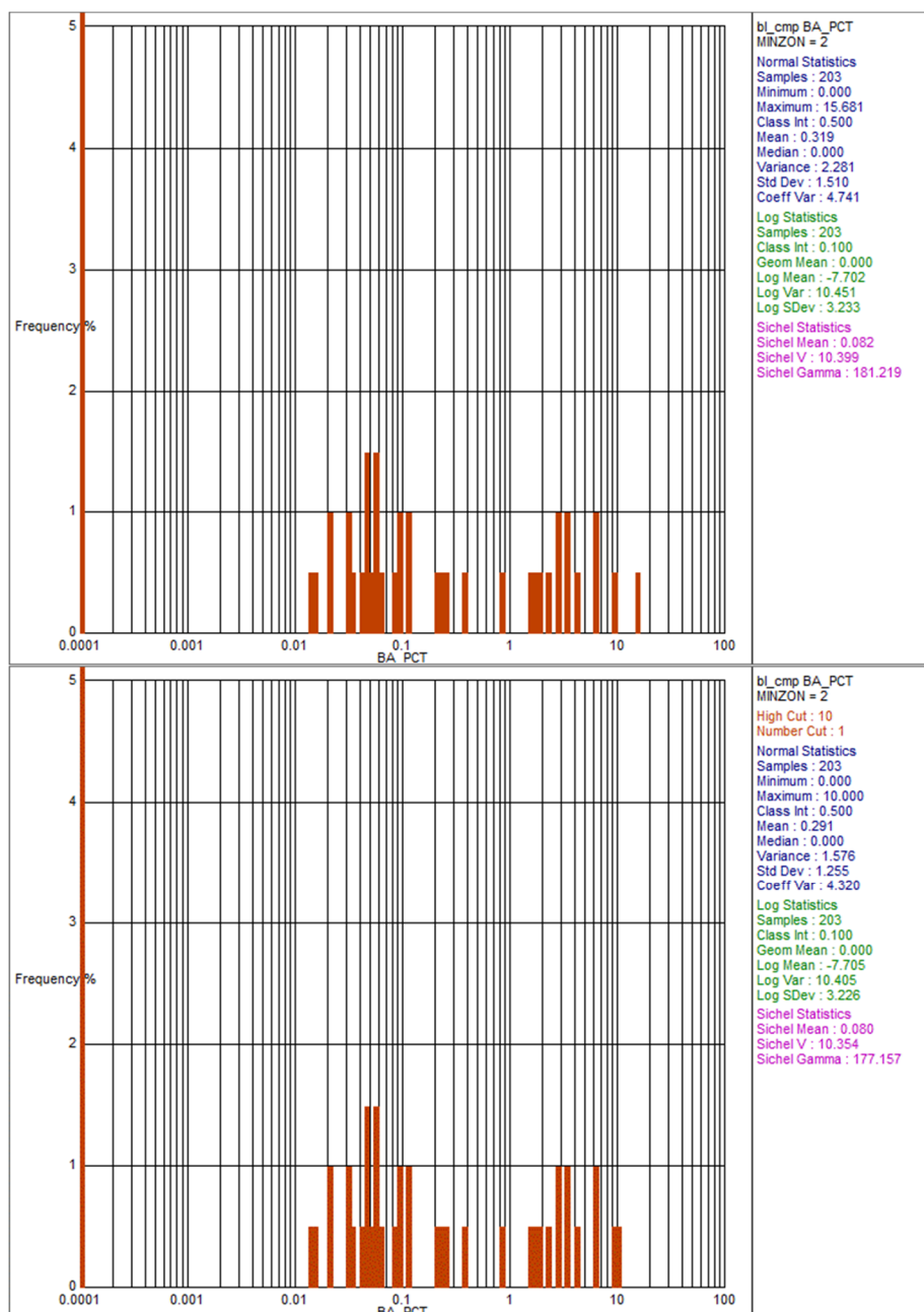
Figure 14.17 BaSO 4 % (MINZON = 2) - Log Histogram Plots Uncut (top) and Top-Cut (bottom) (Source: CSA Global, 2018)
