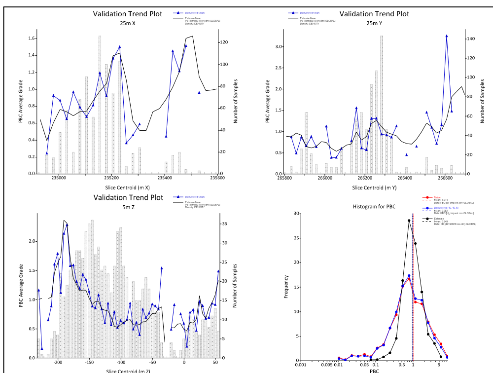
Figure 14.28 Pb% Swath plots and histogram, block model (black) vs. declustered composites (blue) (MINZONs 1-18)
