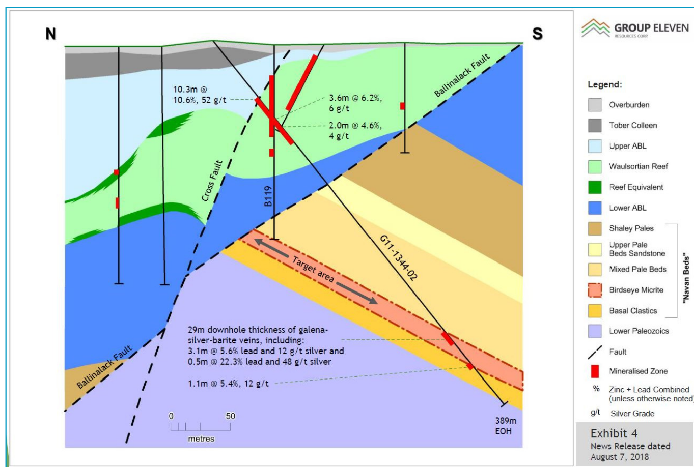
Figure 10.3 Cross section through drillhole G11-1344-02
