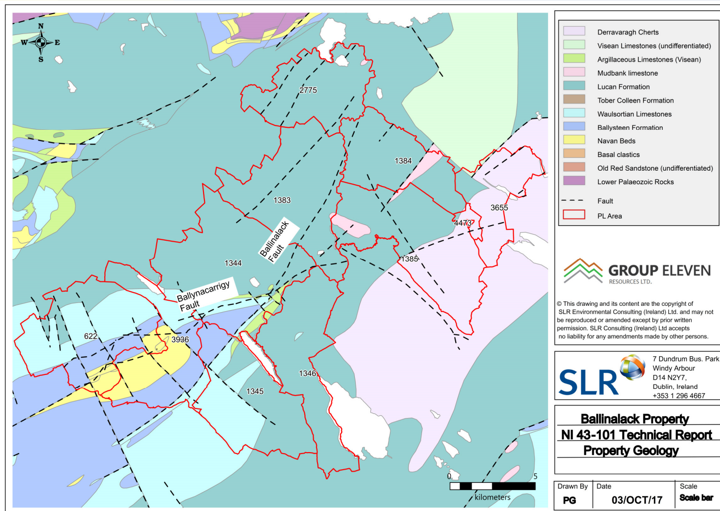
Figure 7.3 Ballinalack Project Geology
