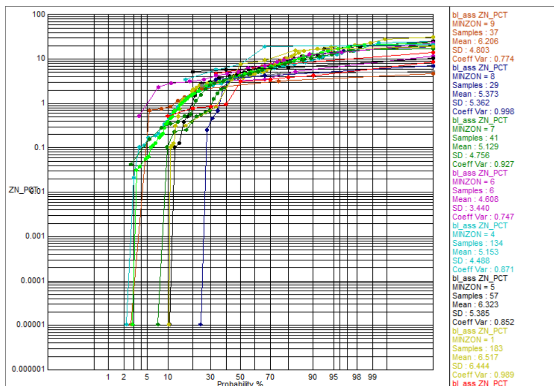
Figure 14.4 Naïve Zn% - Log probability plot overlays of mineralisation per MINZON
