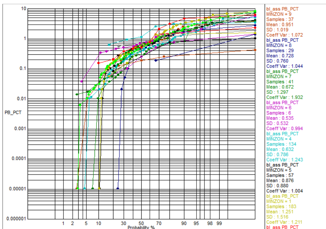
Figure 14.5 Naïve Pb% - Log probability plot overlays of mineralisation per MINZON (Source: CSA Global, 2018)
