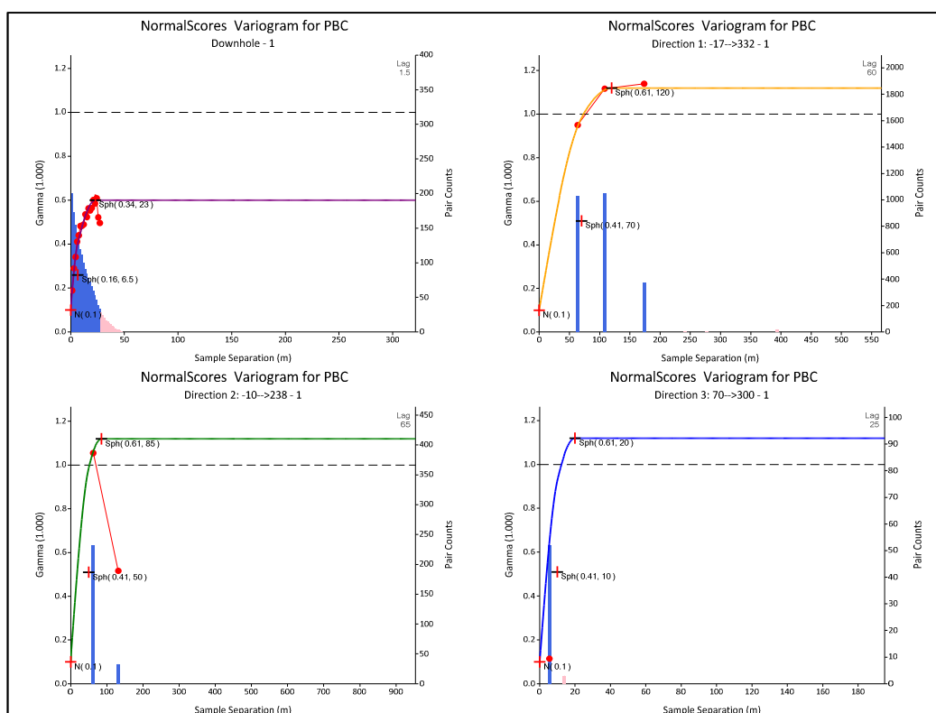
Figure 14.19 Variogram used for Pb% estimation
