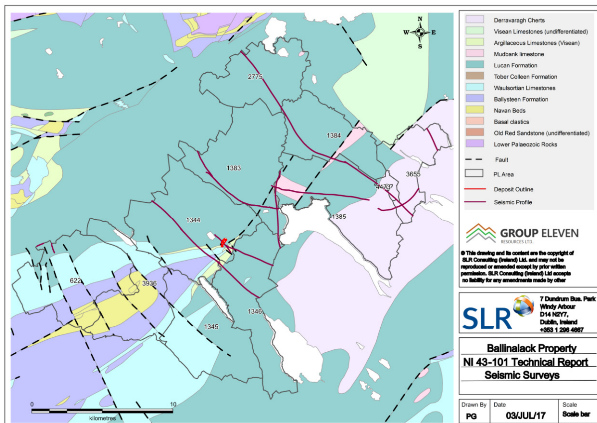
Figure 6.4 Seismic surveying completed by TIL
