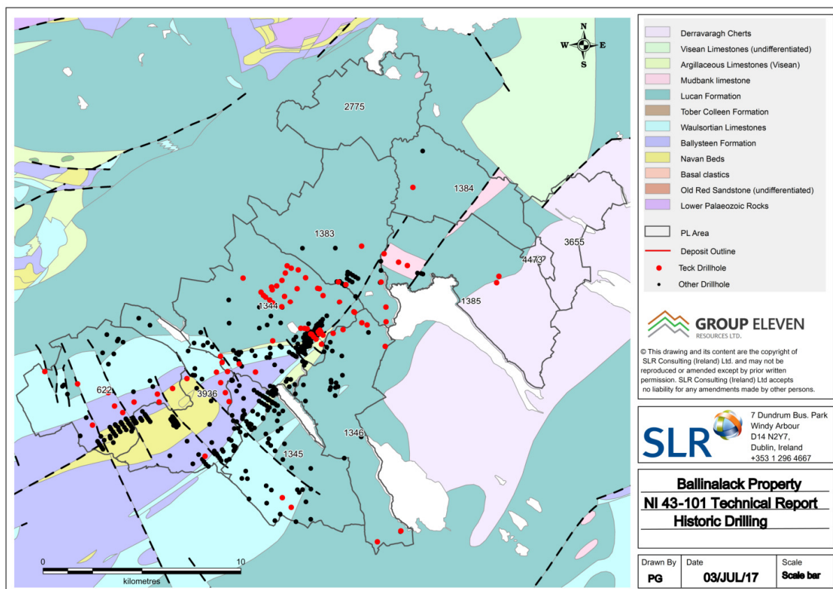
Figure 6.3 Previous drilling on Ballinalack group of PLs.
