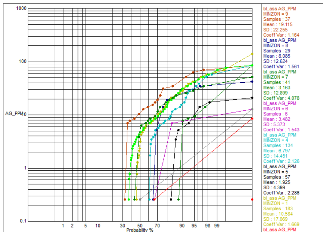
Figure 14.6 Naïve Ag g/t - Log probability plot overlays of mineralisation per MINZON (Source: CSA Global, 2018)
