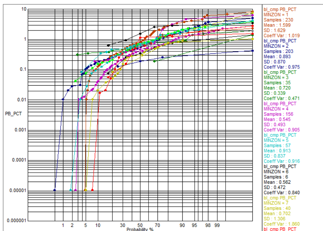
Figure 14.11 Composite Pb% - Log probability plot overlays of mineralisation per MINZON
