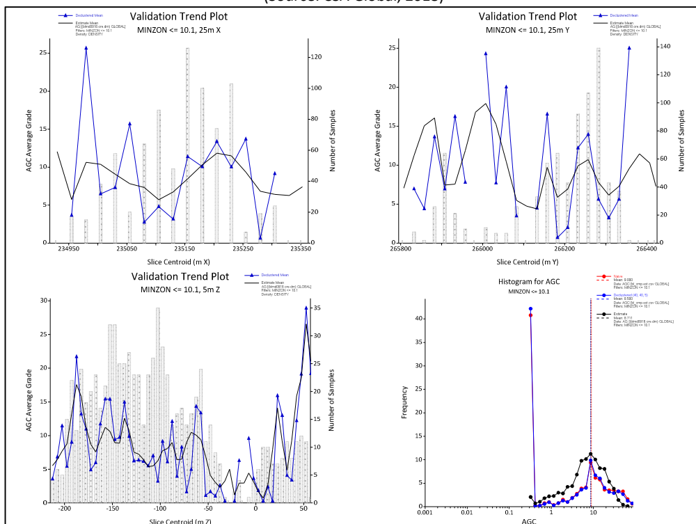
Figure 14.29 Ag g/t Swath plots and histogram, block model (black) vs. declustered composites (blue) (MINZONs 1-10)
