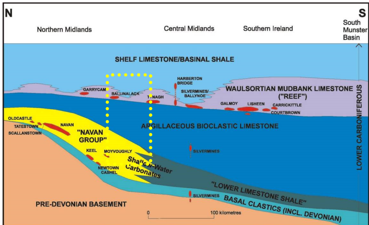
Figure 8.1 Stratigraphic location of Carboniferous-hosted Mineralisation in Ireland. Ballinalack area highlighted
