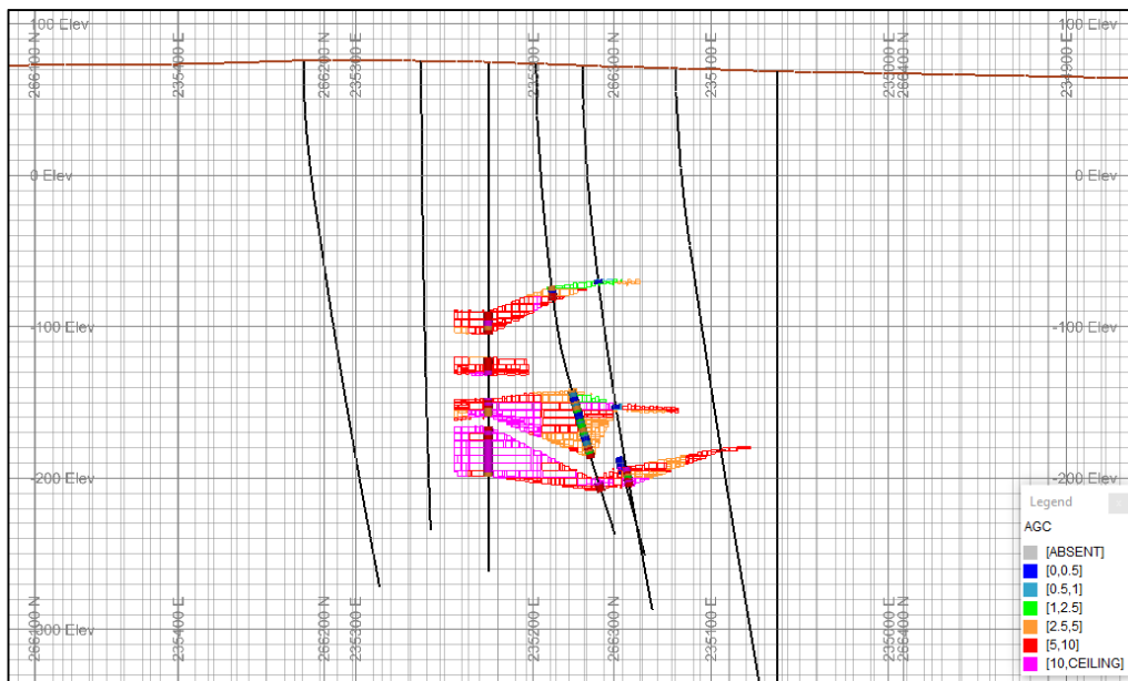
Figure 14.25 Section view – Ag g/t Grade Model and composites
