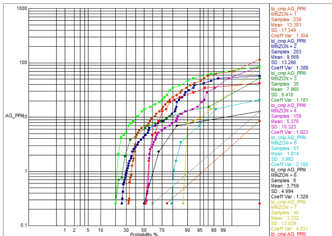
Figure 14.12 Composite Ag g/t - Log probability plot overlays of mineralisation per MINZON
