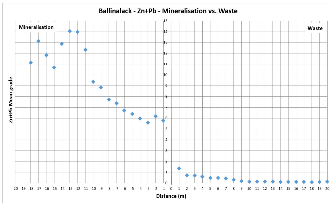
Figure 14.3 Boundary test graph for Ballinalack – Zn+Pb% mineralisation versus Waste.
