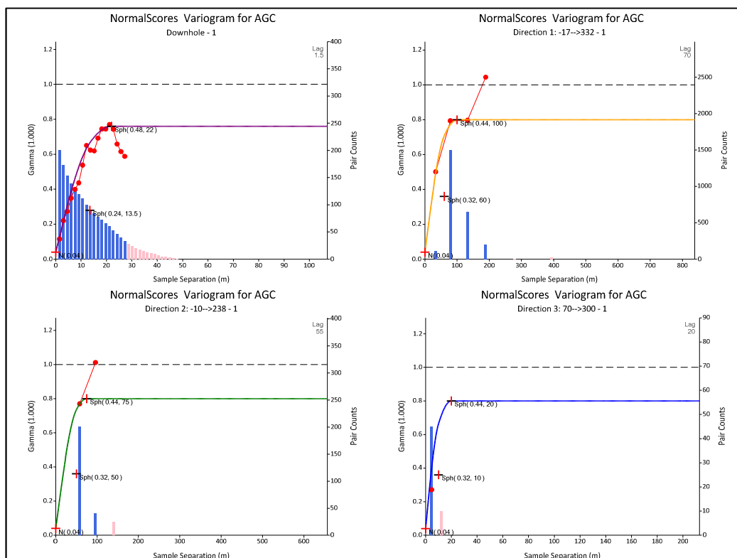
Figure 14.20 Variogram used for Ag g/t estimation
