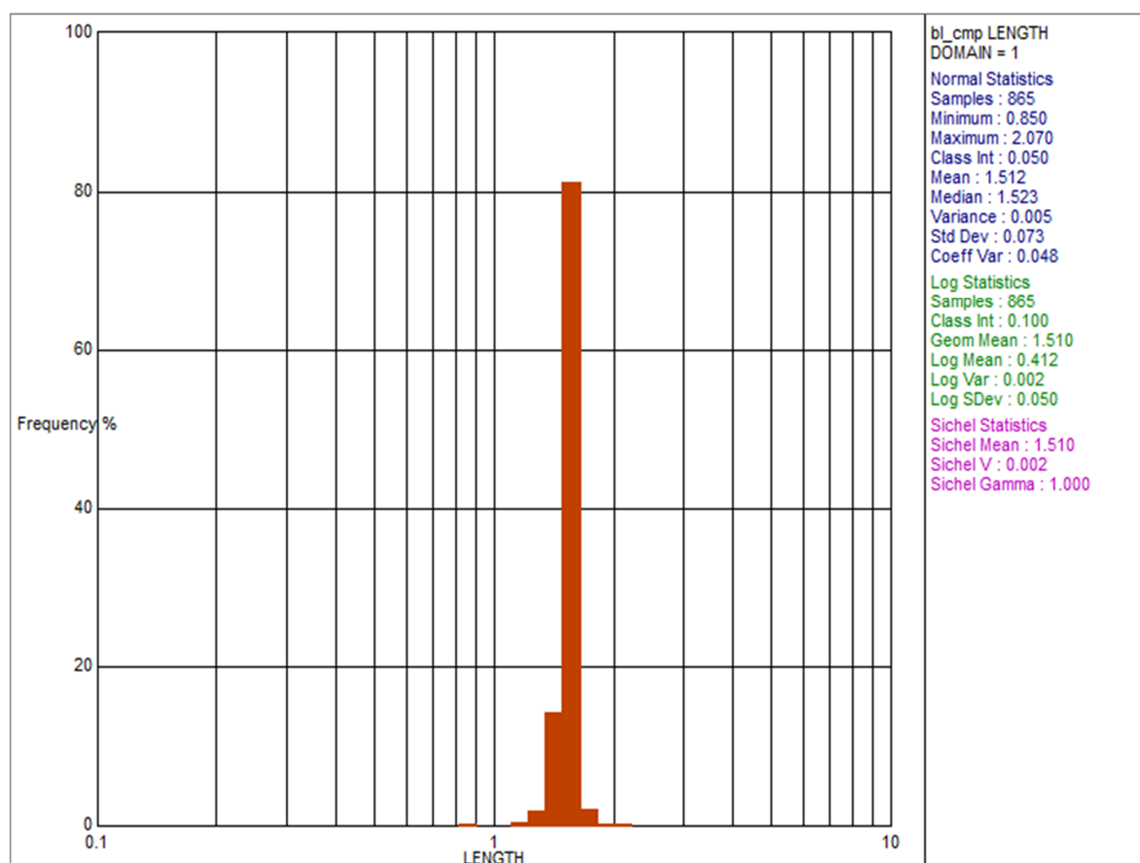
Figure 14.9 Log Normal Histogram of composite lengths for mineralisation (DOMAIN = 1)
