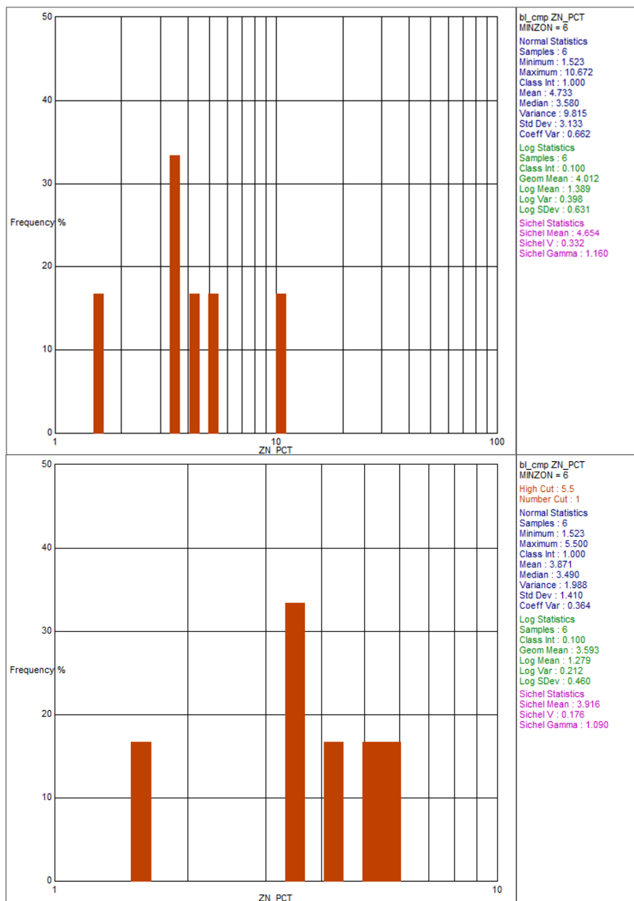
Figure 14.14 Zn% (MINZON = 6) - Log Histogram Plots Uncut (top) and Top-Cut (bottom)
