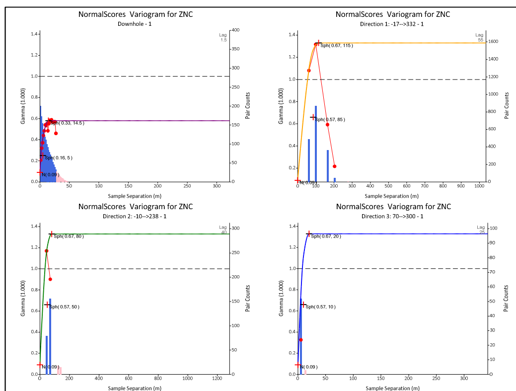
Figure 14.18 Variogram used for Zn% estimation
