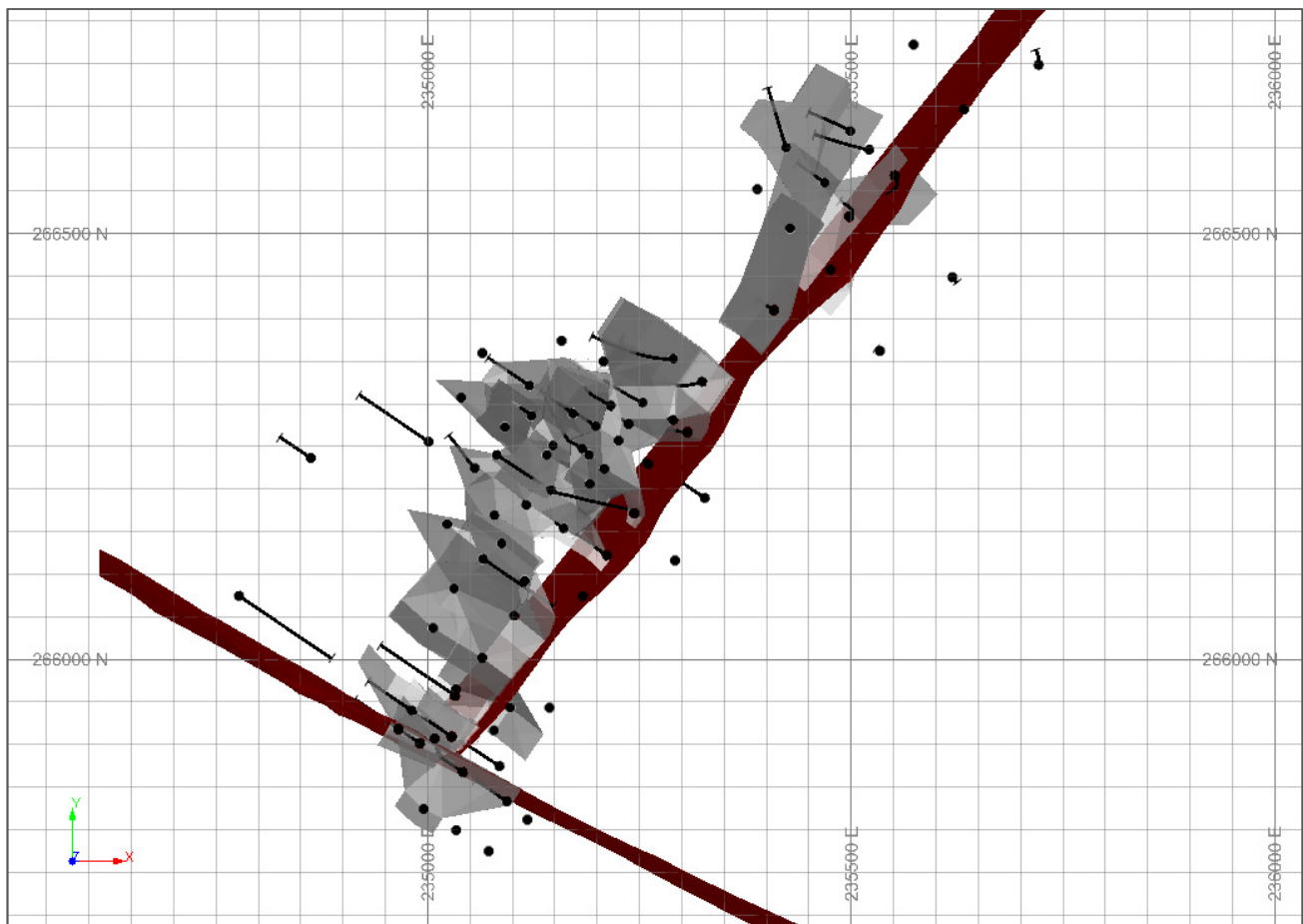
Figure 14.2 Plan view of mineralized wireframes (grey), inferred faults (red) with drillholes
