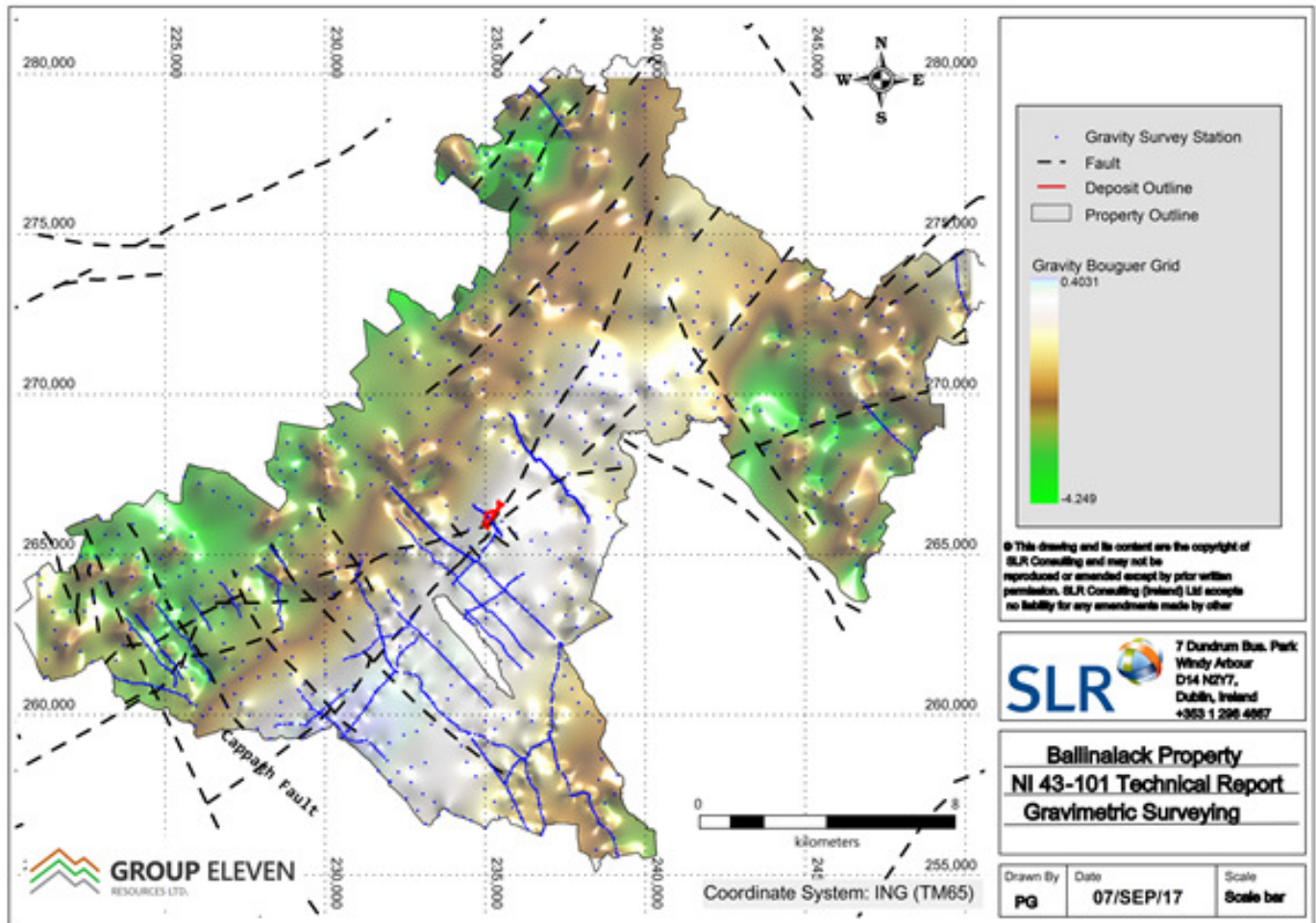
Figure 9.3 Gravity anomalism (based on ground surveys) on the Ballinalack Project, Ireland
