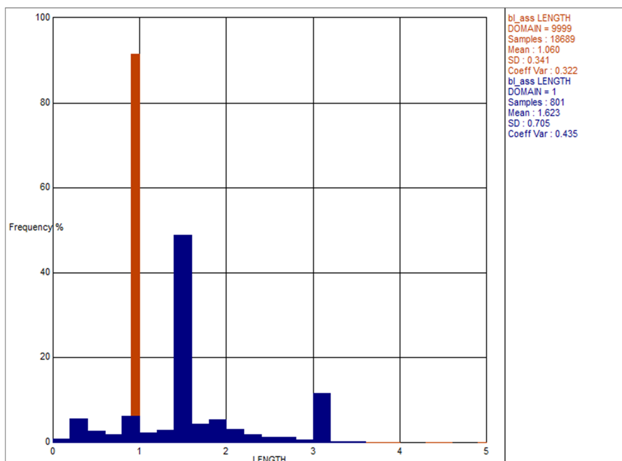
Figure 14.8 Histogram overlay of sample lengths for mineralisation (Blue; DOMAIN = 1) versus Waste (Red; DOMAIN = 9999)
