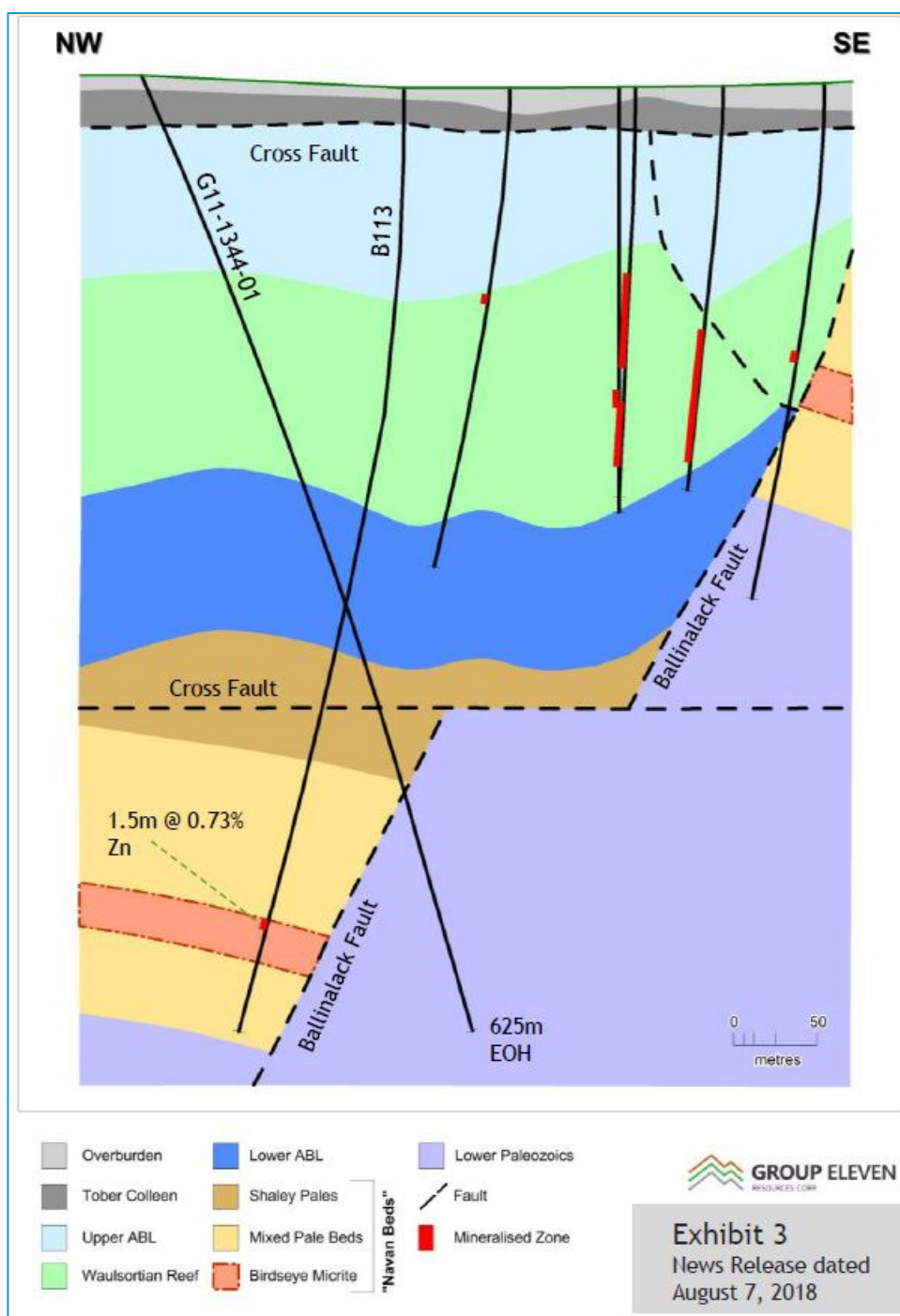
Figure 10.2 Cross section through drillhole G11-1344-01
