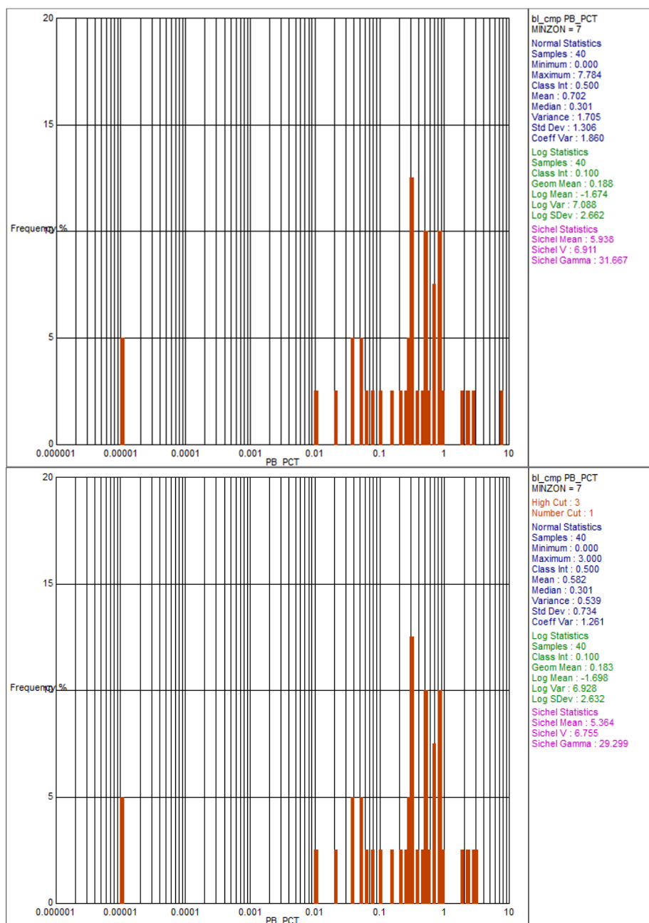
Figure 14.15 Pb% (MINZON = 7) - Log Histogram Plots Uncut (top) and Top-Cut (bottom)
