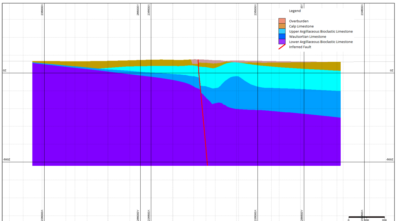
Figure 14.1 Type cross section showing general stratigraphy
