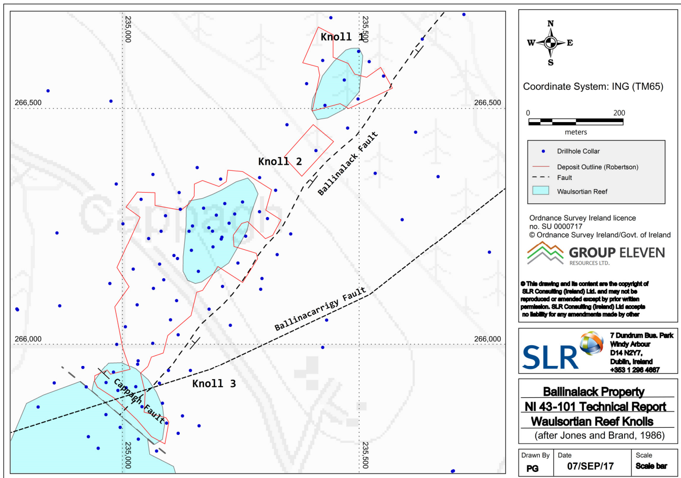
Figure 7.2 Waulsortian knolls at Ballinalack, modified from Jones and Brand (1986)
