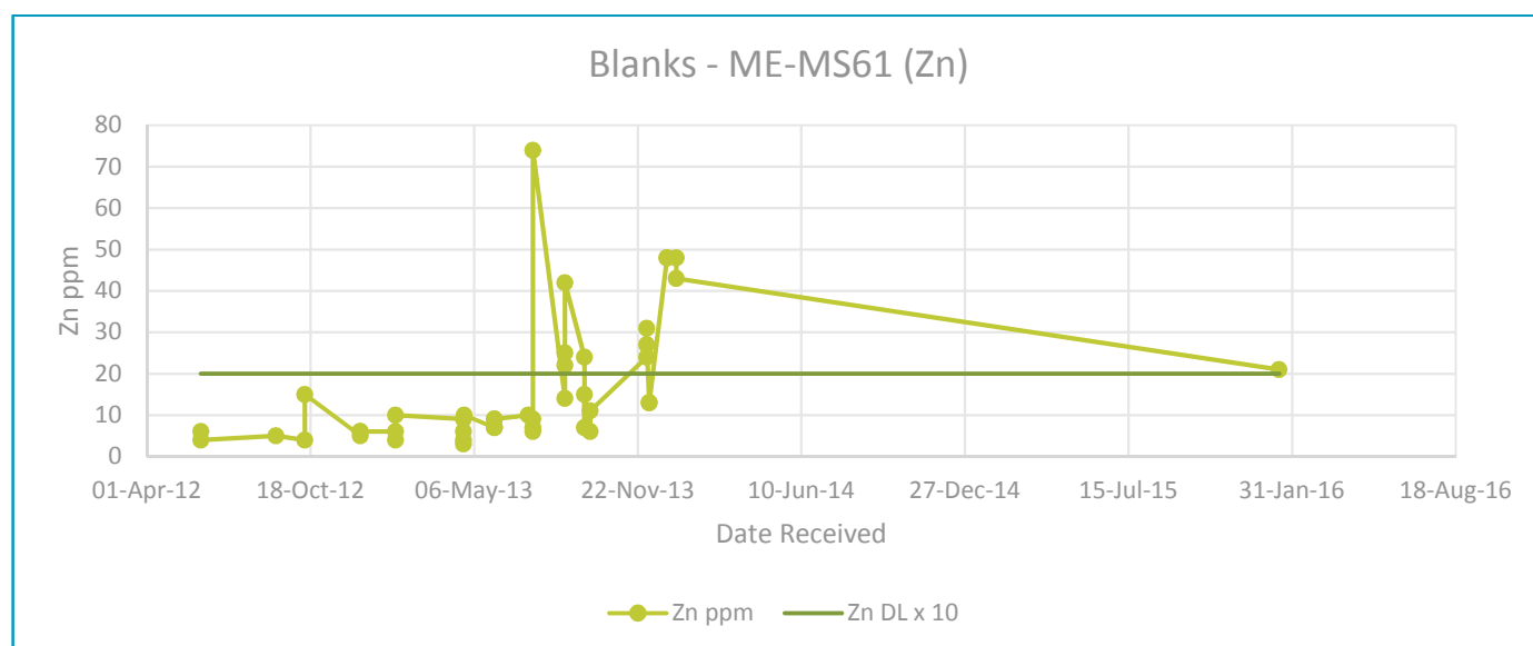
Figure 11.13 Chart showing Zn results for blank samples, using ME-MS61
