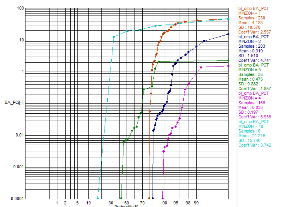
Figure 14.13 Composite BaSO 4 % - Log probability plot overlays of mineralisation per MINZON
