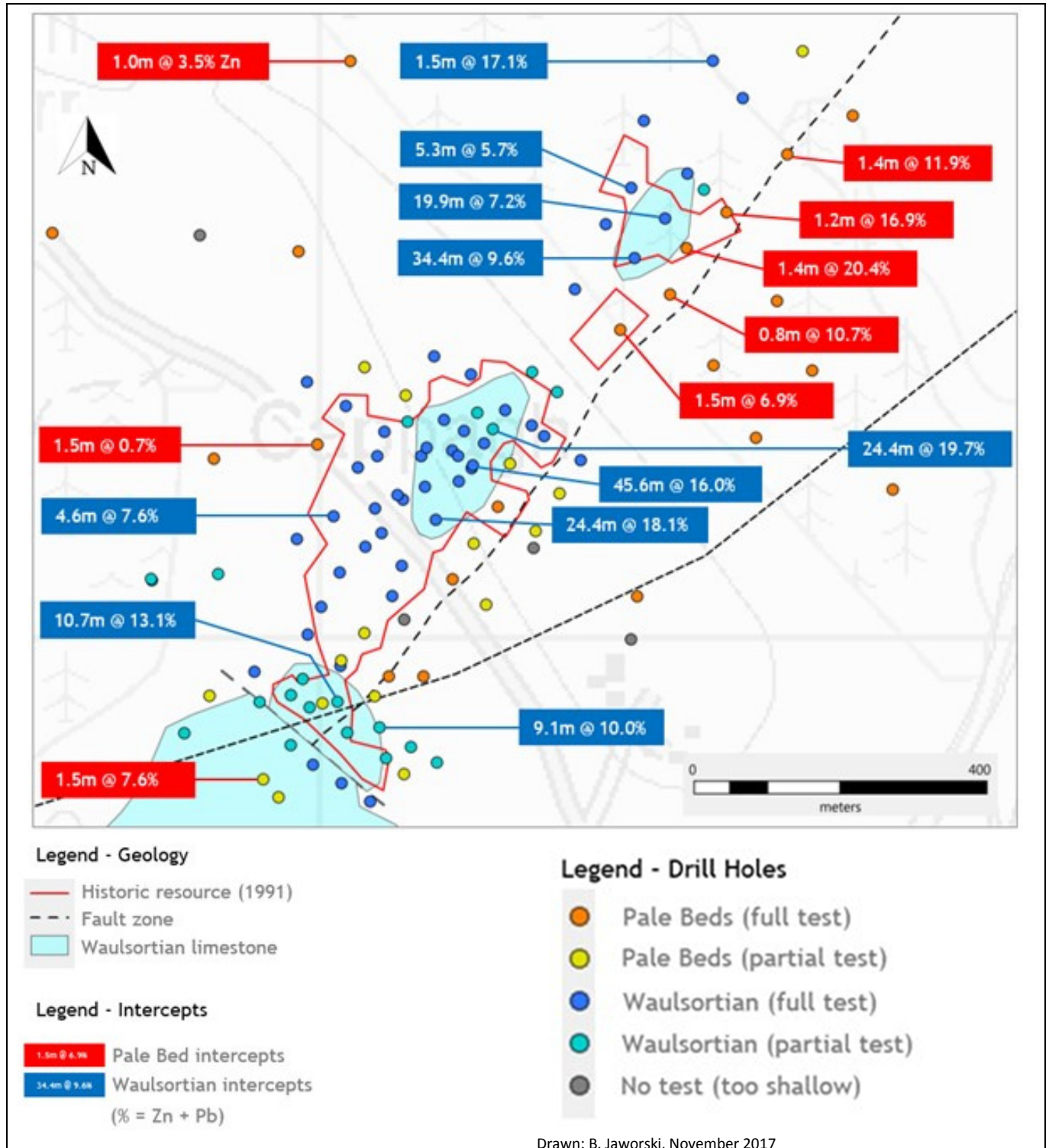
Figure 6.1 Plan map of drillhole intercepts with key intercepts labelled.
