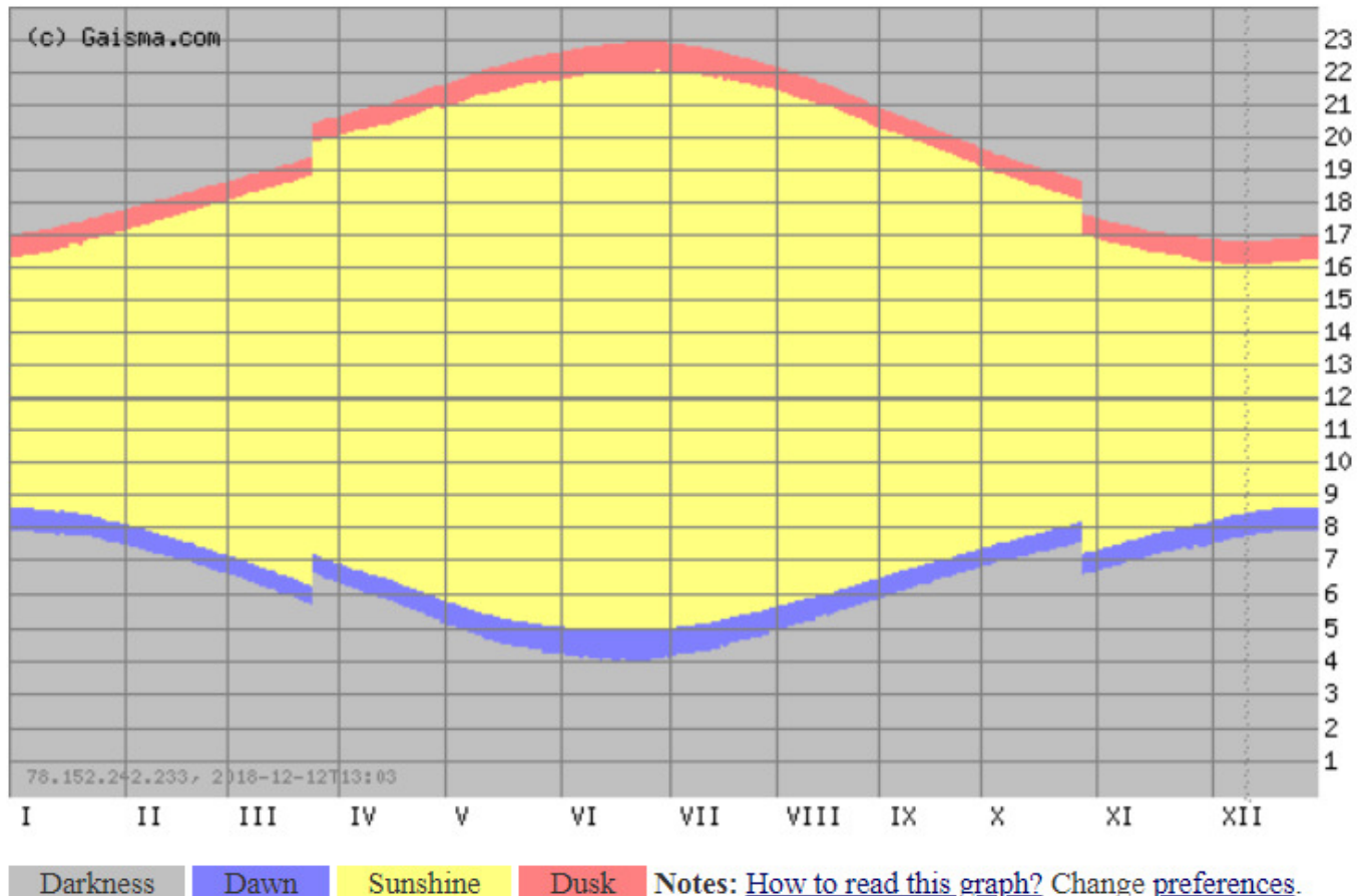
Figure 5.2 Ballinalack graph of sunrise, sunset
