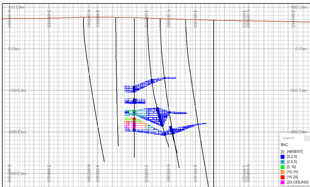
Figure 14.26 Section view – BaSO 4 % Grade Model and composites
