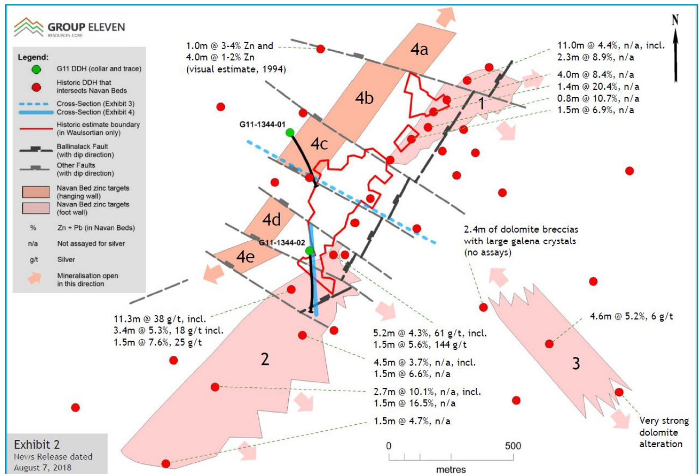
Figure 10.1 Location of target areas and recent drillholes on the Project.
