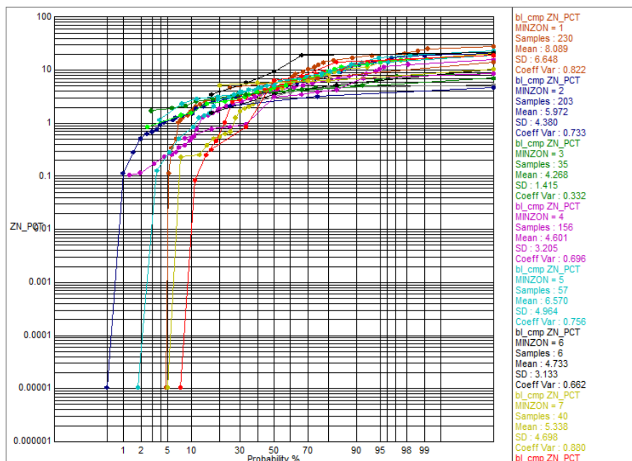
Figure 14.10 Composite Zn% - Log probability plot overlays of mineralisation per MINZON
