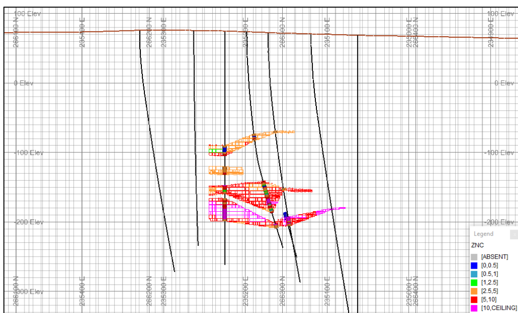
Figure 14.23 Section view – Zn% Grade Model and composites
