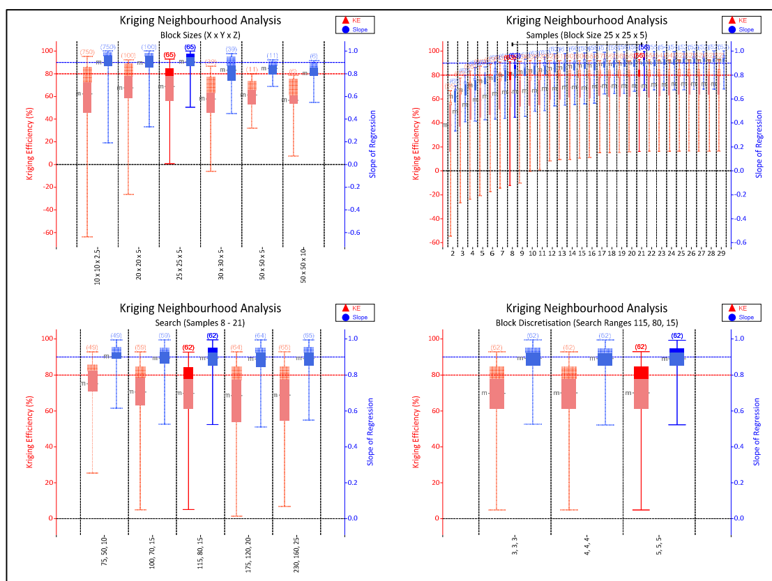
Figure 14.22 KNA block size, samples, search and discretisation results for Zn% estimation
