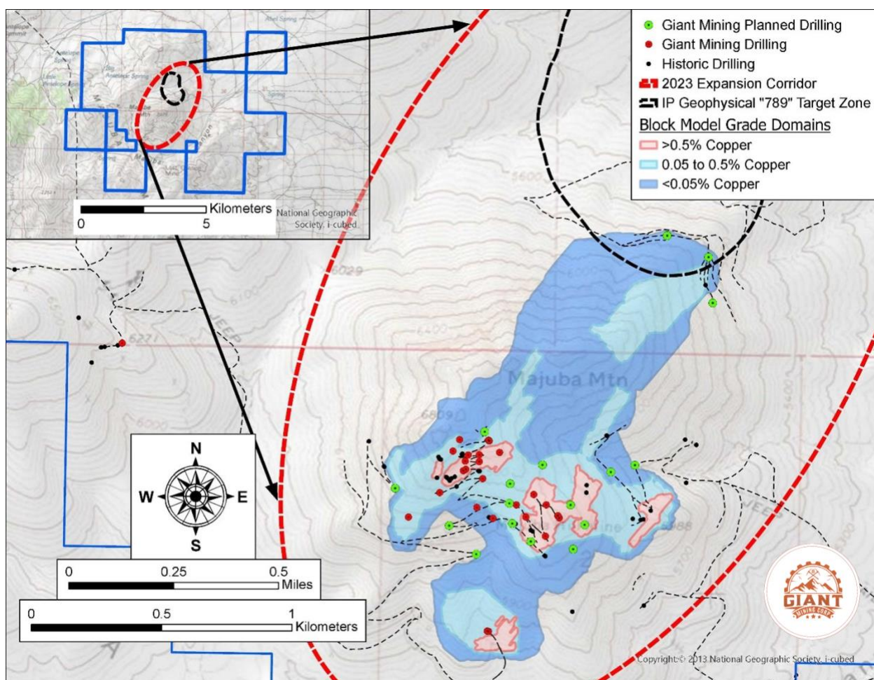
Figure 6: Giant Mining grade domain with recent, historic and planned drilling.
