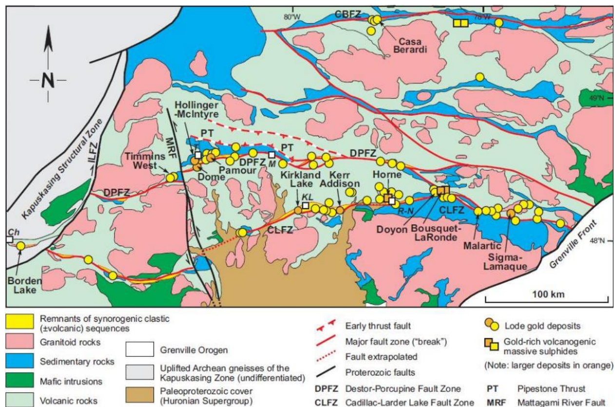
Figure 7.1: Geologic Map of the Southern and Central Abitibi Greenstone Belt (Source: Dube, 2015)
