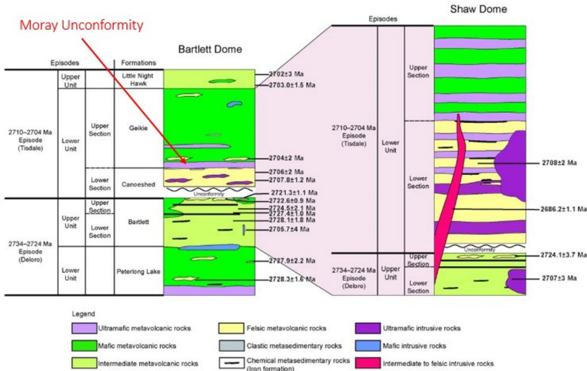
Figure 7.2.2: Comparison of Stratigraphy from the Bartlett and Shaw Domes
