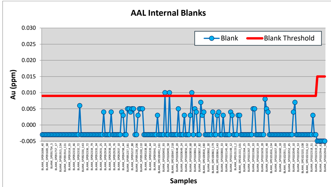
Figure 11.18 AAL Internal performance chart for Au in coarse blank.
