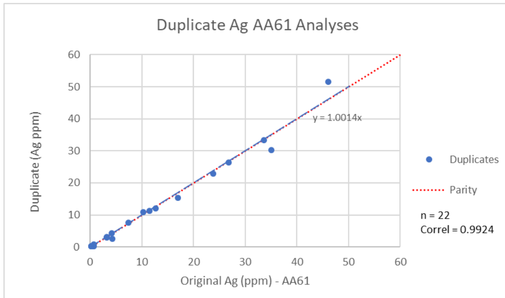
Figure 11.27 2019 duplicate Ag analyses.
