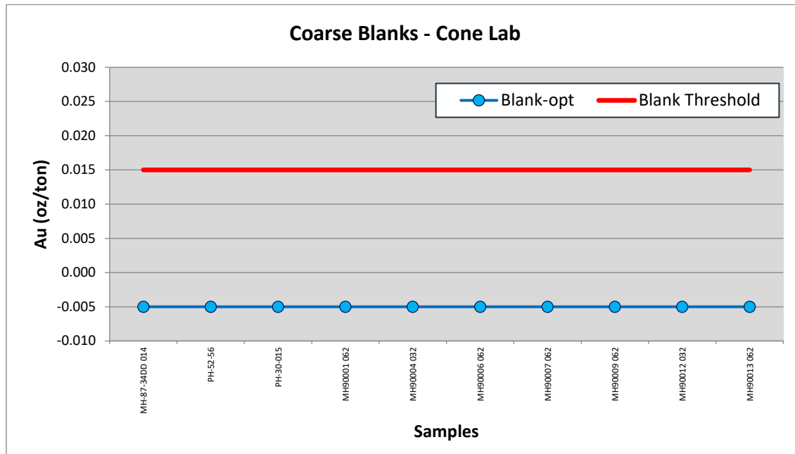
Figure 11.2 Cone performance chart for Au in blank material.
