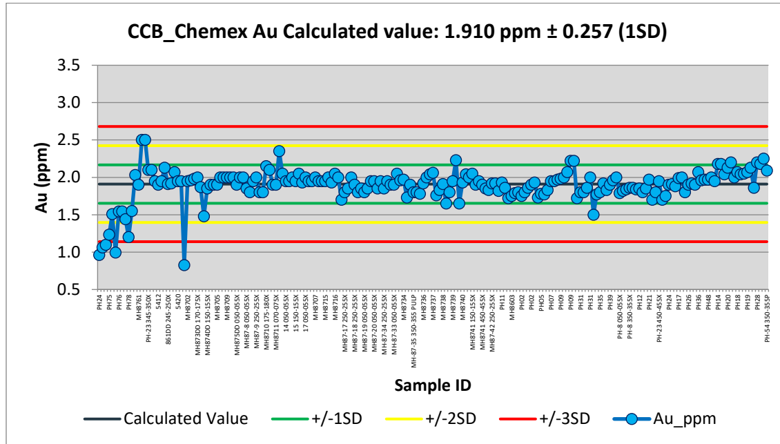
Figure 11.3 Performance chart for Au standard CCB (Chemex).
