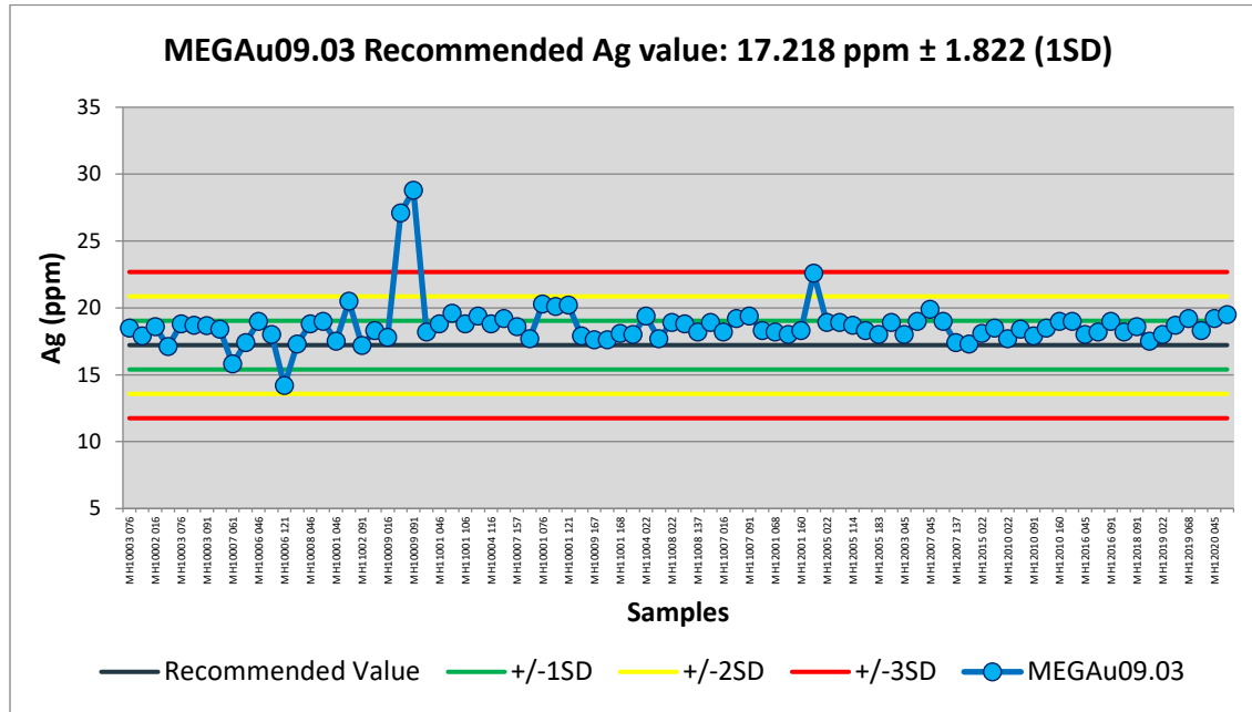
Figure 11.23 Performance chart for Ag standard MEGAu09.03.
