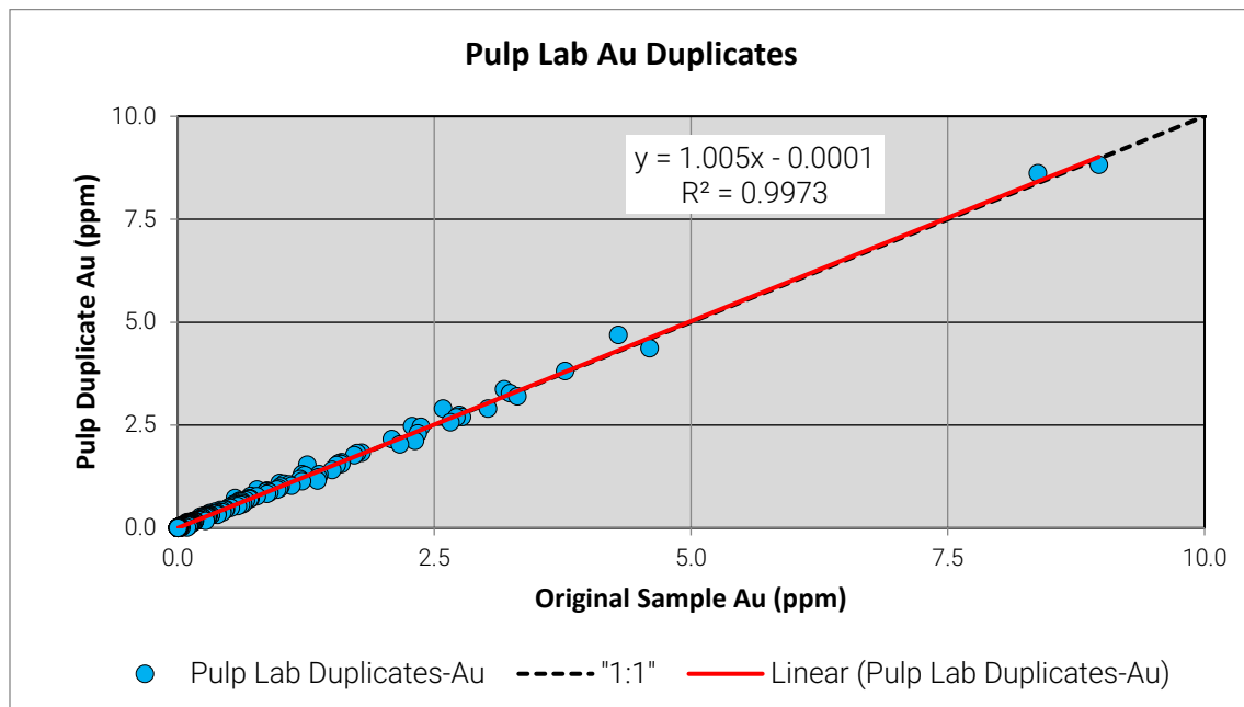
Figure 11.25 Lab pulp duplicate scatter plot Au performance chart.
