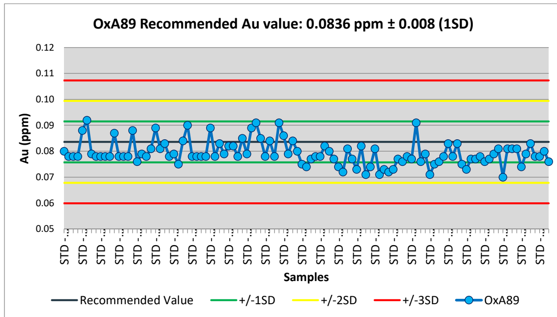
Figure 11.21 Performance chart for AAL Rocklabs Au standard Ox89.
