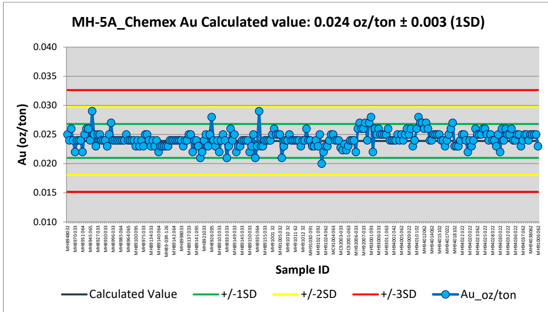
Figure 11.5 Performance chart for Au standard MH-5A (Chemex).
