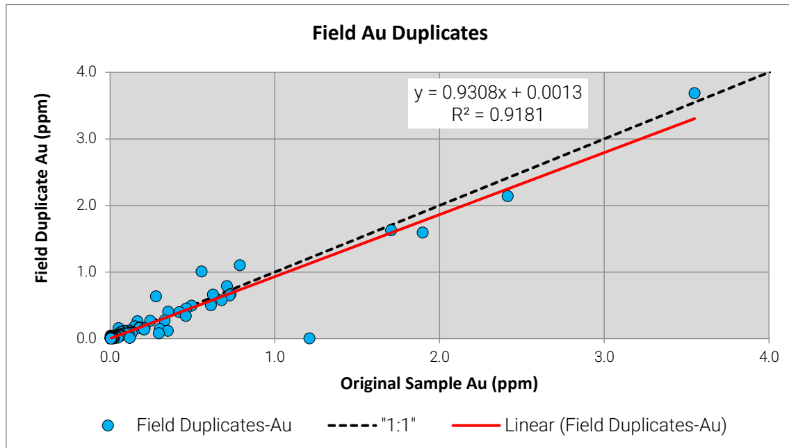
Figure 11.24 Field duplicate scatter plot Au performance chart.
