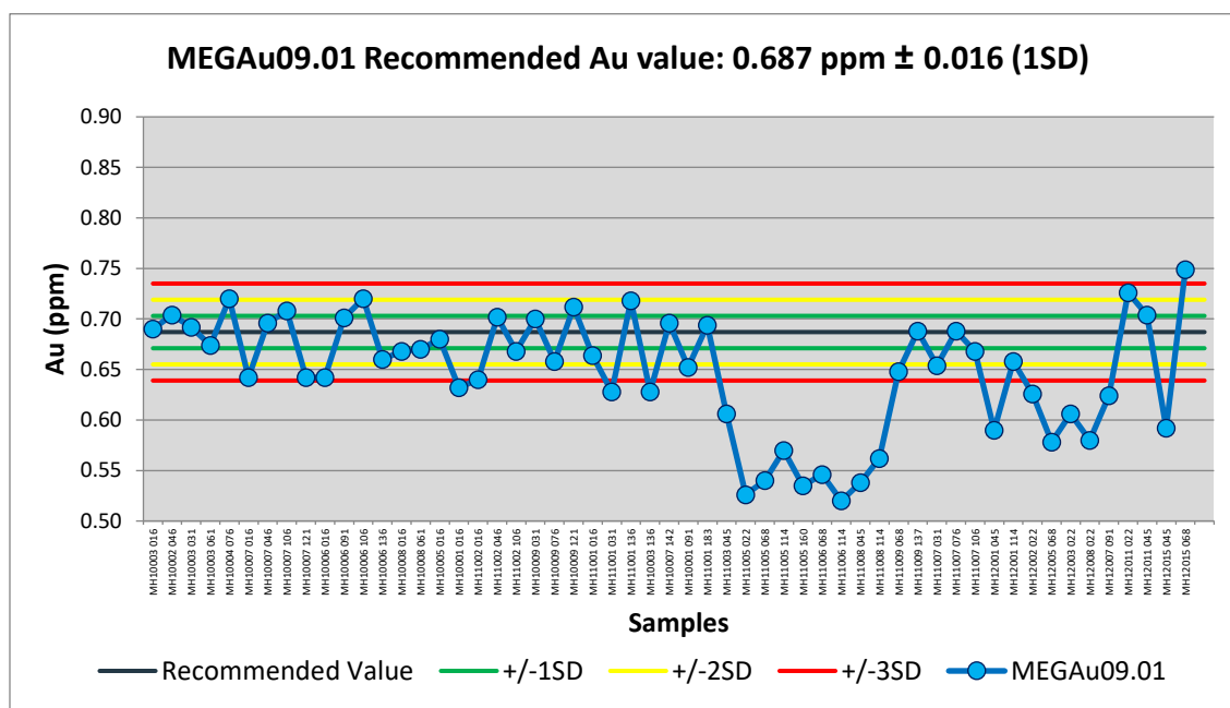
Figure 11.19 Performance chart for Au standard MEGAu09.01.
