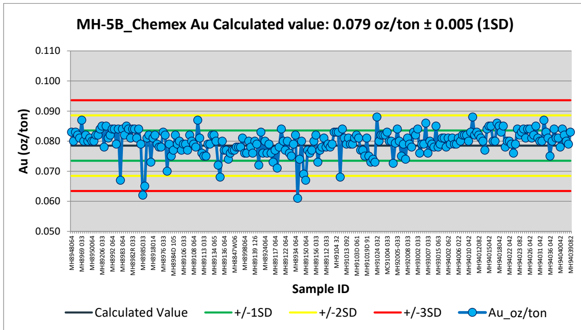
Figure 11.6 Performance chart for Au standard MH-5B (Chemex).
