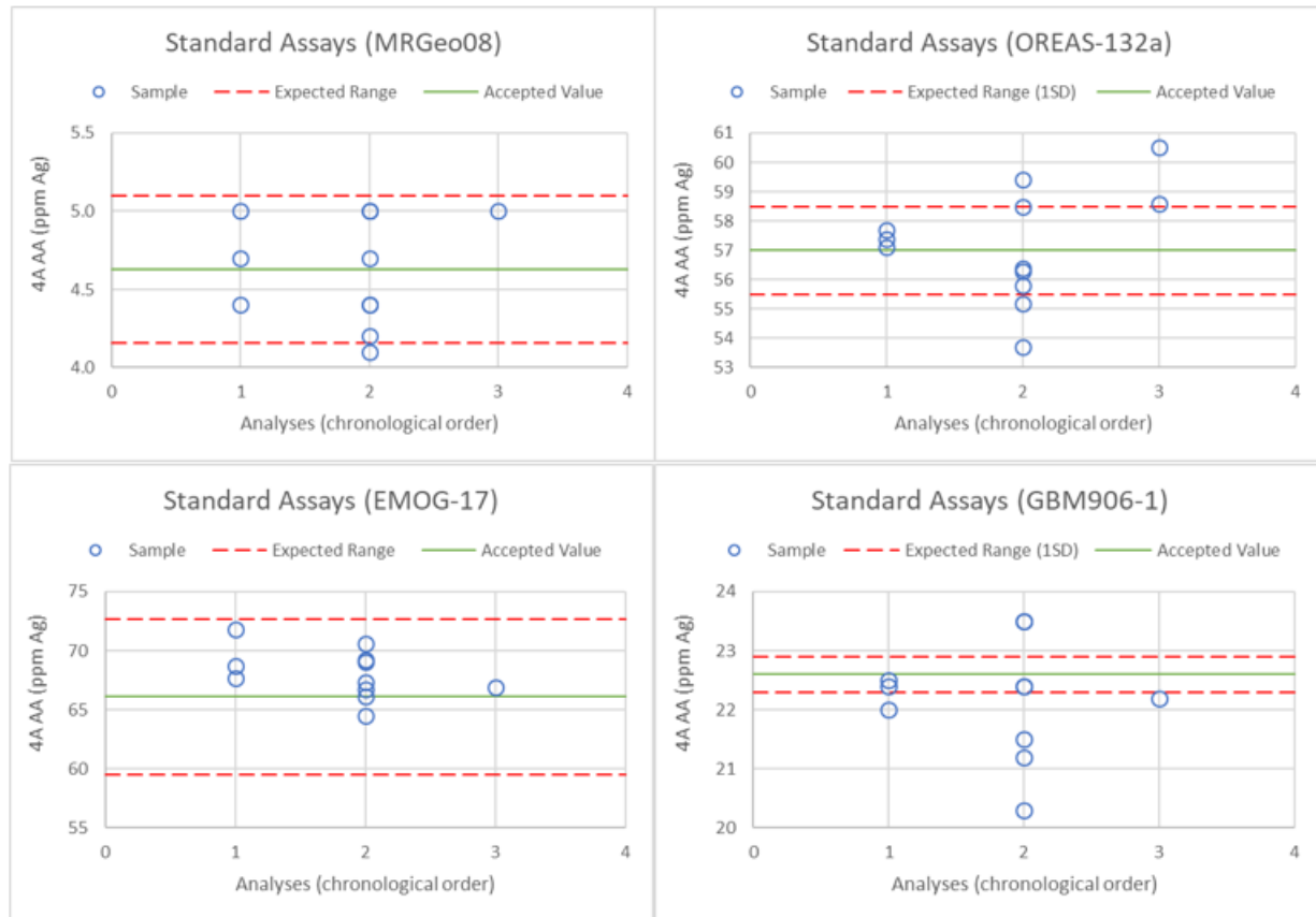
Figure 11.26 Standard reference material analyses for the 2019 Ag analyses.
