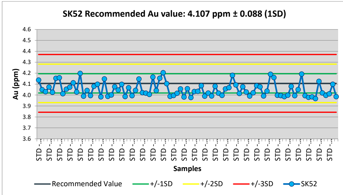
Figure 11.22 Performance chart for AAL Rocklabs Au standard SK52.
