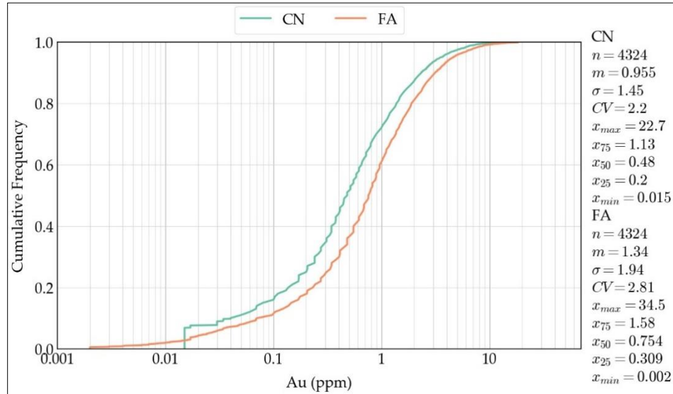
Figure 11.28 Comparison of Au-CN with Au-FA methods.
