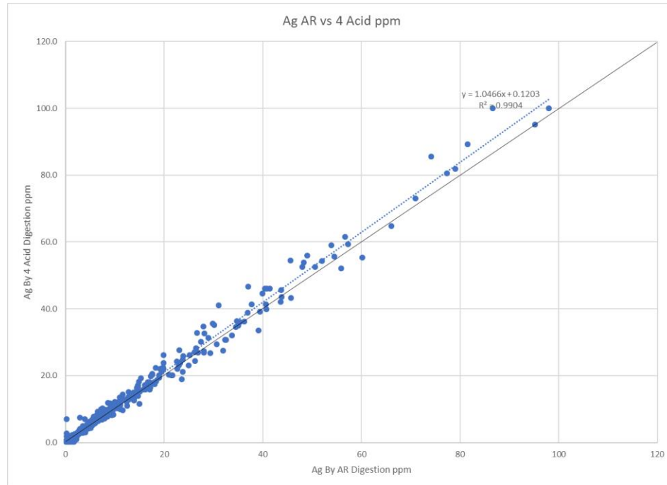
Figure 11.31 Comparison Ag AR to Ag 4 acid analytical technique.
