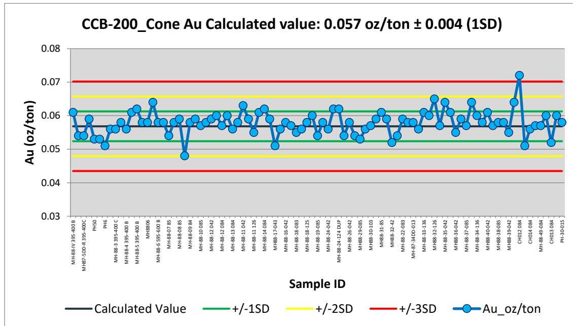
Figure 11.4 Performance chart for Au standard CCB-200 (Cone).
