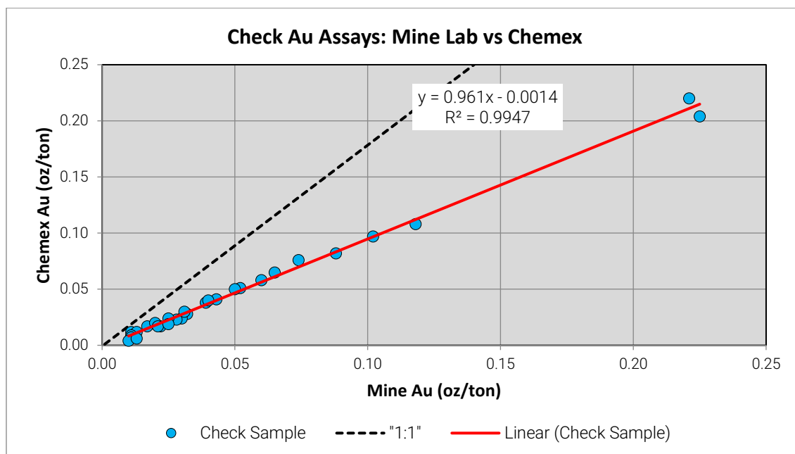
Figure 11.16 Scatter plot of mine lab vs Chemex check Au assays.
