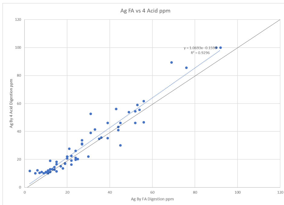
Figure 11.33 Comparison Ag FA to Ag 4 acid technique.
