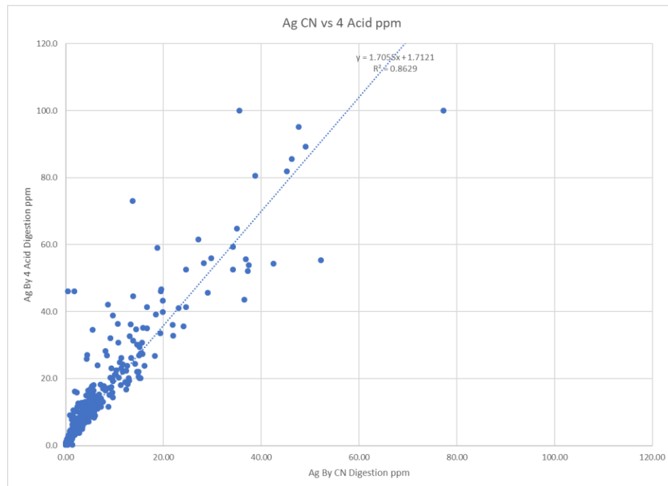
Figure 11.32 Comparison Ag CN to Ag 4 acid technique.
