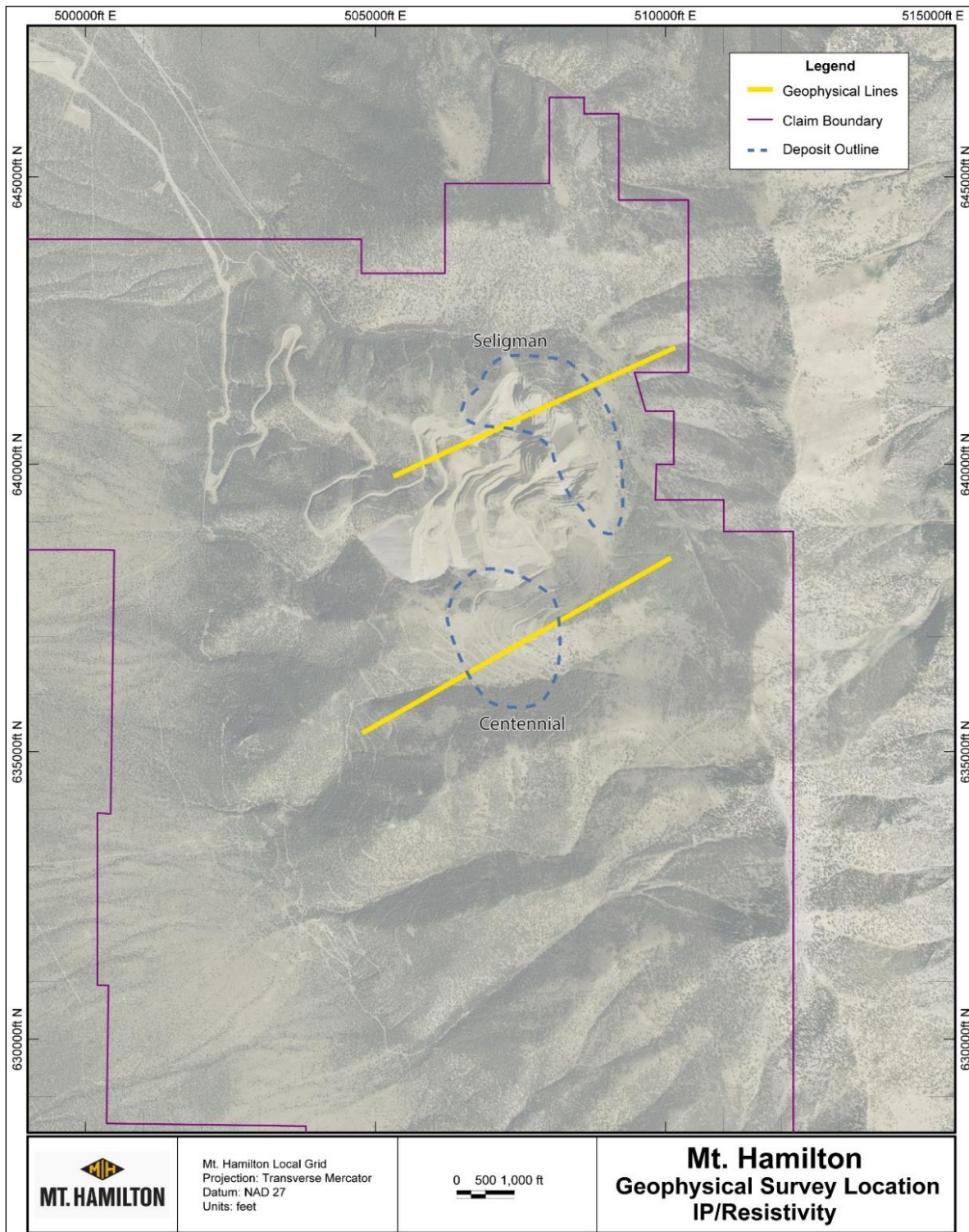
Figure 6.1 Location of 2004 geophysical IP/resistivity survey.
