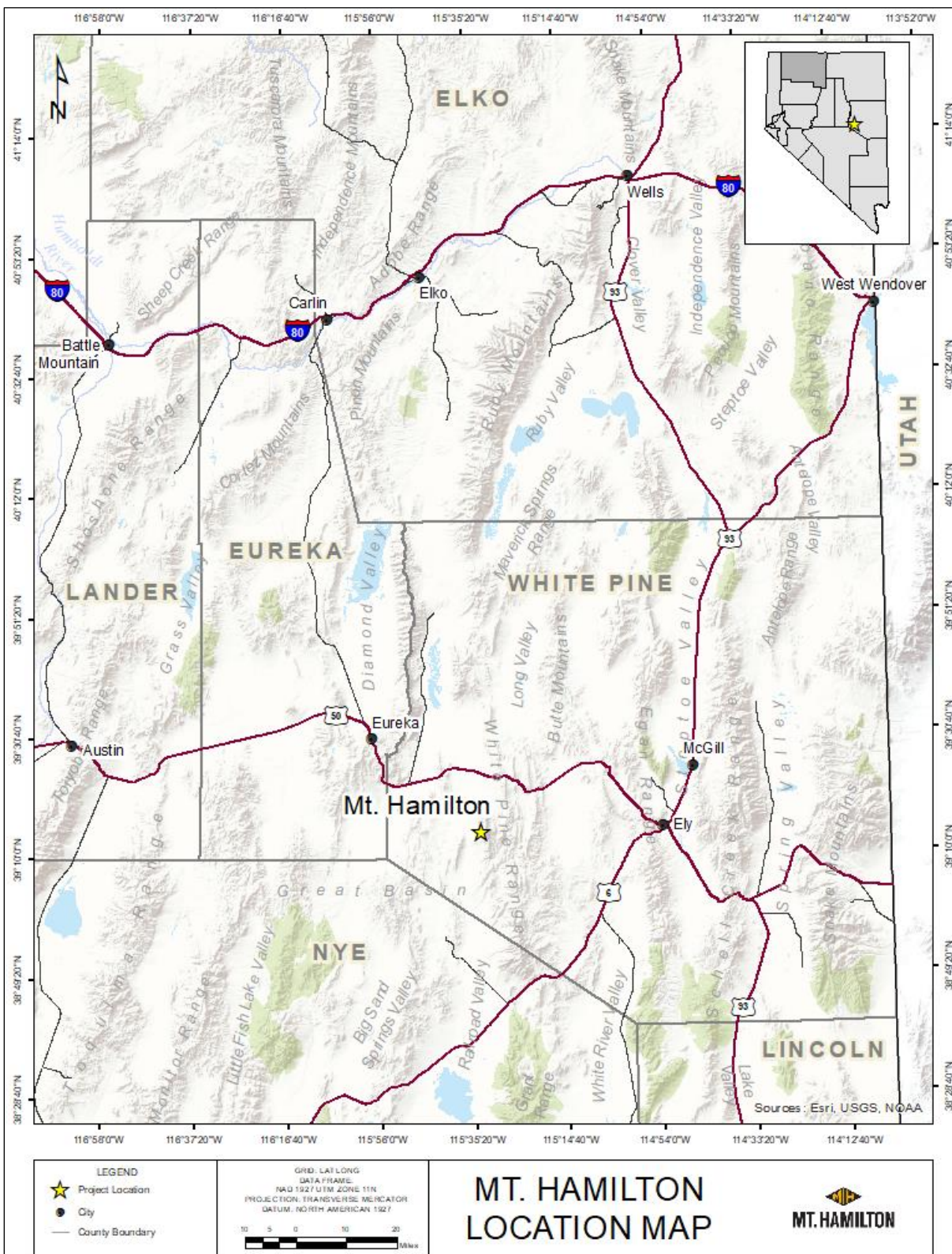
Figure 2.1 Mt. Hamilton Property location.
