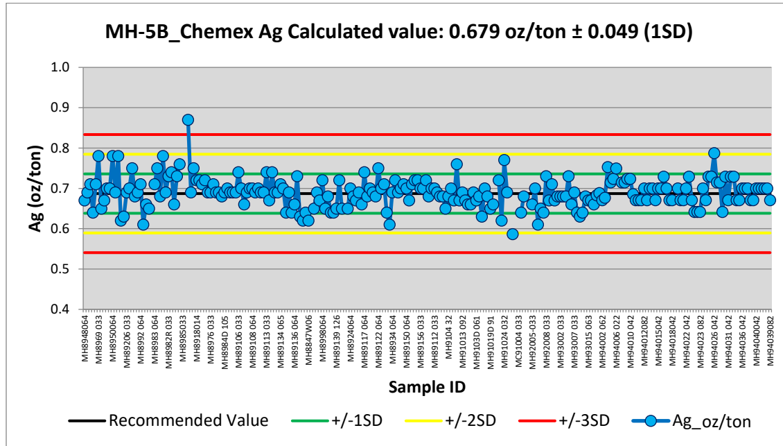
Figure 11.8 Performance chart for Ag standard MH-5B (Chemex).
