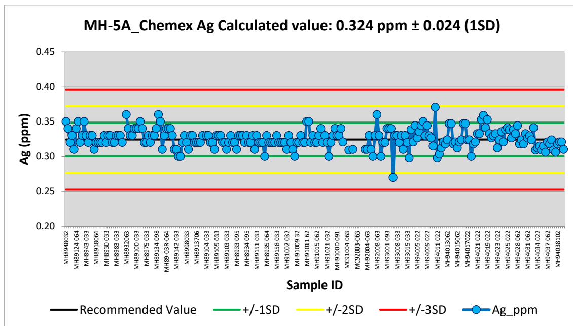
Figure 11.7 Performance chart for Ag standard MH-5A (Chemex).
