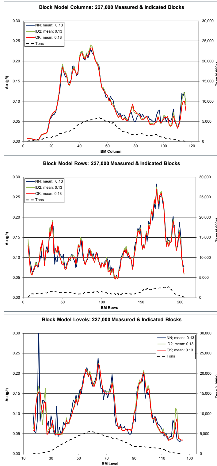
Figure 14.7 Swath plots through the gold resource model.
