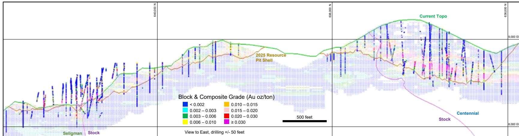
Figure 14.6 Section 507,400E - gold block model and composites data.
