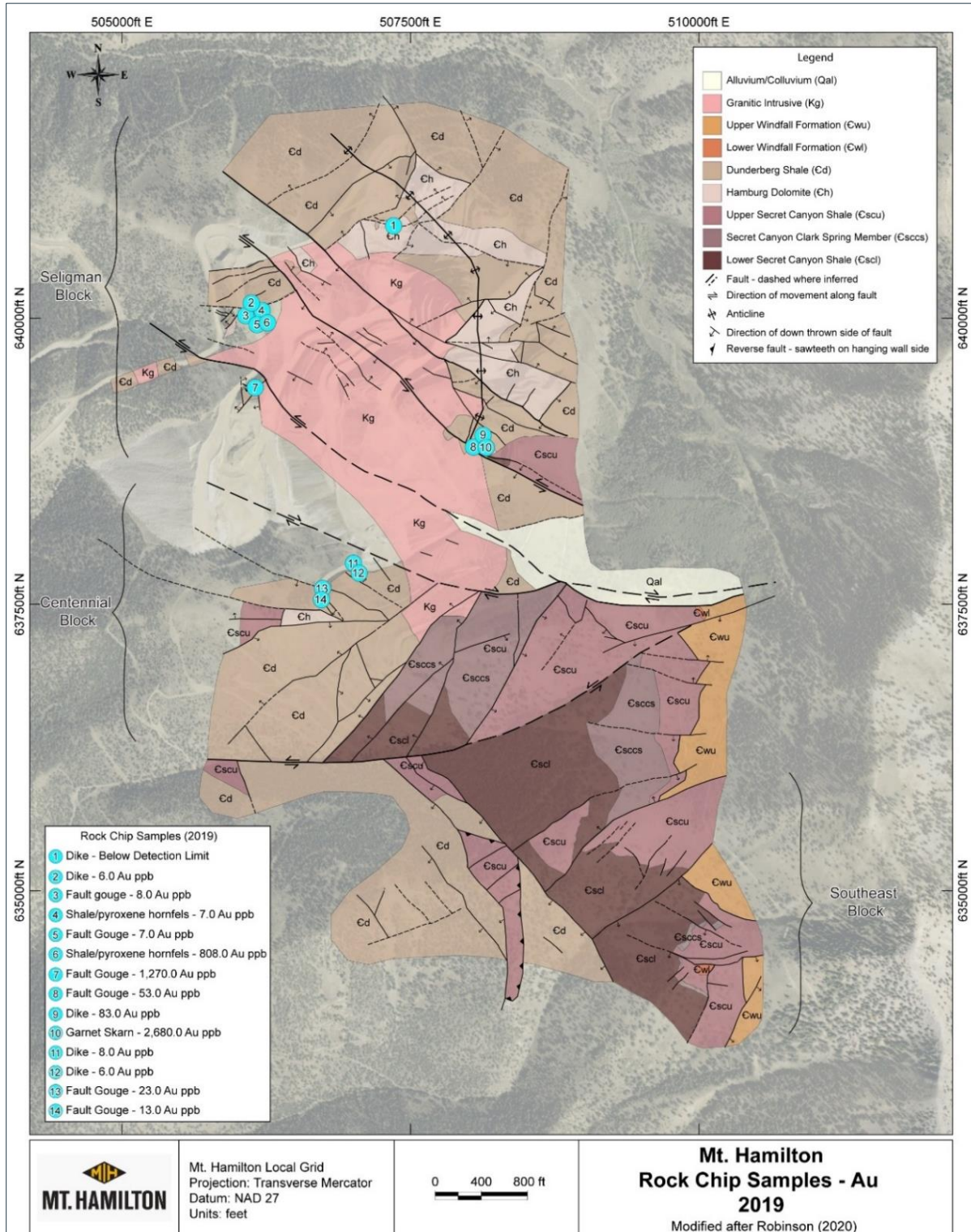
Figure 9.1 Location and results of 2019 Au rock chip sampling.
