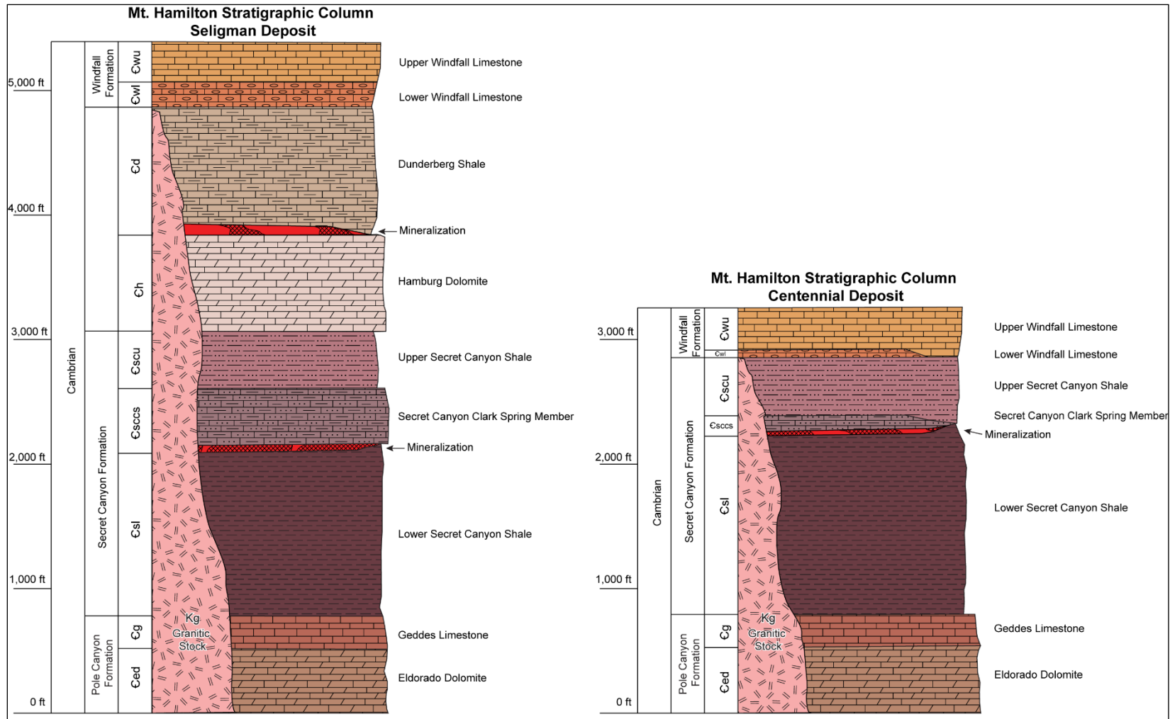
Figure 7.3 Mt. Hamilton stratigraphy relative to the Seligman and Centennial deposits.
