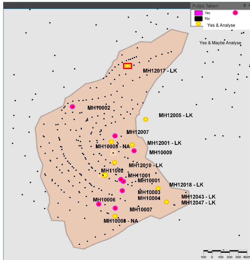
Figure 11.30 Drillhole location and pulp selection.
