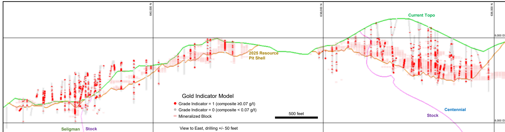
Figure 14.4 Section 507,400E - Indicator Modelled mineralized zones.
