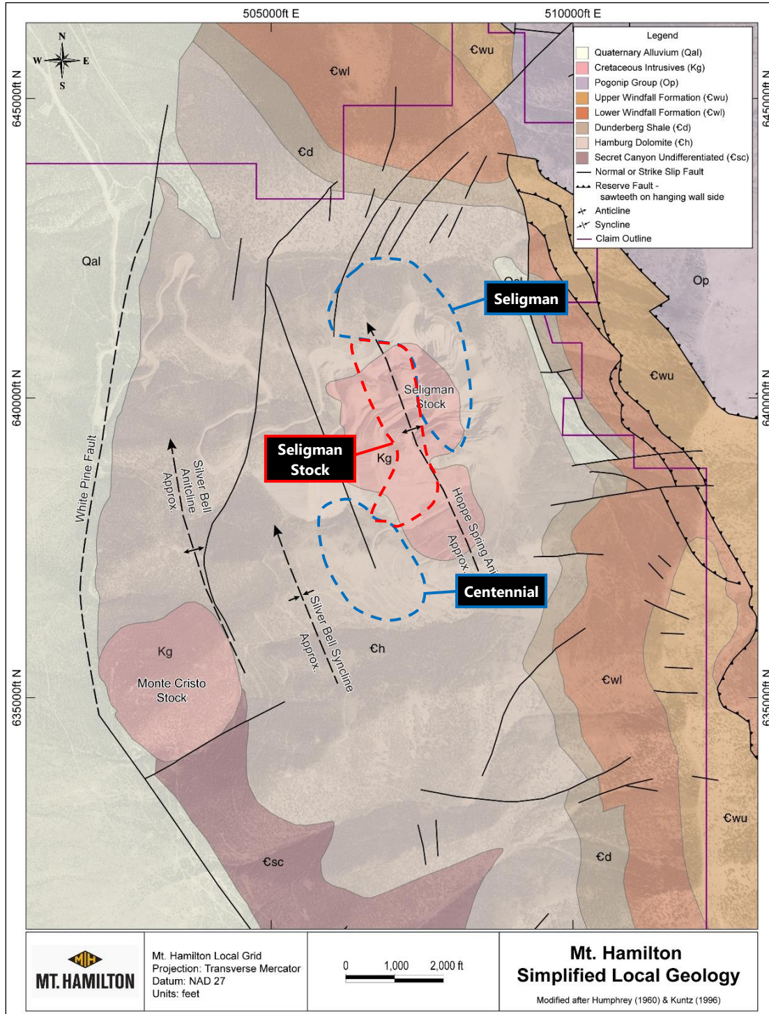
Figure 7.2 Mt. Hamilton Property geologic map with deposit outlines.
