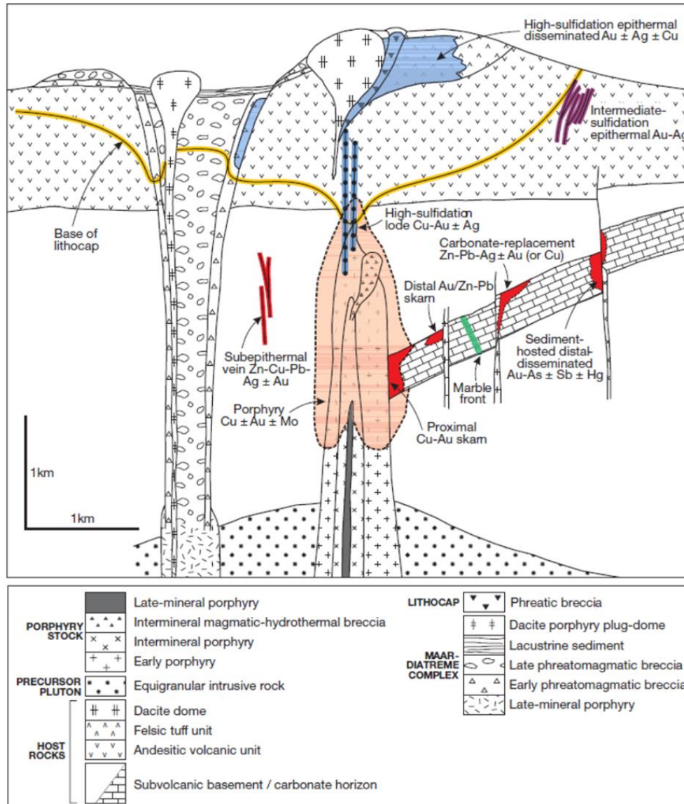
Figure 8.2 Conceptual model of the porphyry and epithermal systems.
