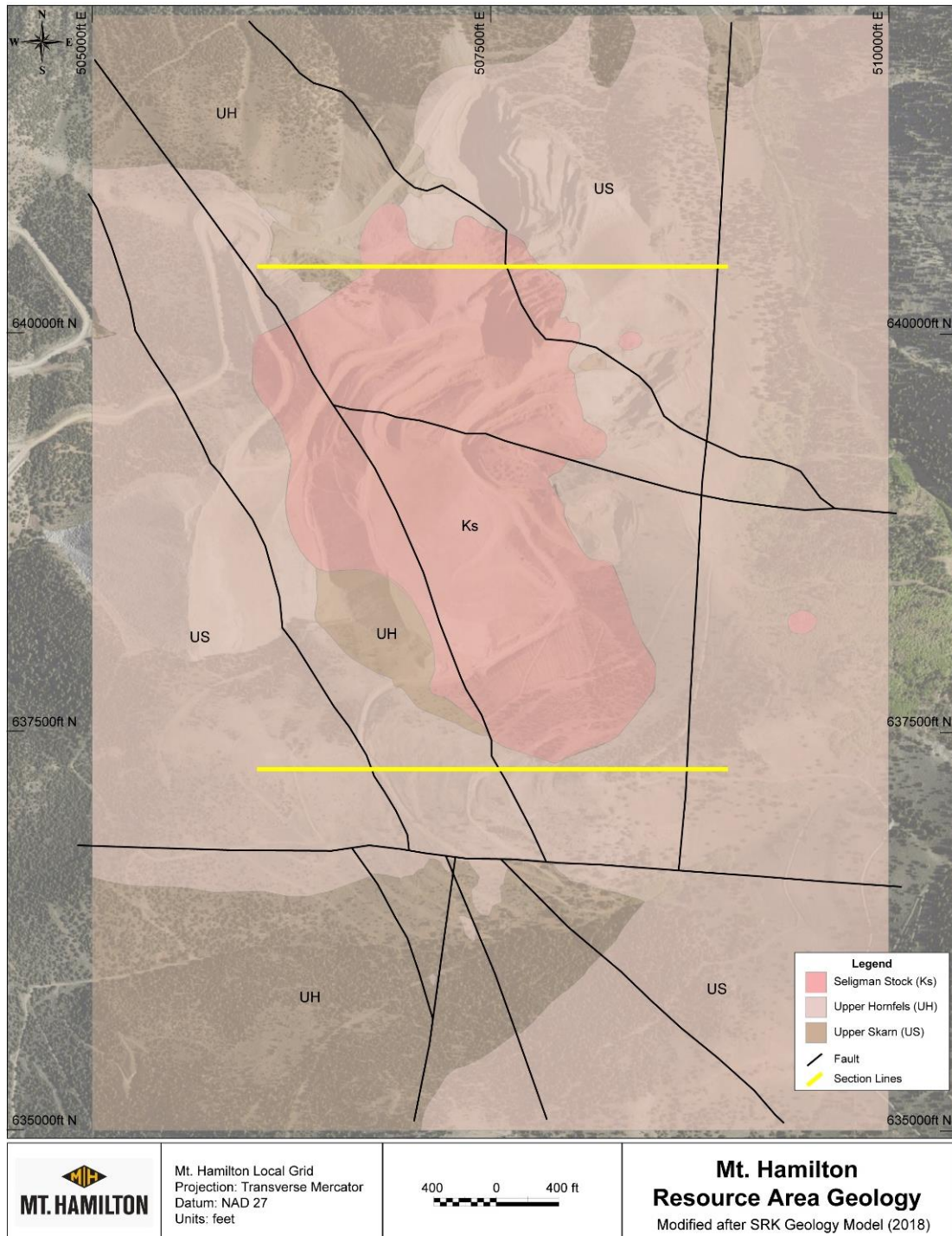
Figure 7.4 Resource area geology with structural blocks separating the Seligman deposit to the north and the Centennial deposit to the south.
