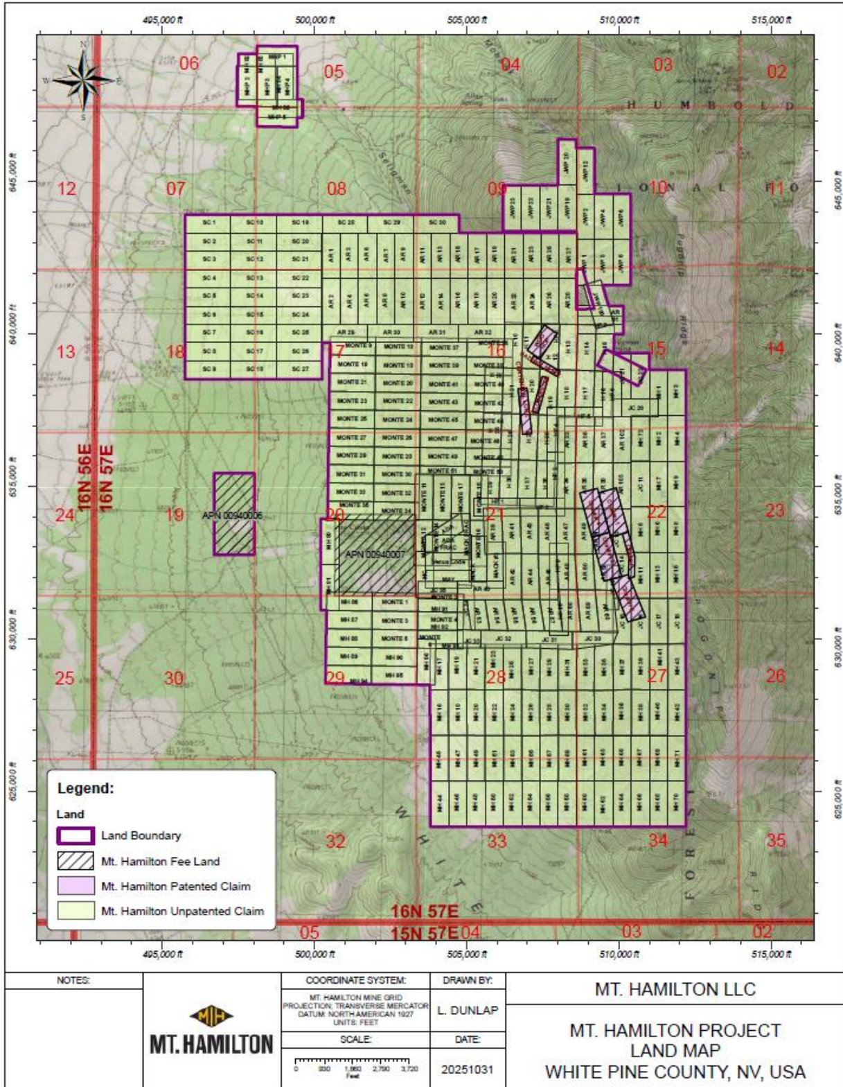
Figure 4.1 Mt. Hamilton Property mineral tenure.
