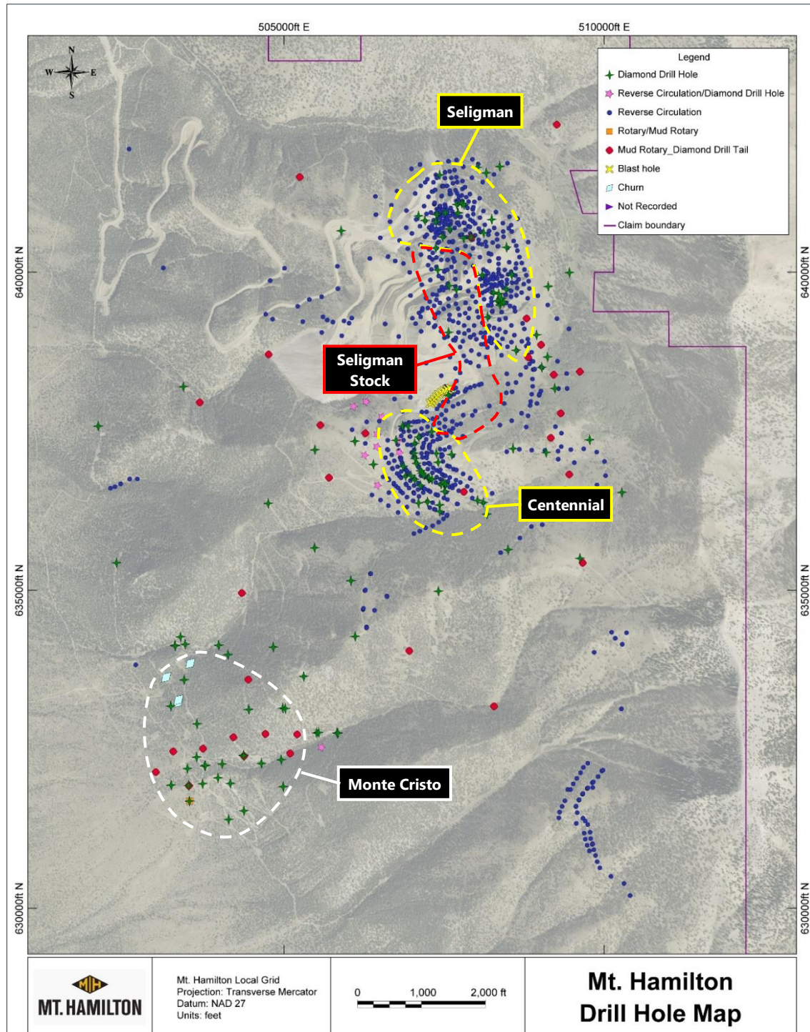
Figure 10.1 Drillholes located within the Mt. Hamilton Property boundary.
