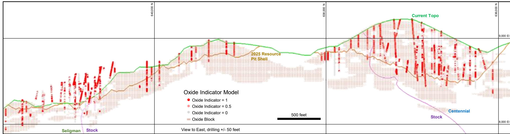
Figure 14.2 Section 507,400E – oxide block model by indicator estimation.
