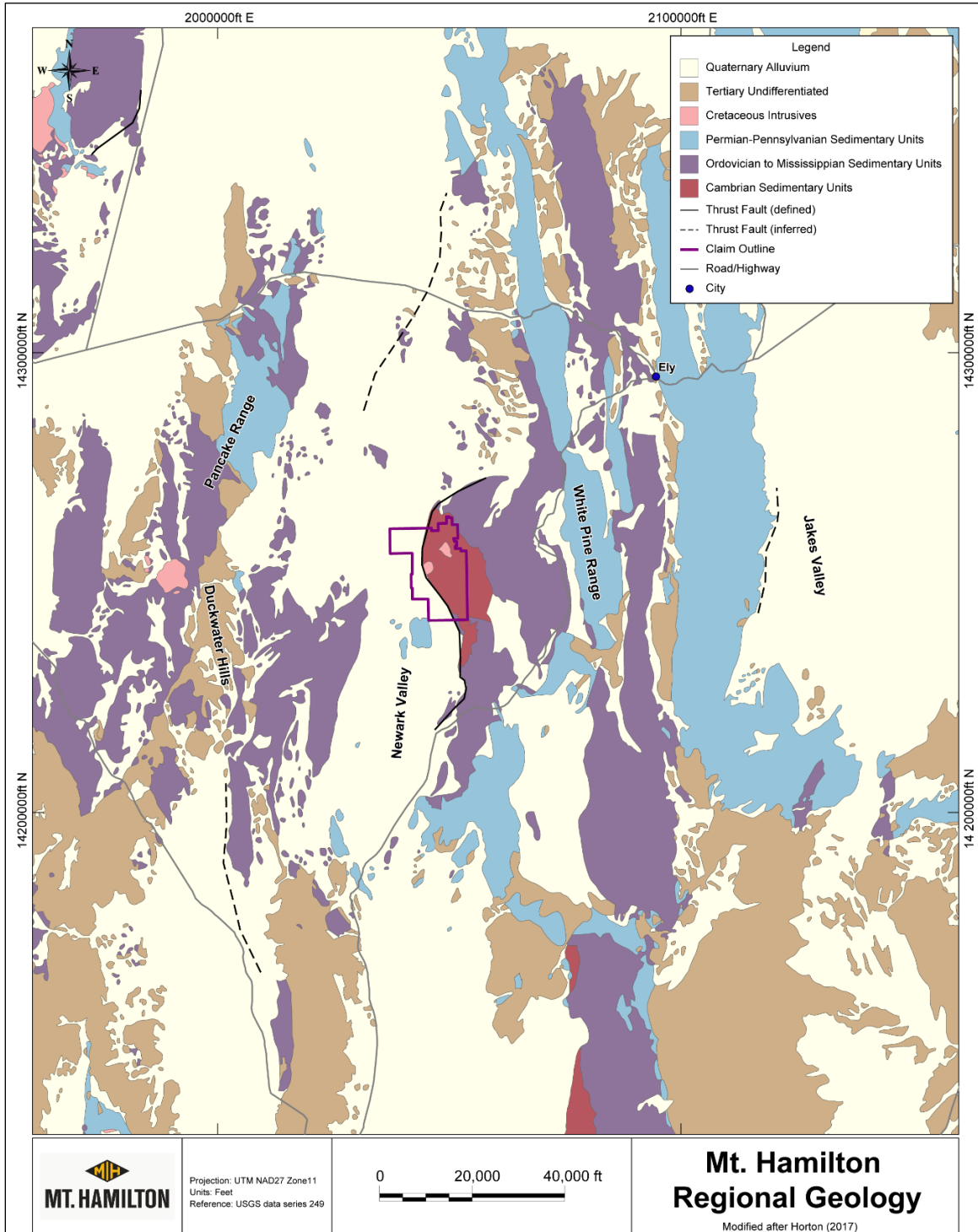
Figure 7.1 Regional geology map of the Property area.
