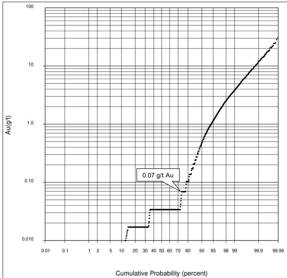
Figure 14.3 Log Probability Plot – all gold assays.
