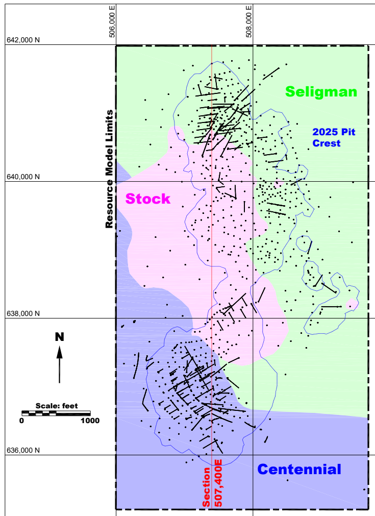
Figure 14.1 Block model limits and drill plan.
