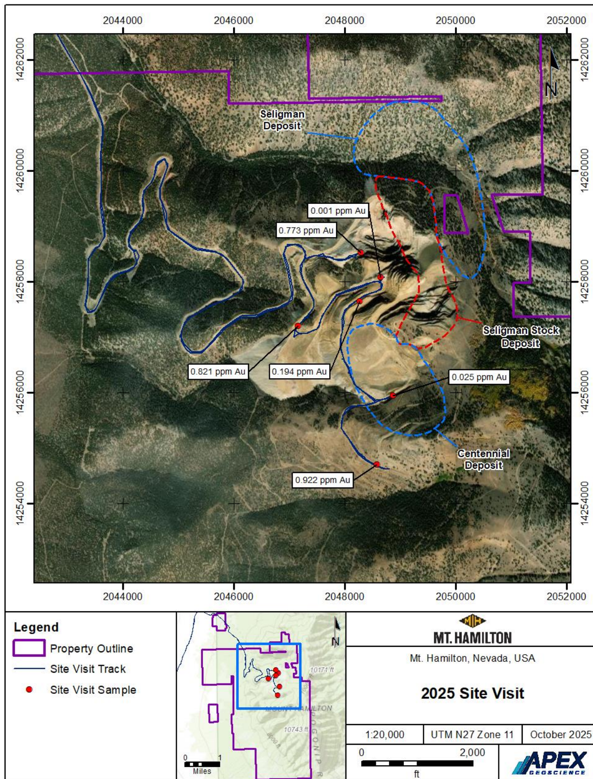
Figure 12.1 Traverse and samples collected during the author's 2025 site visit.
