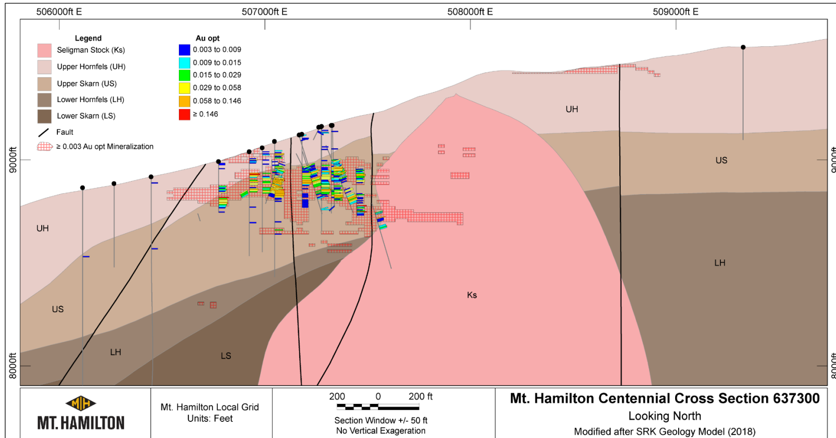
Figure 7.6 Cross section of the Centennial deposit with drillholes, mineralization, redox, and Au grade.
