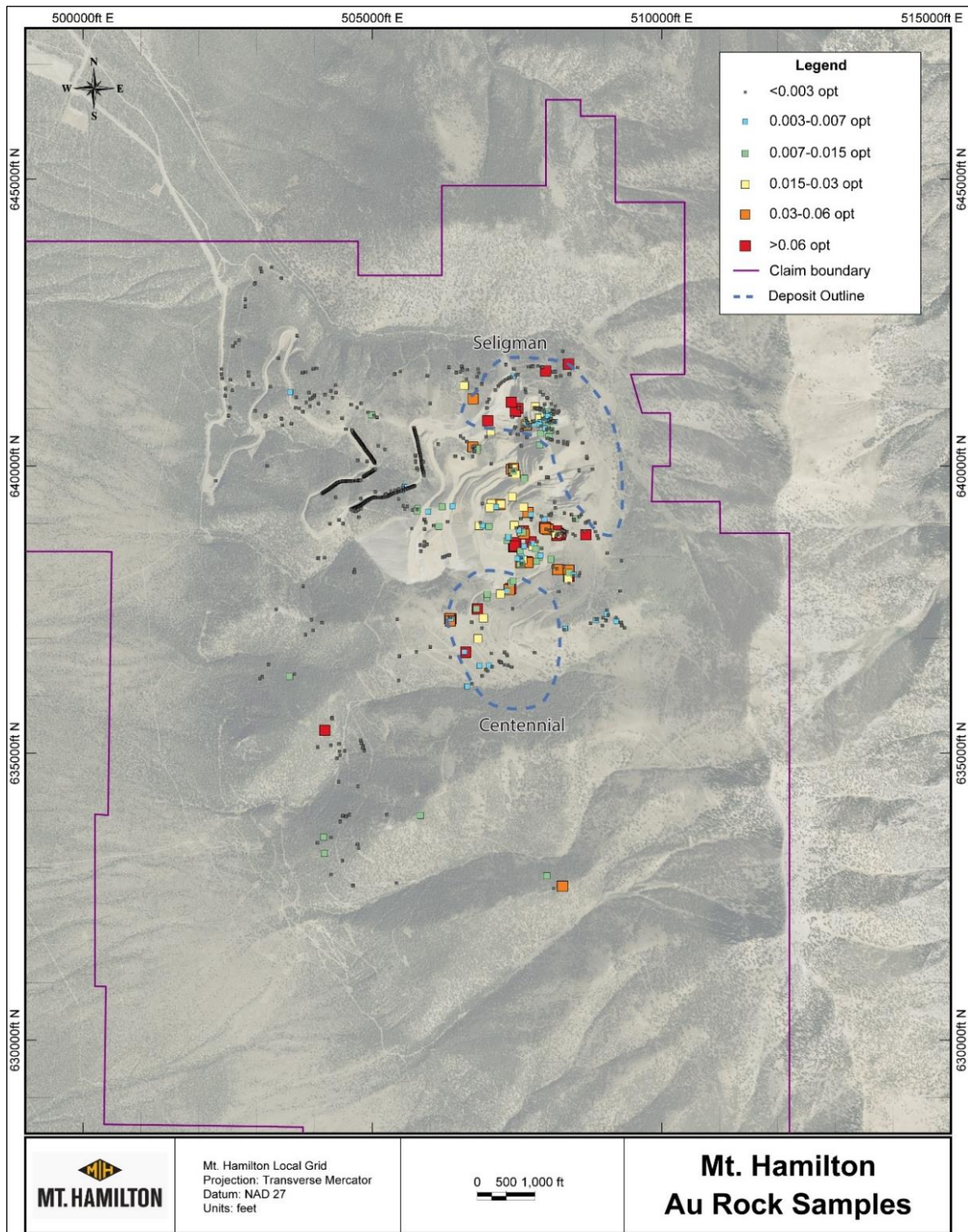
Figure 6.3 Rock samples with Au grades.
