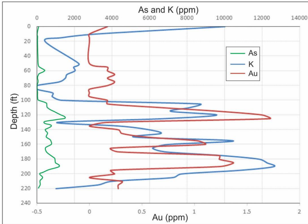
Figure 10.2 Hole 95172 Au assay data and pXRF potassic (K) and arsenic (As) chemistry.
