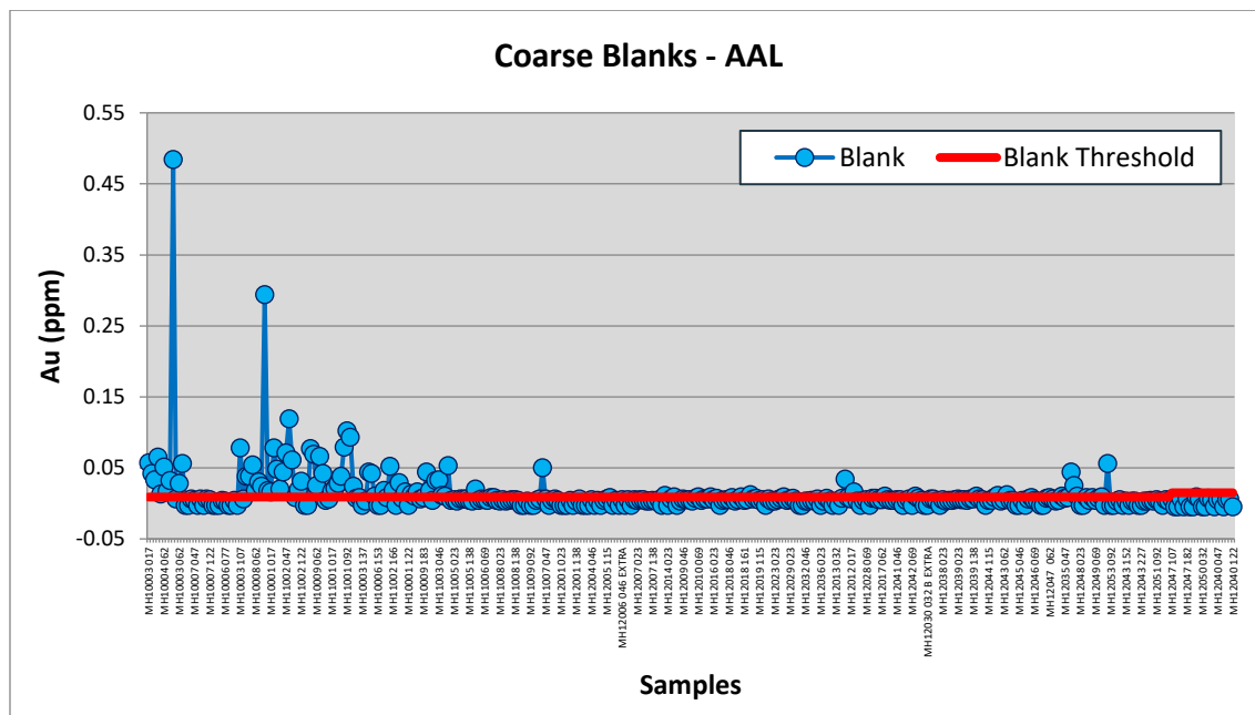
Figure 11.17 AAL Performance chart for Au in coarse blank.
