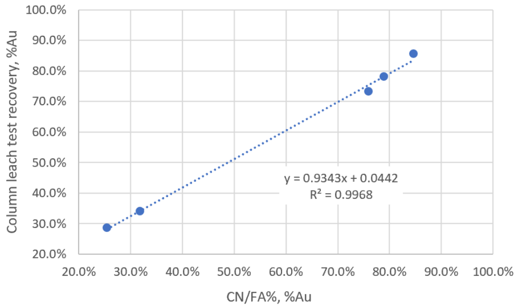
Figure 13.1 Au CN/FA% vs column leach Au recovery %.
