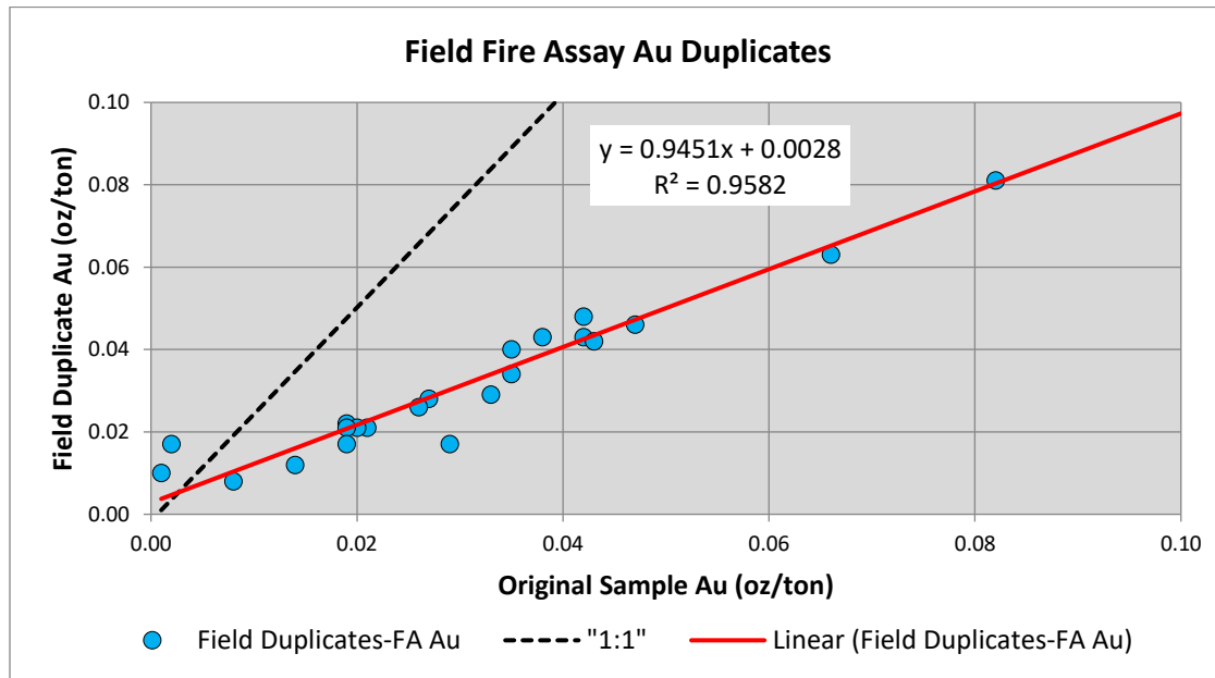
Figure 11.15 Field duplicate scatter plot FA Au performance.
