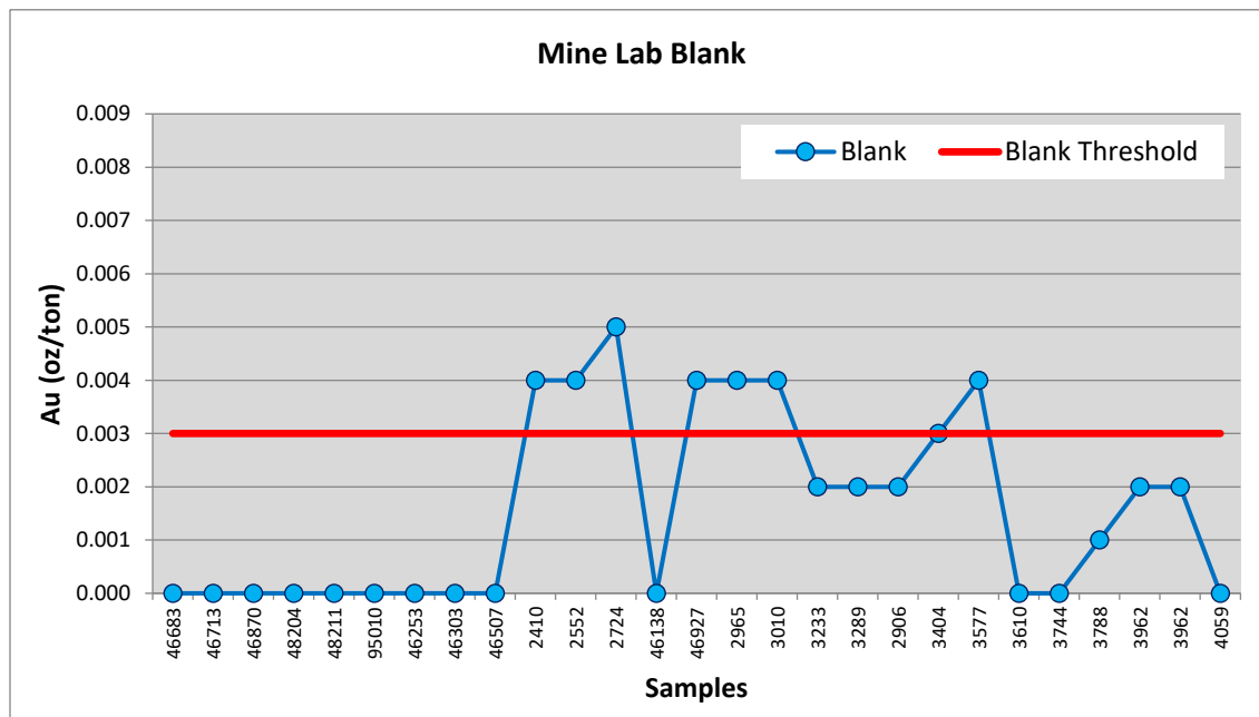
Figure 11.11 Mine site performance chart for Au in coarse blank.
