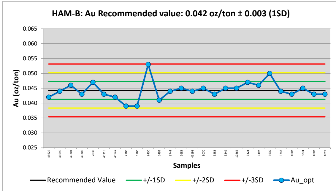
Figure 11.12 Performance chart for Au standard HAM-B.
