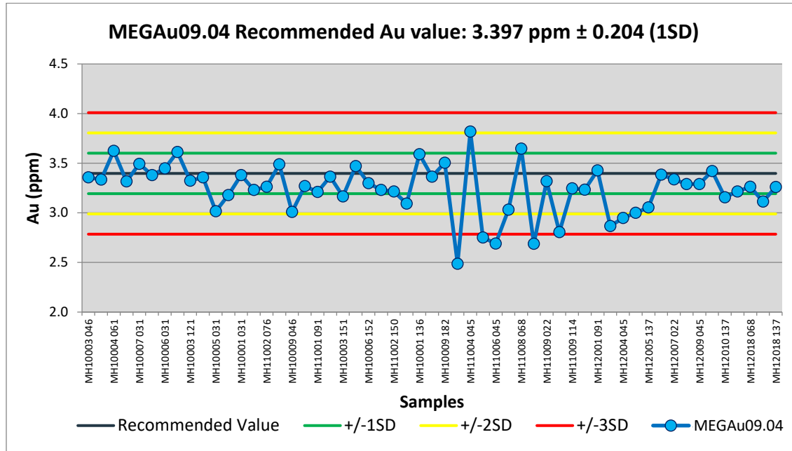
Figure 11.20 Performance chart for Au standard MEGAu09.04.
