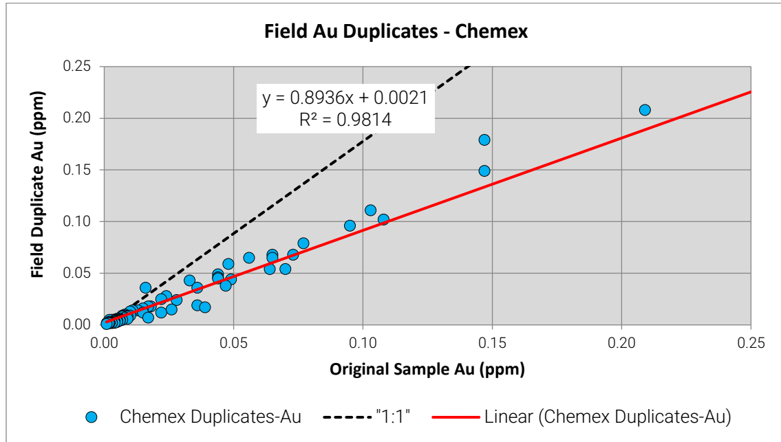
Figure 11.9 Field duplicate scatter plot Au performance (Chemex).
