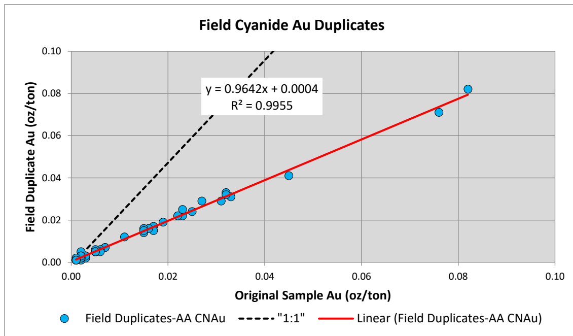
Figure 11.14 Field duplicate scatter plot cyanide Au performance.
