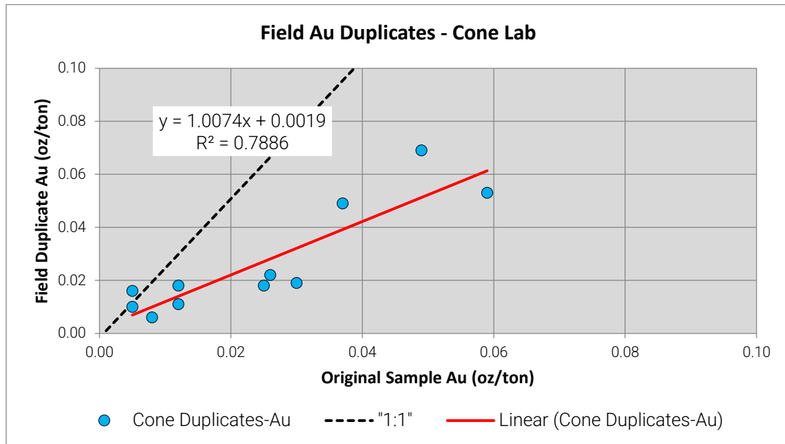
Figure 11.10 Field duplicate scatter plot Au performance (Cone).
