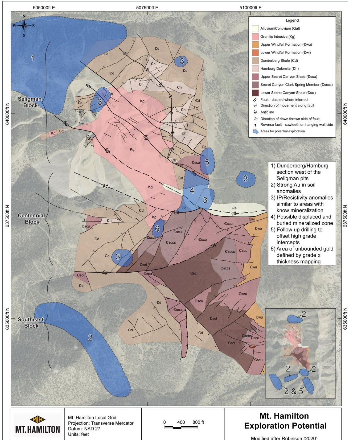
Figure 9.2 Geologic map showing potential Au-Ag exploration target areas.
