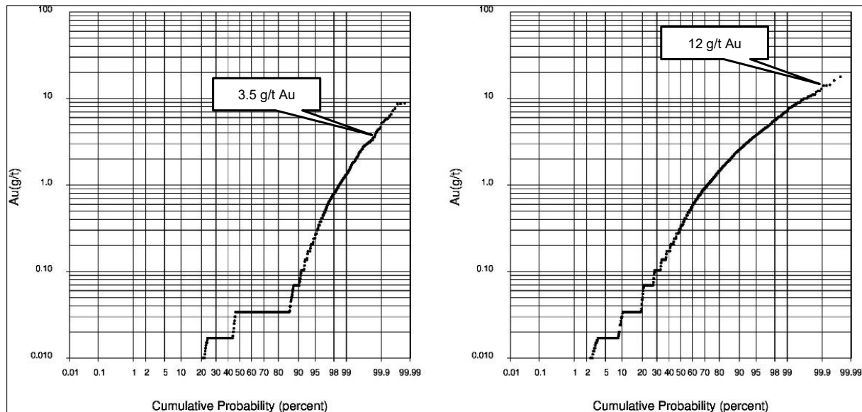
Figure 14.5 Centennial assay probability plots (background – left, mineralized – right).
