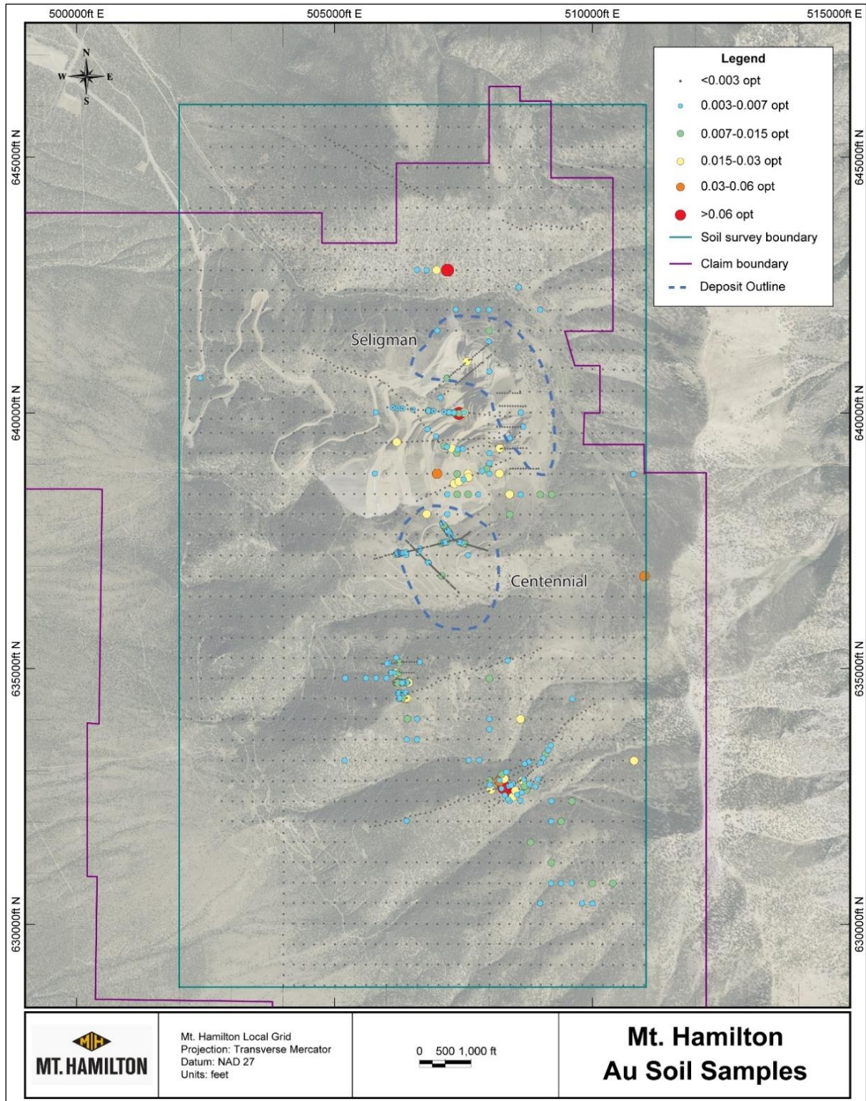
Figure 6.2 Soil sample survey with Au grades.
