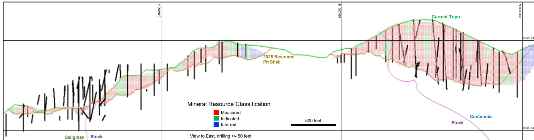
Figure 14.8 Section 507,400E – classified mineral resource blocks.
