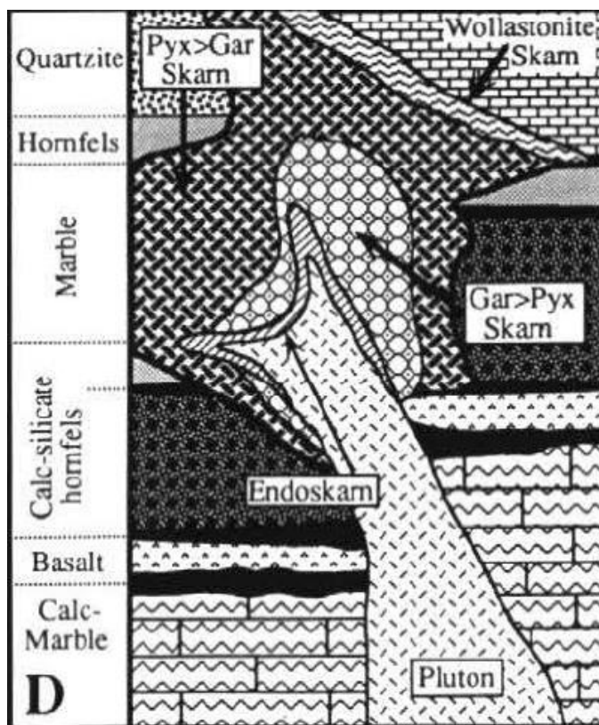
Figure 8.1 Generalized cross-section of a skarn deposit and alteration halo
