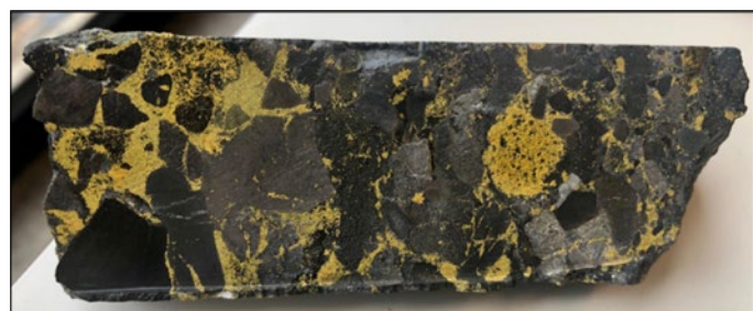
Matrix-filling and disseminated blebs and clots of orpiment (yellow mineral) in silicified, brecciated limestone conglomerate (Hole P22-02; 46.74m to 46.86m)
