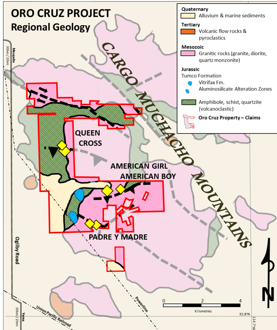
Regional Geology of the Cargo Muchacho Mountains
