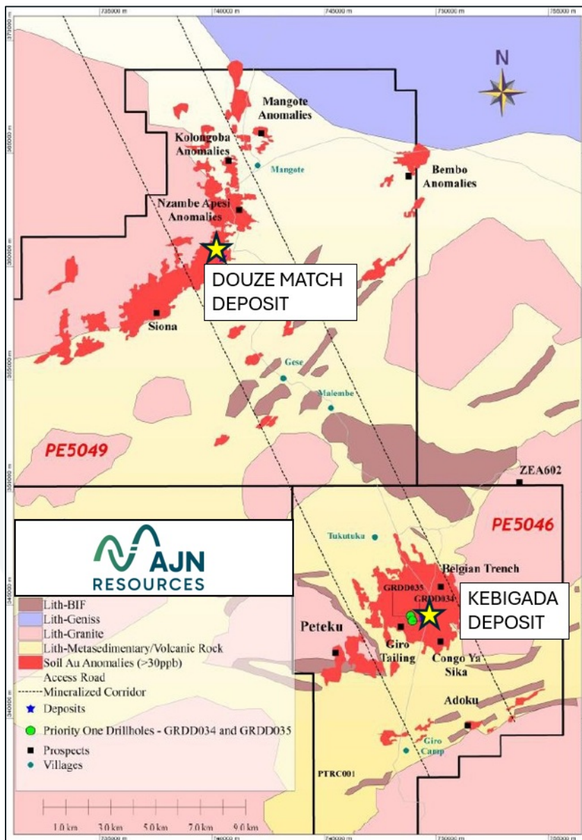
Figure 2: Map 2 showing the geology and >30ppb gold-in-soil anomalies (red) at the Giro Gold Project.
