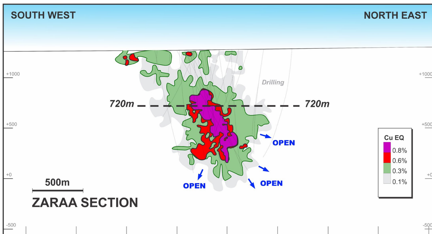
Figure 8: Long section of the Zараа Deposit, displaying the Mineral Resource Estimate extents in relation to drilling.
