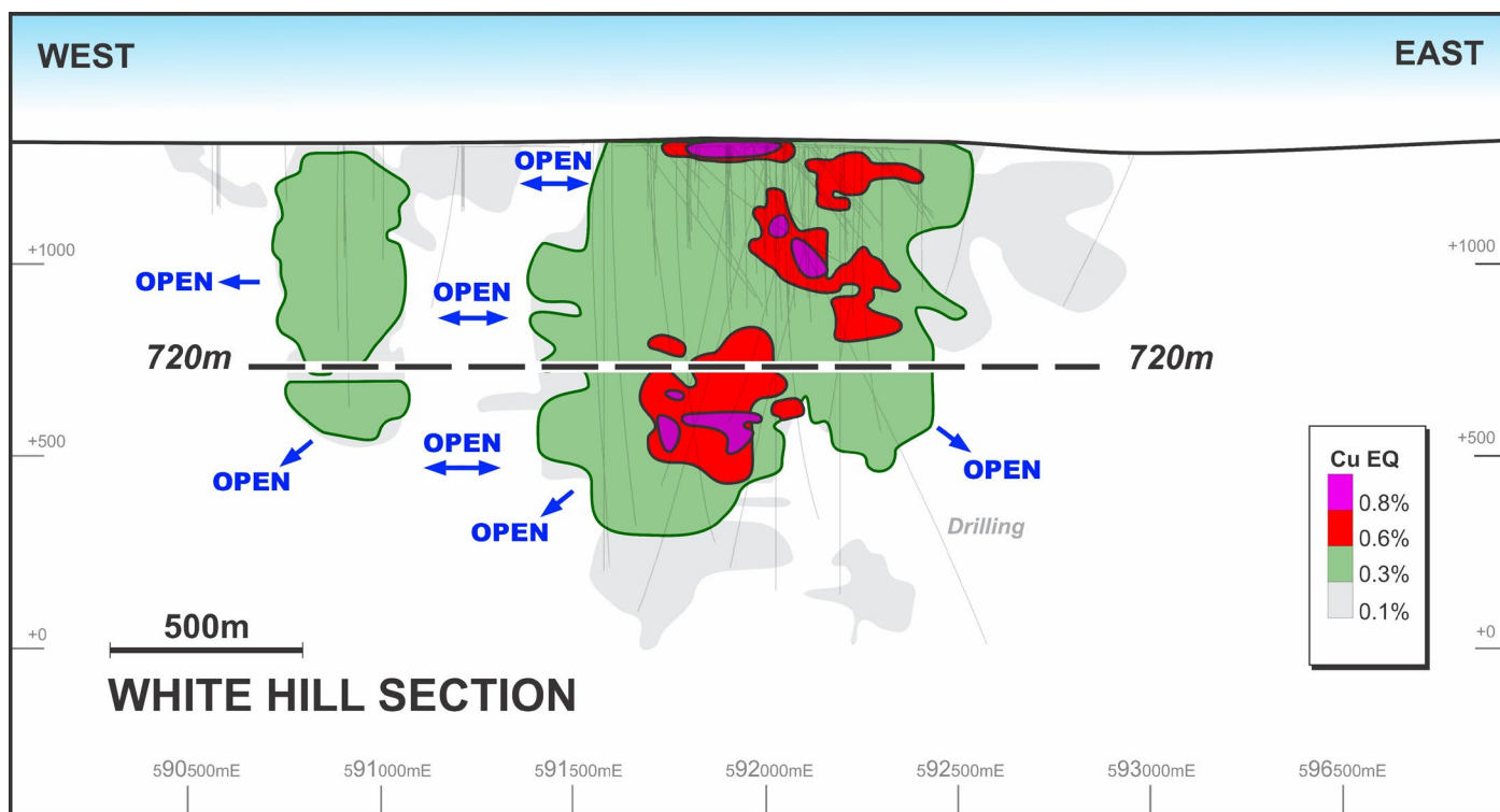
Figure 7: Long section of the White Hill Deposit, displaying the Mineral Resource Estimate extents in relation to drilling.
