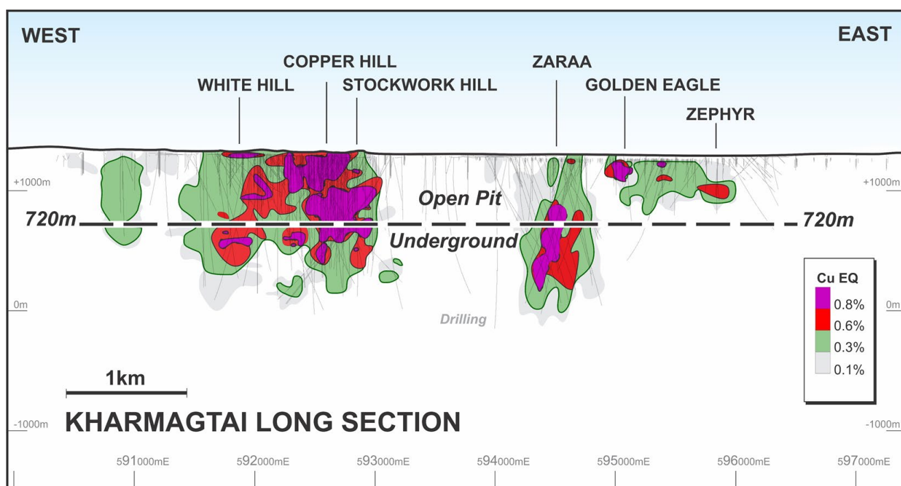
Figure 2: Long-section of the Kharmagtai district, displaying the Mineral Resource Estimate extents in relation to drilling, showing notional 720mRL split between potential open pit and underground.
