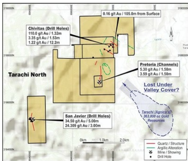
Figure 1: Tarachi North Area. San Javier – Mineralization host in sheared, brecciated and altered volcanics and mineralization open along strike and to depth. (CNW Group/Tarachi Gold Corp.)
