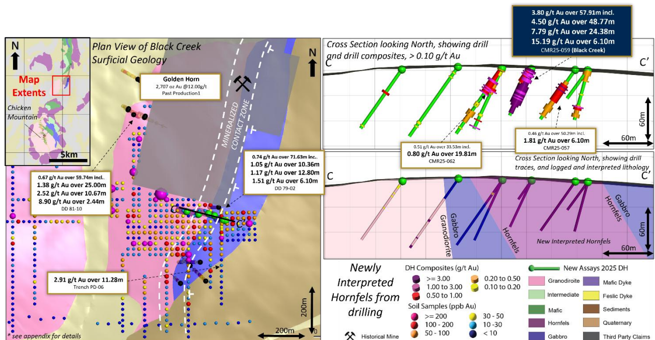
Figure 2: Cross Section Looking North of Black Creek Drilling Line, highlighting drill results and higher-grade corridors can be viewed at: CLICK HERE TO VIEW FIGURE 2
