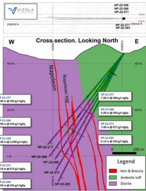
Figure 4: Napoleon cross section with significant intercepts below inferred resources at Ojo de Agua (CNW Group/Vizsla Silver Corp.)
