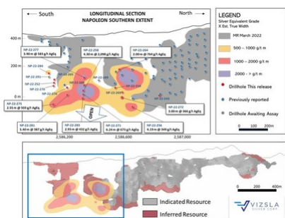
Figure 2: Longitudinal section of the main Napoleon Vein. The section is inclined along the dip of the structure (CNW Group/Vizsla Silver Corp.)
