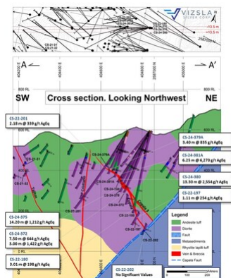
Figure 3: Cross section showing Copala structure, Cristiano, Copala 3, and Tajitos veins with completed drilling. (CNW Group/Vizsla Silver Corp.)
