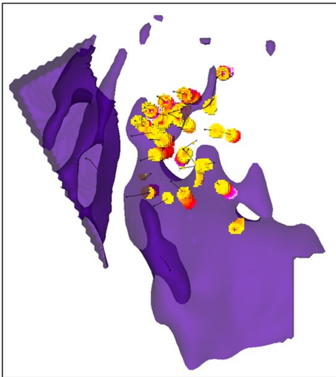
Figure 8 - 3D screenshot displaying phyllic alteration intensity on drill hole traces (yellow to pink representing increasing intensity) and <120 ohm-m resistivity as a purple isosurface.
