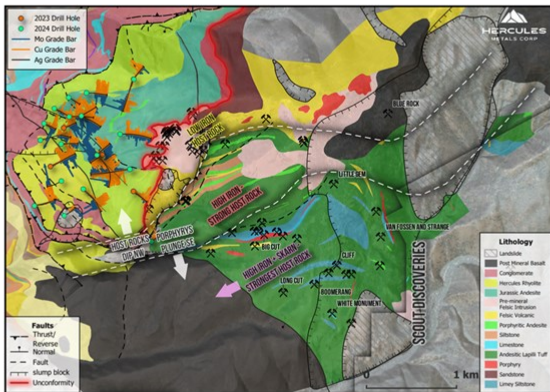
Figure 3 - 2024 Lithology and Structure Map. White dashed lines represent boundaries of varying host rock prospectivity.
