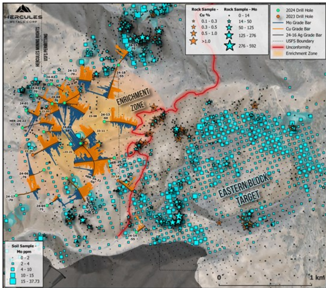
Figure 2: Molybdenum in soil and rock chip samples.
