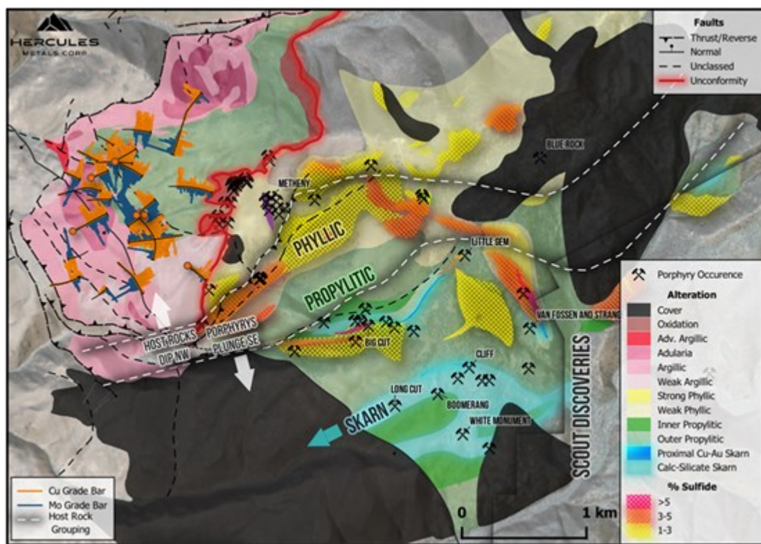
Figure 4 - Alteration map. Triassic porphyry alteration is exposed in the Eastern Block Zone on the east side of the map, while Jurassic epithermal alteration is largely restricted to the gently folded Hercules Rhyolite unit on the west side of the map. Porphyry alteration is largely influenced by host rock geometry.
