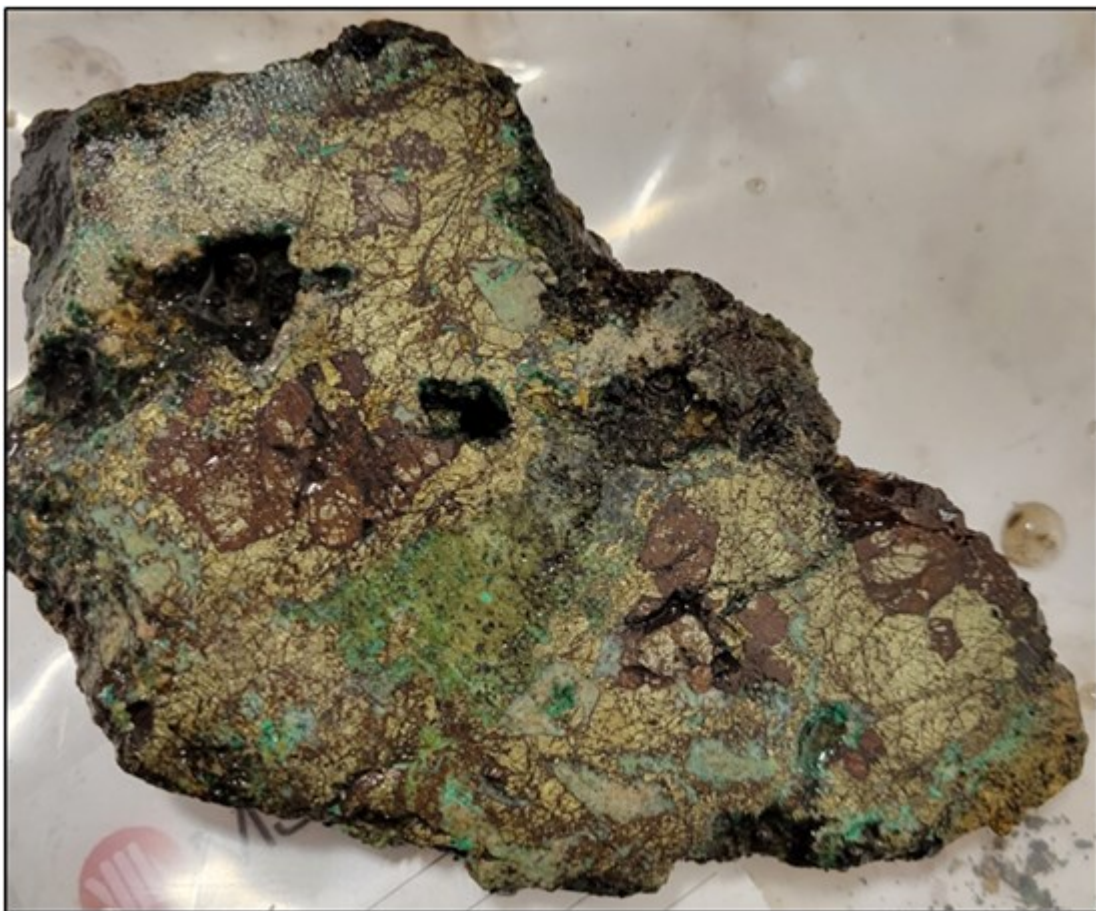
Photo 1: Select sample of moderately weathered massive chalcopyrite within the Big Cut Skarn grading 21% copper, 93 g/t silver
