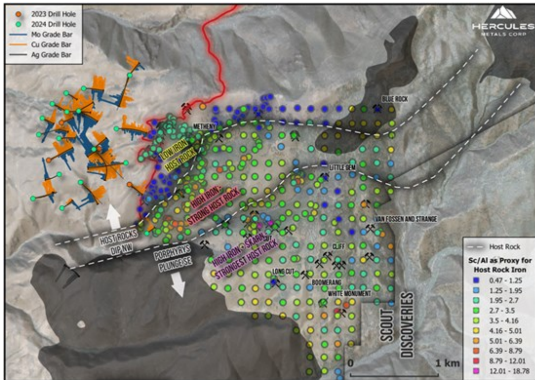
Figure 5 - Scandium (ppm) /Aluminum (%) as a proxy for silicate iron concentration in host rock.
