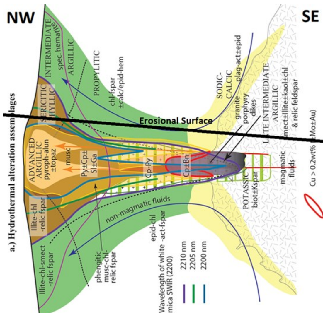
Figure 7 - Classic porphyry alteration model rotated 90 degrees for exaggeration to illustrate the expected surface alteration pattern at Leviathan.
