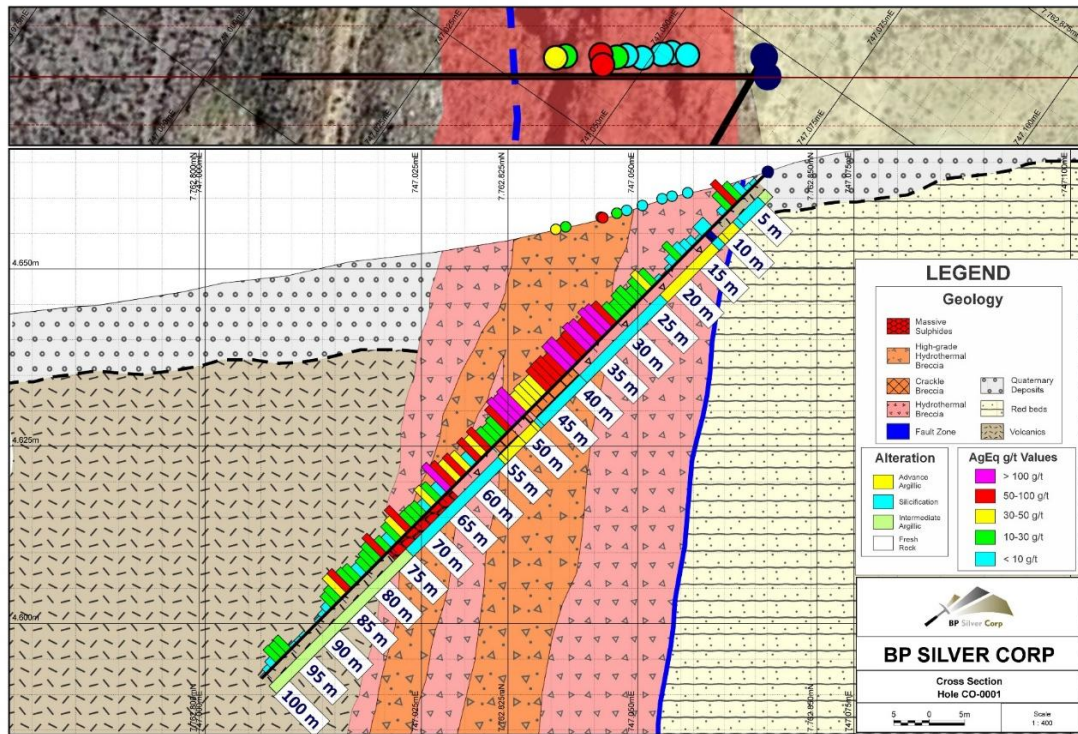
Figure 2: Jalsuri Target Cross Section illustrating surface geochemistry, hole CO-0001 trace, mineralization, alteration and geology.
