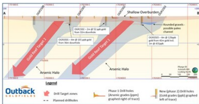
Figure 2 – Section A to B showing the near-surface Phase 1 arsenic drill results as well as Phase 2 top of bedrock air-core gold results. The interpreted gold reef targets are shown in red. Note, drilling vertical holes using air-core drilling techniques does not return core which can be oriented to allow an estimation of true widths of intercepts. All intercepts reported are at downhole lengths, no true width has been estimated. (CNW Group/Outback Goldfields Corp.)
