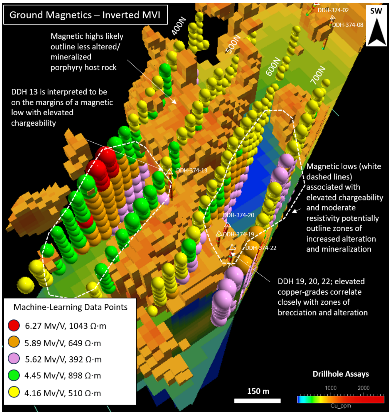
Figure 4: 2024 inverted ground magnetic data (MVI) with machine-learning cluster data outlining prospective zones with resistivity-chargeability anomalies associated with magnetic lows.
