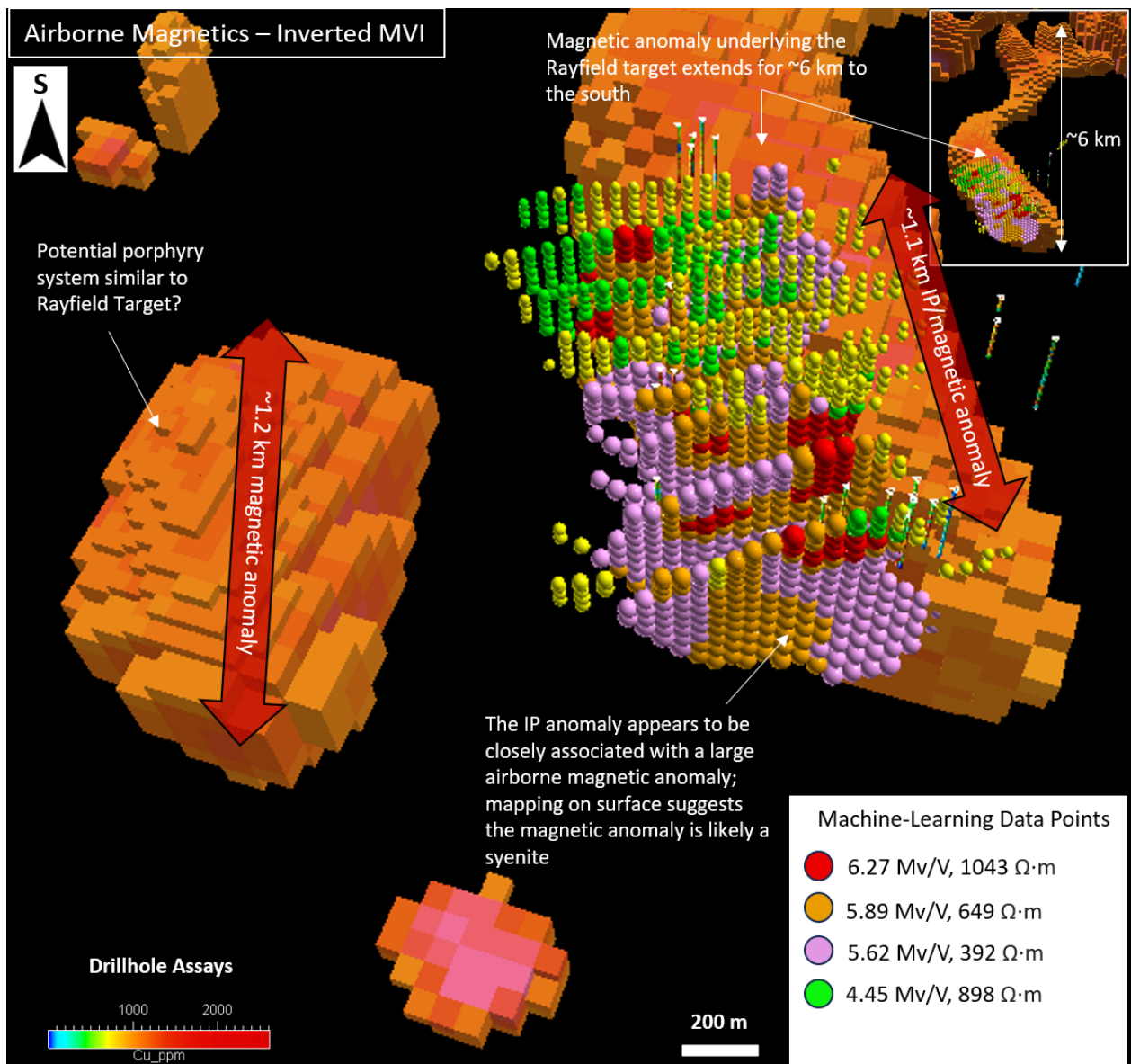
Figure 3: 2024 inverted airborne magnetic data (MVI) with machine-learning cluster data outlining prospective zones and a newly identified ~1.2 km magnetic anomaly to the east.
