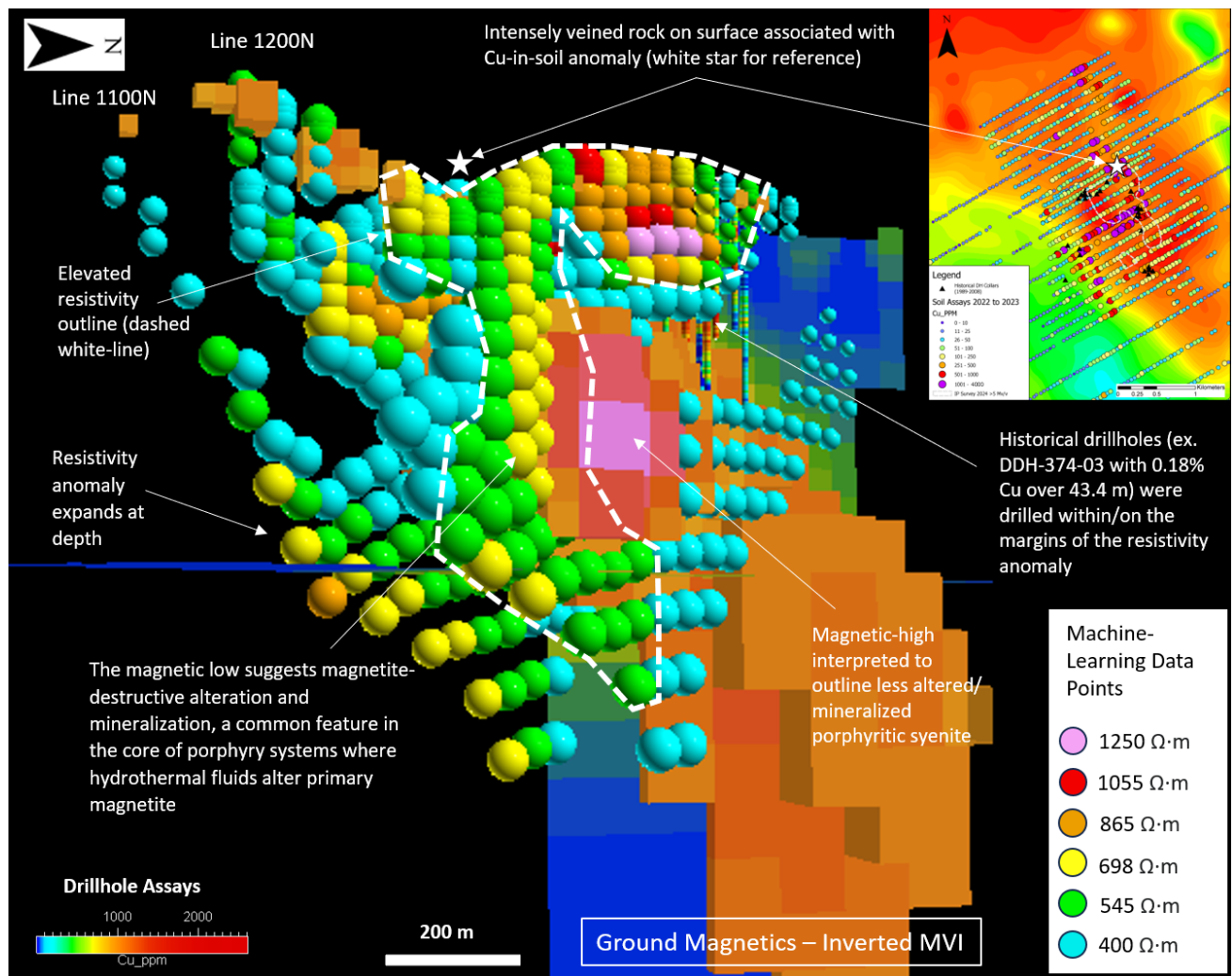
Figure 5: 2024 inverted ground magnetic data (MVI) with machine-learning cluster data outlining prospective zones with resistivity anomalies associated with the margins of an interpreted syenite intrusion.
