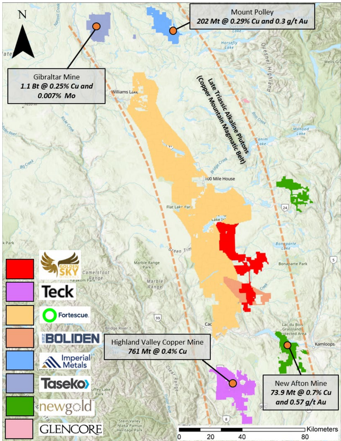
Figure 2: The ~50,800-hectare Rayfield Cu-Au Property is located within the Quesnel Trough, British Columbia's primary copper-producing belt.
