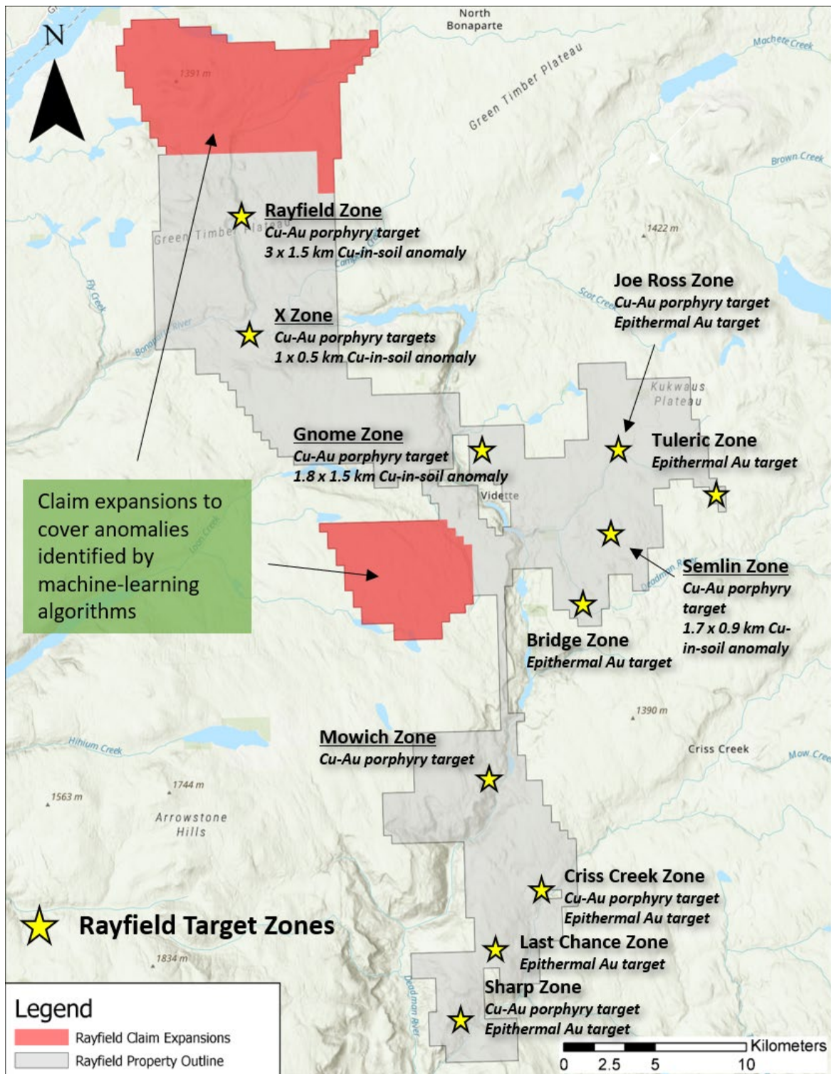
Figure 1: The Rayfield target zone is defined by a large 3.0 km x 1.5 km multi-element soil geochemical anomaly. The Rayfield target zone is highly prospective, with anomalous copper-in-soil values up to ~0.396%, and rock samples grading up to 0.63% Cu and 245 ppb Au. Based on newly identified geophysical anomalies through machine-learning algorithms, Golden Sky has expanded the existing property by 20% to total ~50,800 hectares.
