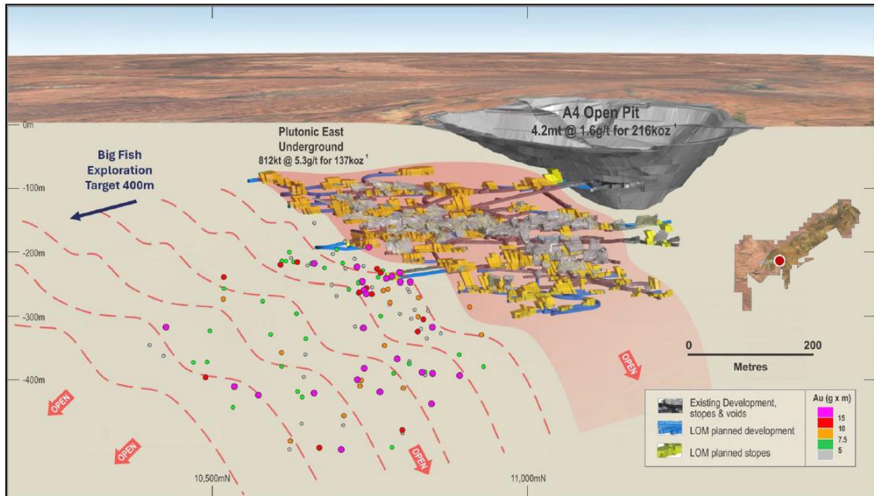
Figure 2: Plutonic East's mine plan showing mineralisation adjacent to planned work areas.
