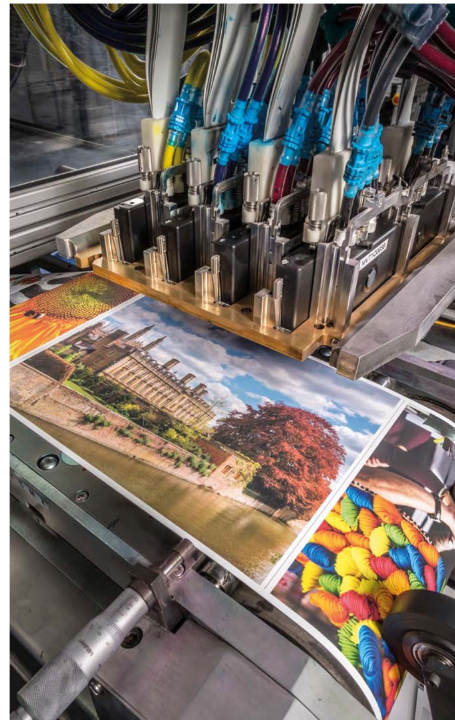
Xaar 5601 printheads in action
