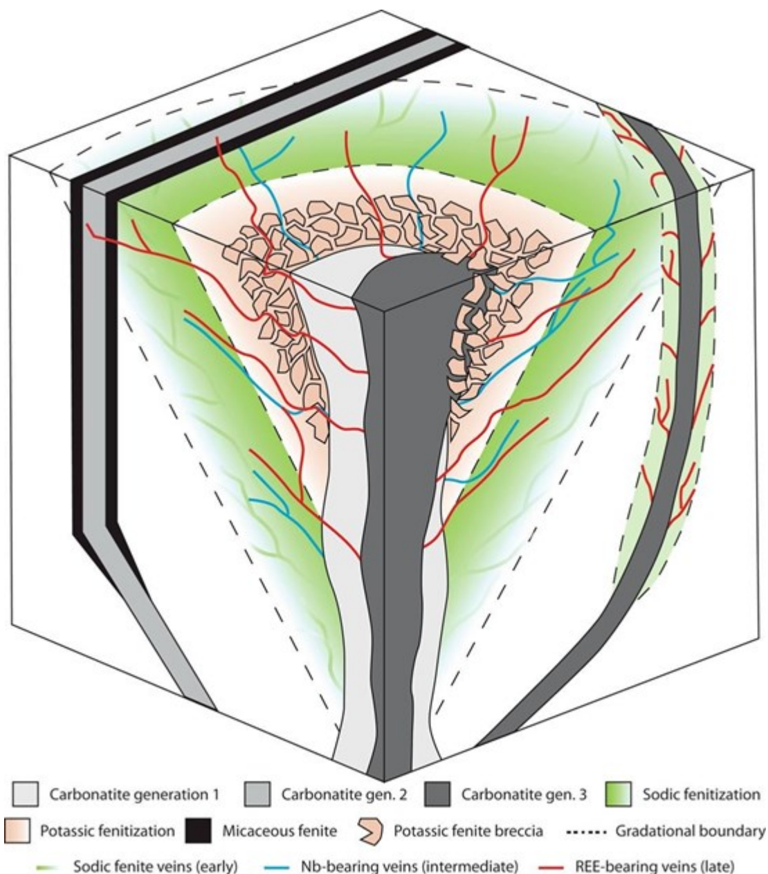
Figure 4. Idealized block diagram summarizing fenitization relationships and carbonatite pipe architecture at a generalized carbonatite complex (Elliot et al., 2018).
