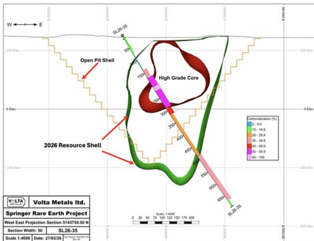
Figure 1. Drill hole SL26-35 cross section showing volume % carbonatite mineralization from detailed geological logging, 2026 resource estimate shell and conceptual open pit outline (visual estimates of carbonatite do not necessarily indicate the presence of REE and Ga mineralization. Assays are pending).
