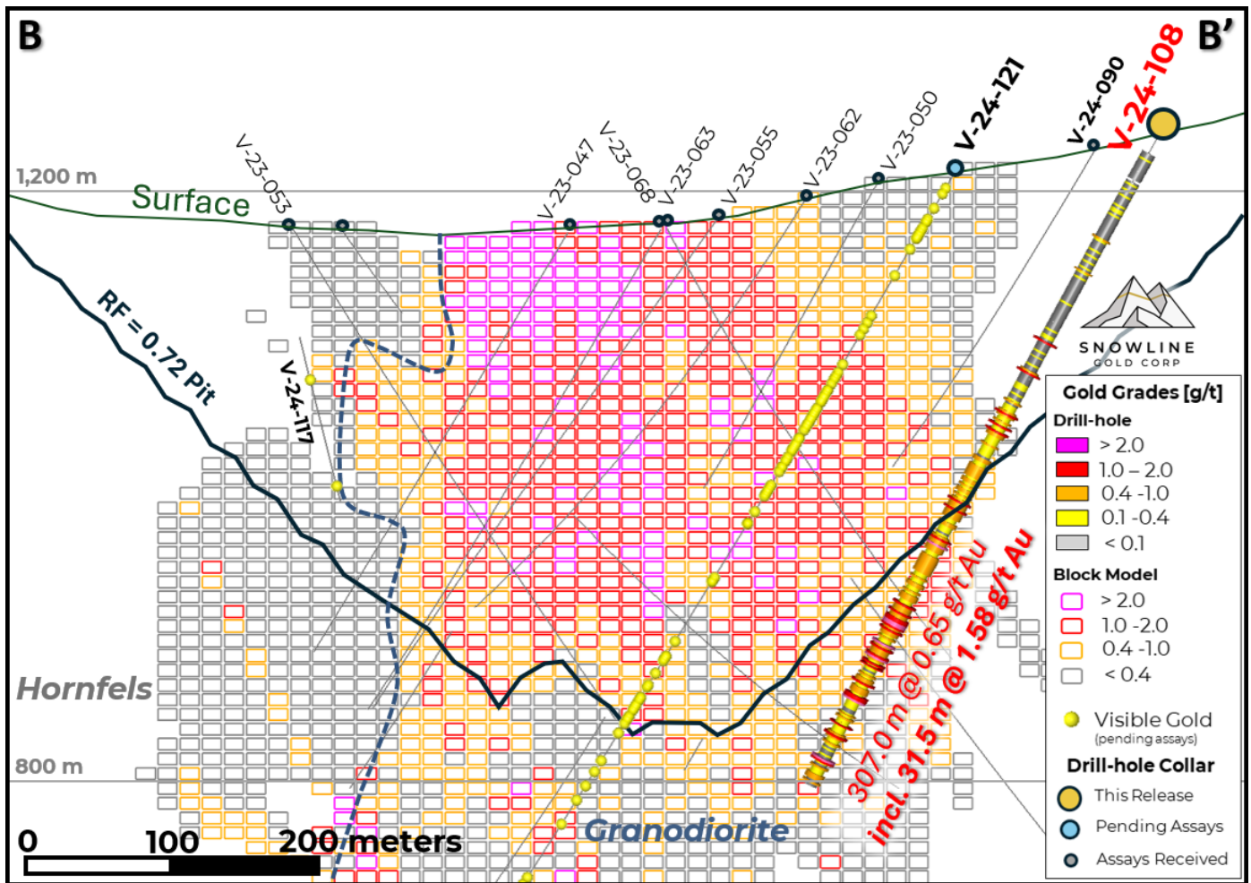
Figure 3 – Cross-section B-B', showing V-24-108 in the context of the initial Valley MRE block model and MRE-constraining revenue factor 0.72 pit shell. Note that most of the mineralization in the hole is outside the current resource-limiting pit shell. The block model has not been updated to reflect the current results, nor any results to date from 2024 (bold labels). Blocks shown outside of the current pit shell constraint are not included in the initial MRE for Valley. Areas without blocks have not been modelled and were assumed as nil for the initial Valley MRE. Instances of visible gold in holes still awaiting assay results are marked by yellow spheres.
