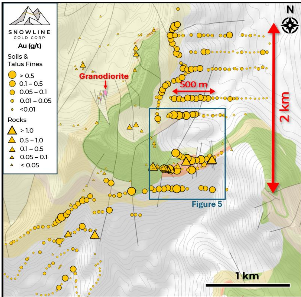
Figure 6 – Broad-scale view of the Aurelius target , showing the context of Figure 5 drill locations amidst a wider geochemical anomaly accompanied by widespread hydrothermal alteration associated with proximal (and possibly buried) mid-Cretaceous granodioritic intrusions.
