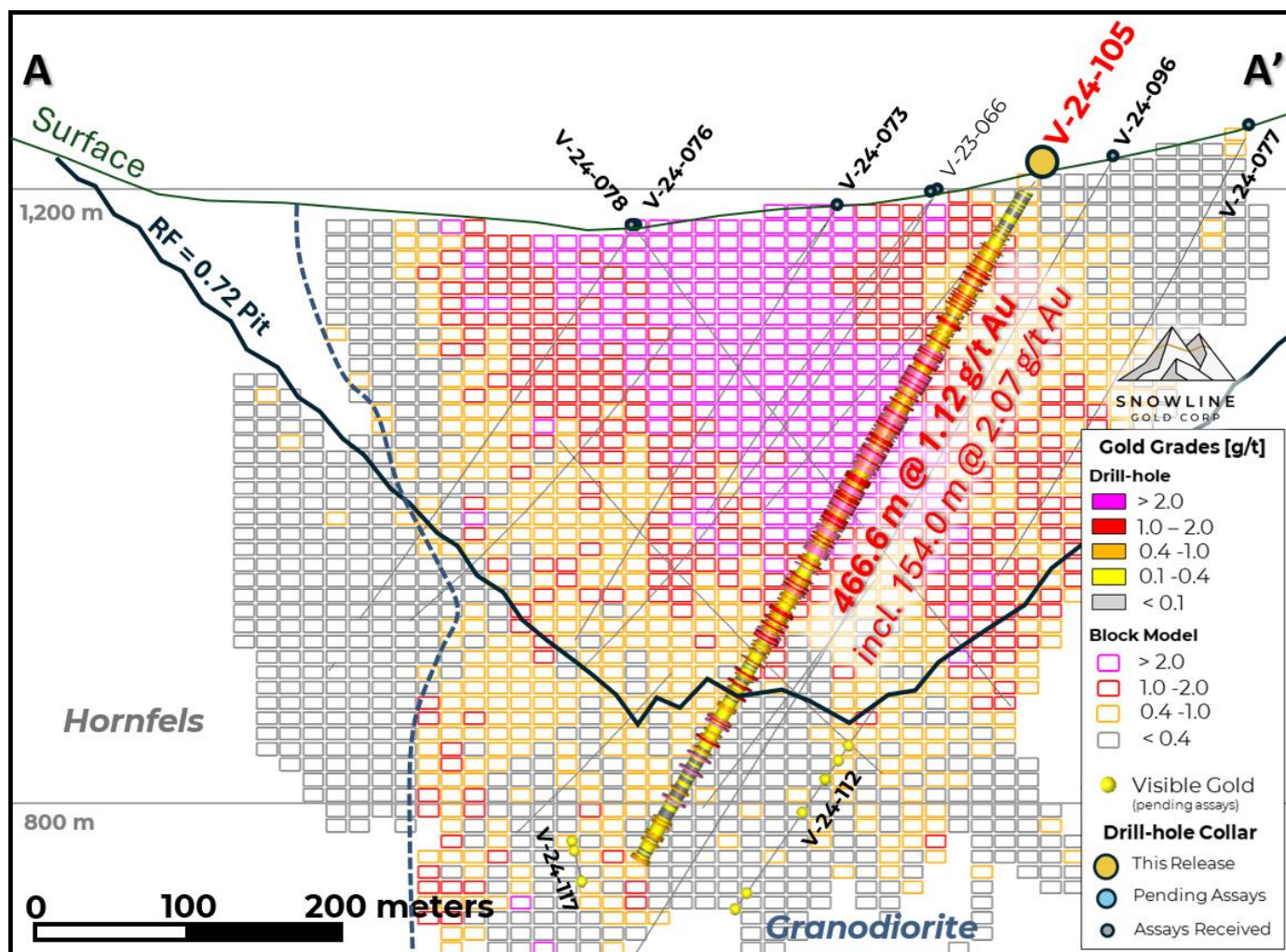
Figure 2 – Cross-section A-A', showing V-24-105 in the context of the initial Valley MRE block model and MRE-constraining revenue factor 0.72 pit shell. The block model has not been updated to reflect the current results, nor any results to date from 2024 (bold labels). Blocks shown outside of the current pit shell constraint are not included in the initial MRE for Valley. Areas without blocks have not been modelled and were assumed as nil for the initial Valley MRE. Instances of visible gold in holes still awaiting assay results are marked by yellow spheres.
