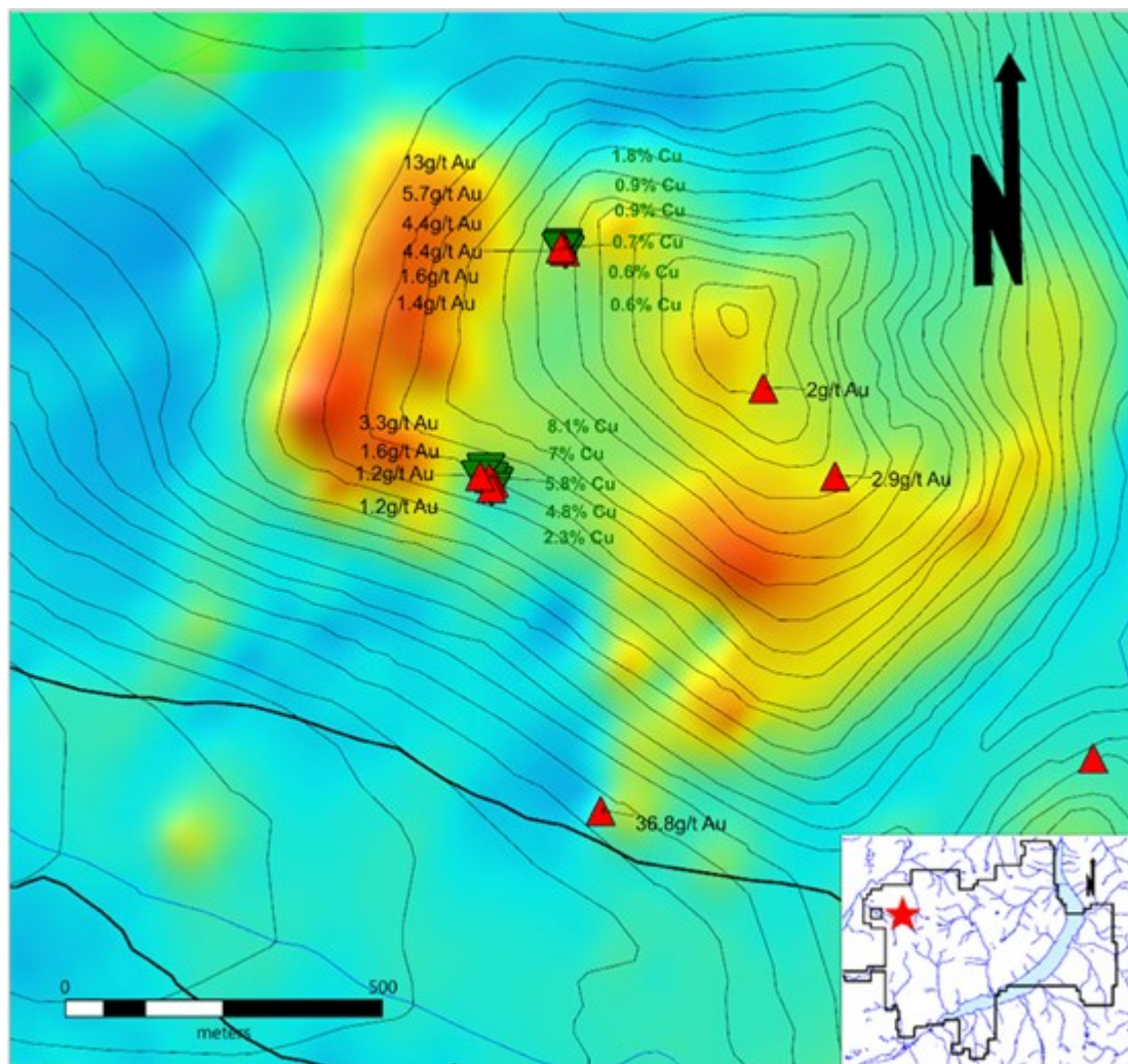
Figure 2: Total magnetic intensity map from the Ruffner area showing sample locations and assay results. The data suggest the mineralized porphyry may extend ~1 km in strike length.
