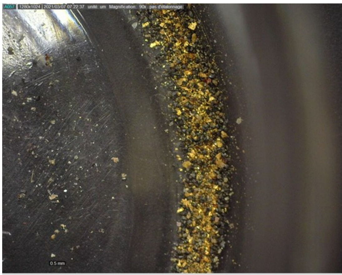
Image of recovered gold from Megantic overburden sample 798741. Magnification 90X, Scale 0.5 mm (bottom right)
