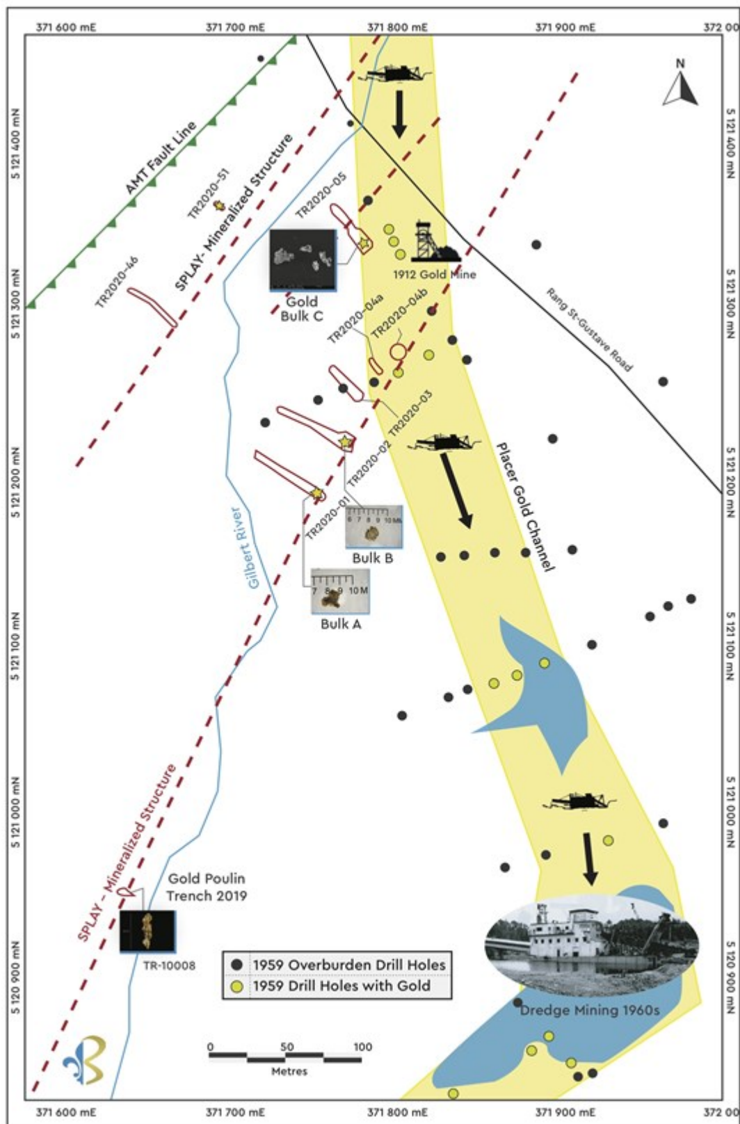
Figure 1: Layout of trenches, Placer Channel, main Fault, Splays and Bulk samples A, B, C.
