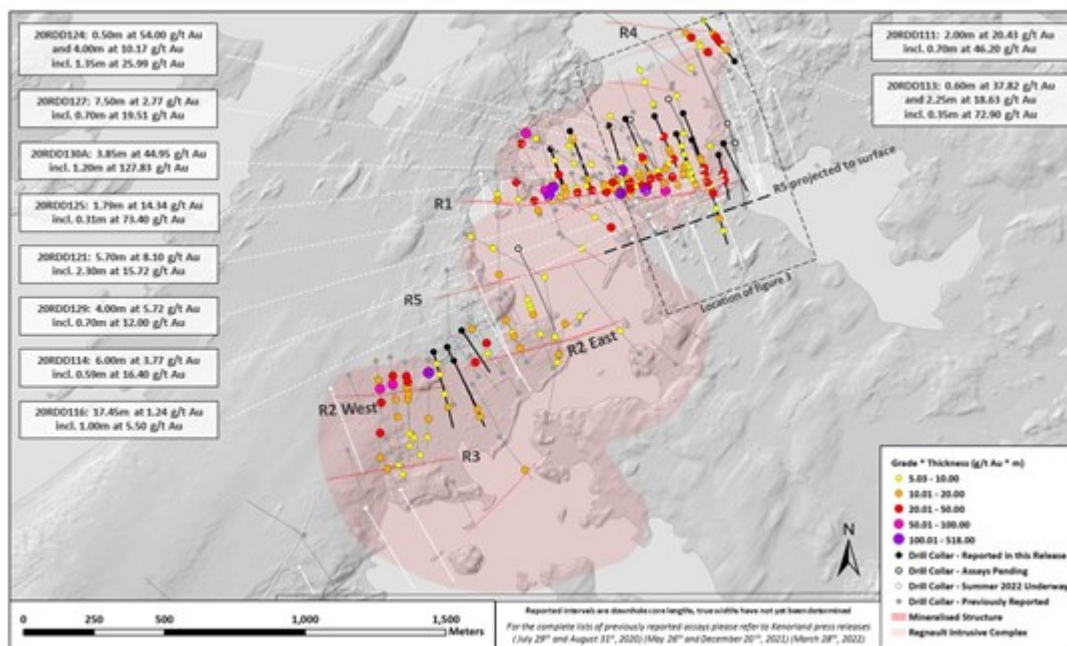
Figure 1. Plan map of Regnault drilling (reported, assays pending, and current program)
