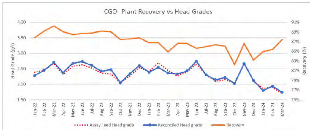
Figure 17-3 Tuckabianna process recoveries v. head grade: Westgold.
