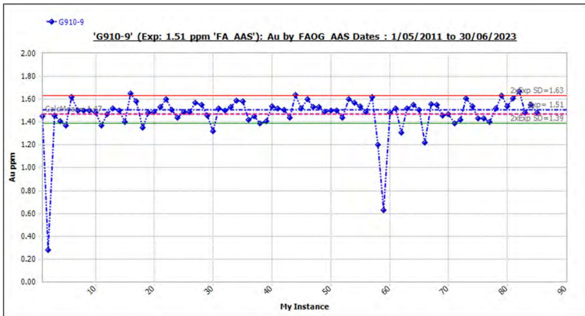
Figure 11-24 Standard G910-9: Outliers Included.
