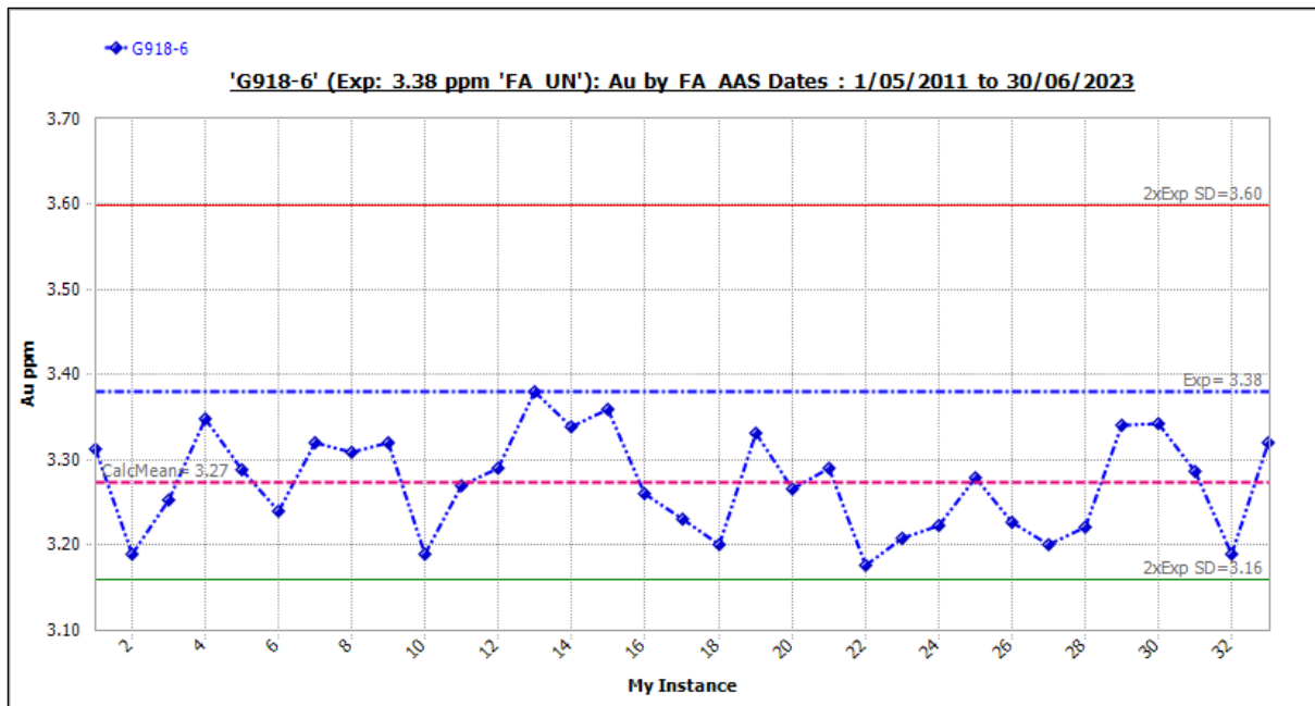
Figure 11-36 Standard G918-6: Outliers Included.
