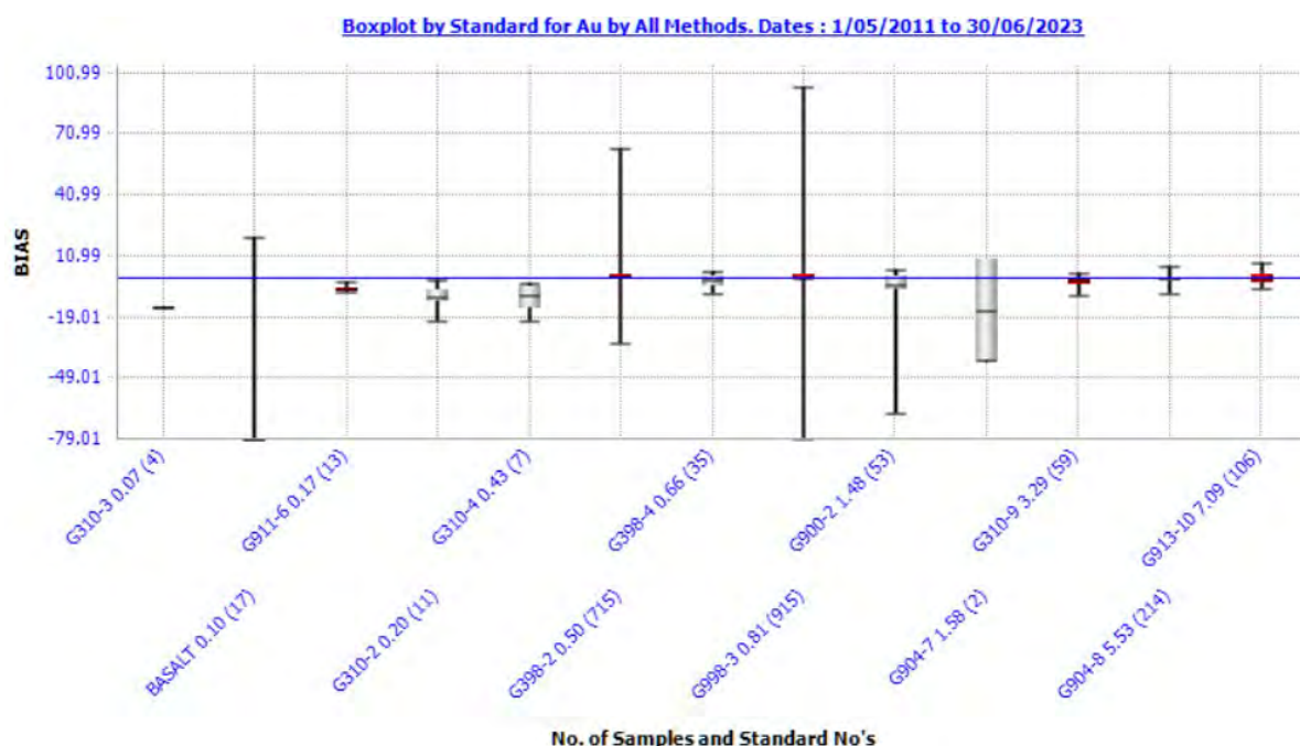
Figure 11-43 Boxplot by Standard for Au by Fire Assay (all methods).
