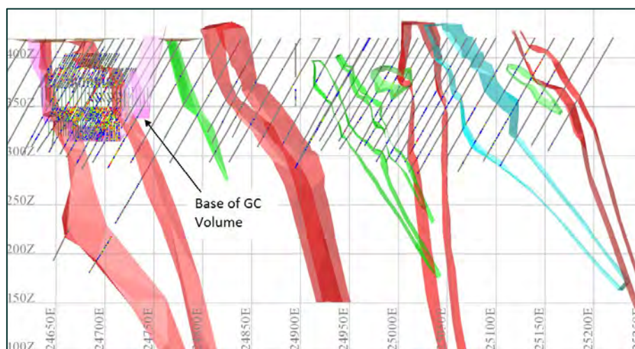
Figure 14-33 Black Swan South base of grade control drilling volume – domain 3100 at cross section 28,680 mN +/- 10 m. Source: Westgold.
