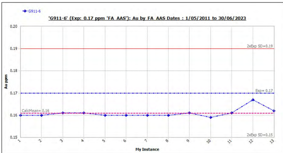
Figure 11-25 Standard G911-6: Outliers Included.
