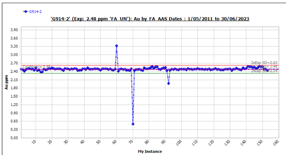
Figure 11-27 Standard G914-2: Outliers Included.
