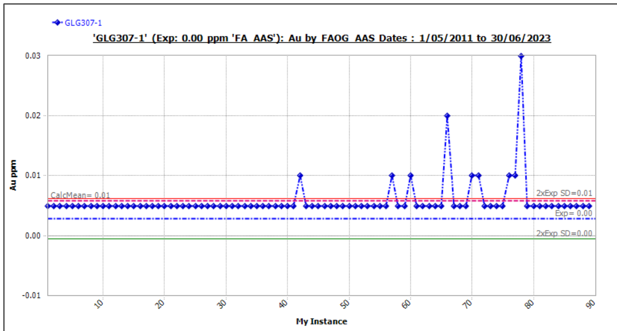
Figure 11-38 Standard GLG307-1: Outliers Included.
