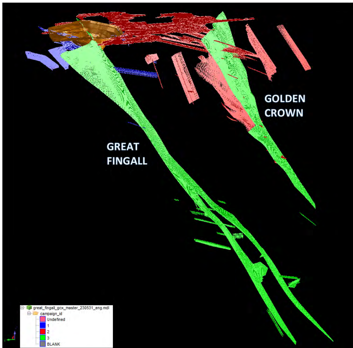
Figure 14-56 Combined Great Fingall - Golden Crown model. Mineralisation domains by campaign_id. Mineralisation domains in blue and red have had all attributes imported from the preceding 2022 model. Note - Mineralisation domains in red are unchanged from the 2016 Golden Crown model. Source: Westgold.
