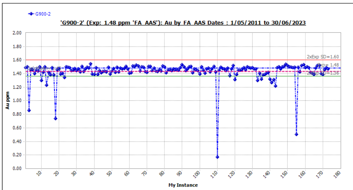
Figure 11-21 Standard G900-2: Outliers Included.
