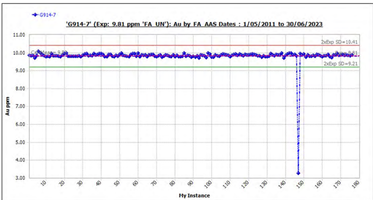
Figure 11-29 Standard G914-7: Outliers Included.
