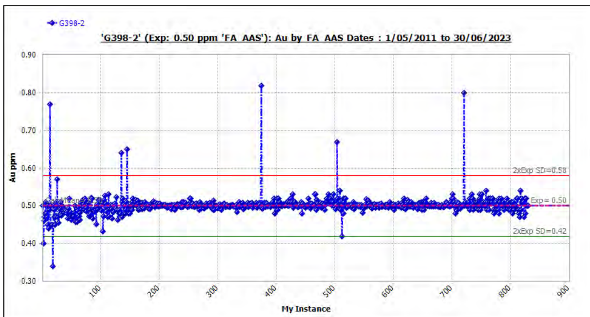
Figure 11-19 Standard G398-2: Outliers Included.
