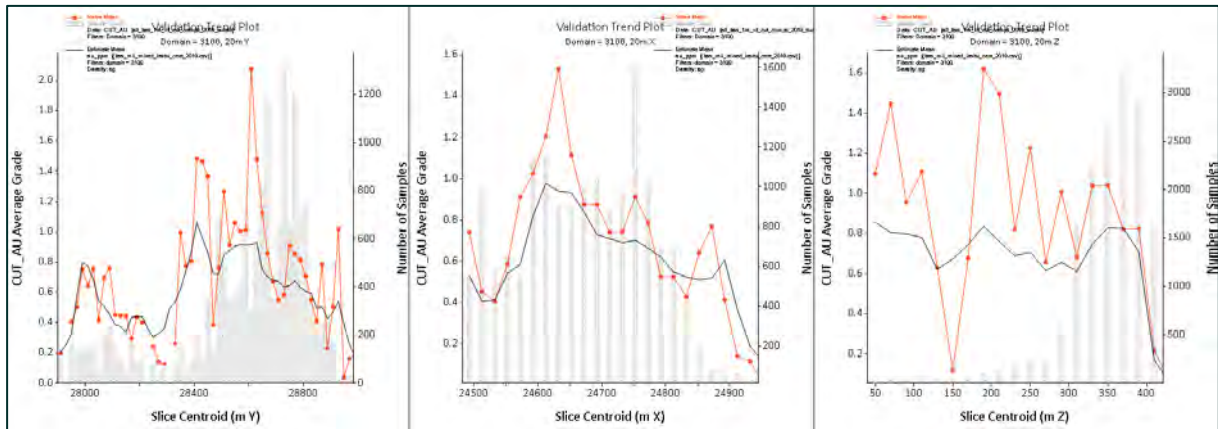
Figure 14-38 Black Swan South swath plots for domain 3100. Source: Westgold.
