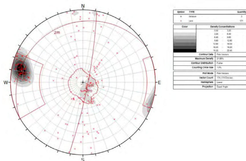
Figure 16-11 Fender defect orientation data obtained from pit mapping. Source: Westgold.
