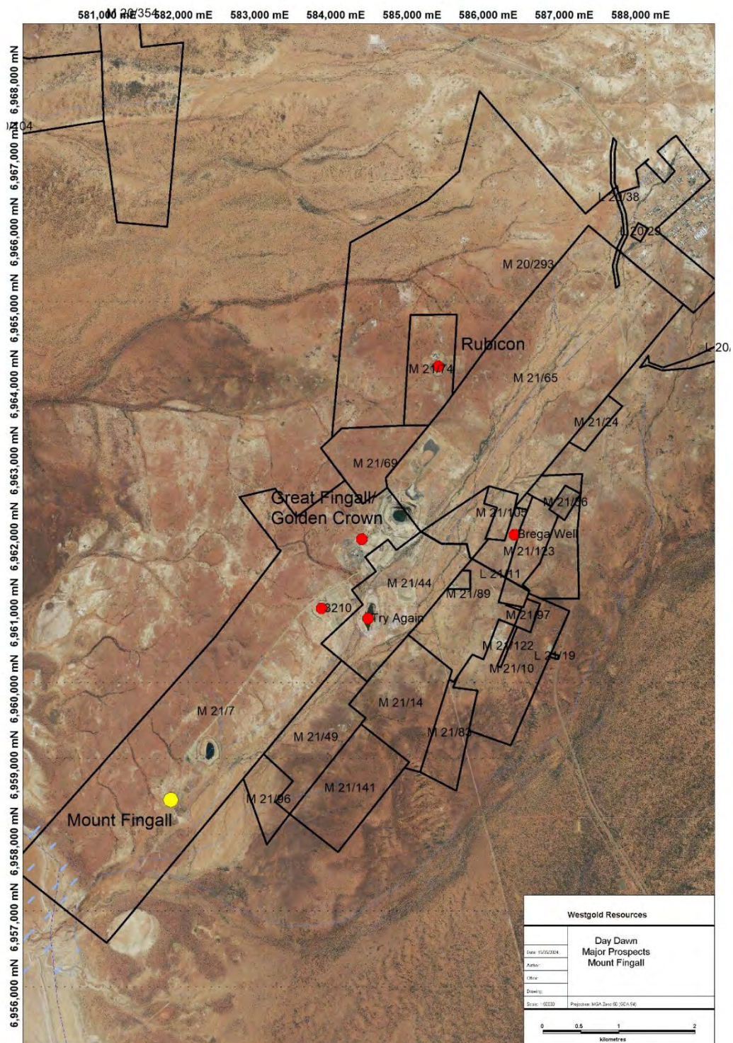
Figure 14-61 Mount Fingall location map. Source: Westgold.
