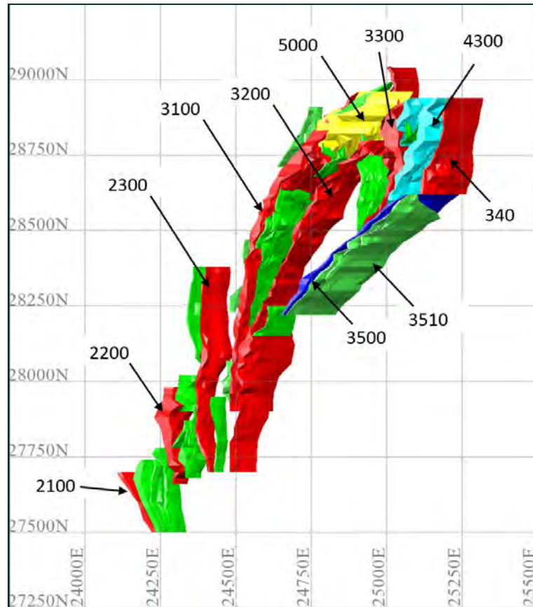
Figure 14-29 Black Swan South porphyry interpretation domains. Source: Westgold.
