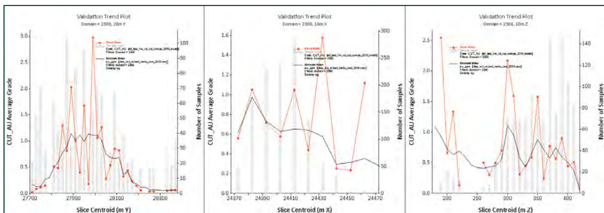
Figure 14-37 Black Swan South swath plots for domain 2300. Source: Westgold.
