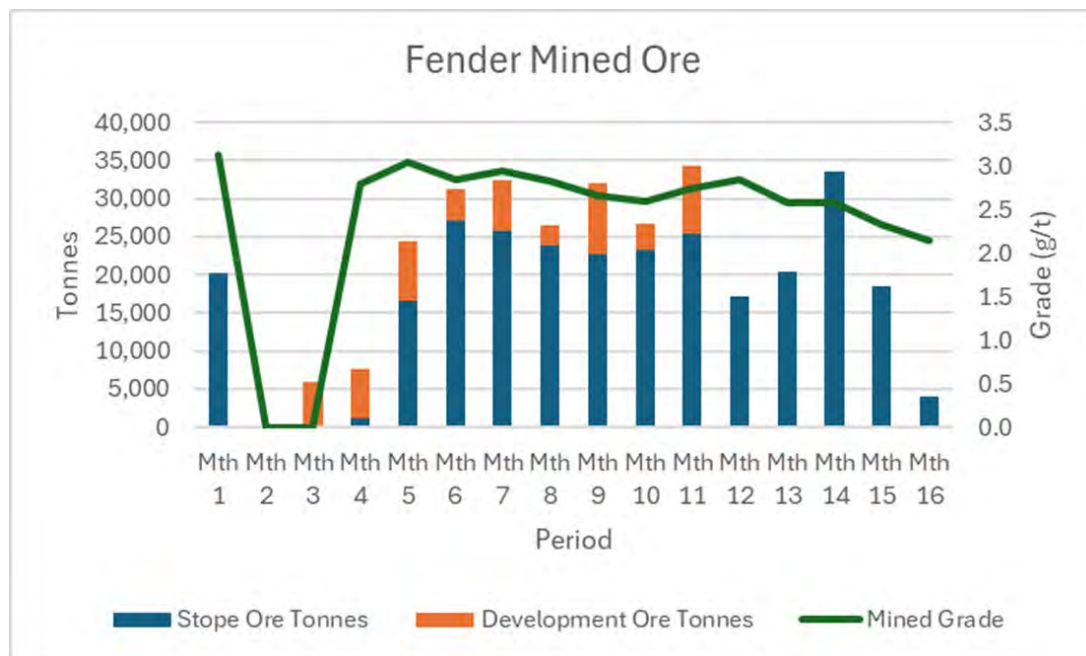
Figure 16-20 Fender Underground schedule. Source: Westgold.
