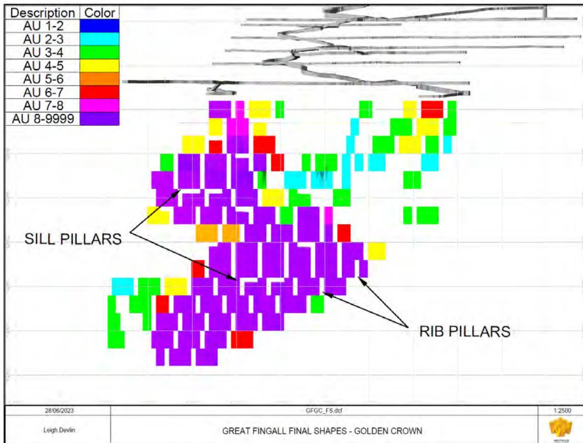
Figure 16-27 Great Fingall – Golden Crown final stope shapes output. Source: Westgold.
