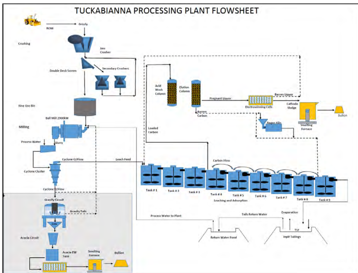
Figure 17-1 Tuckabianna process flowsheet 2023. Source: Westgold.
