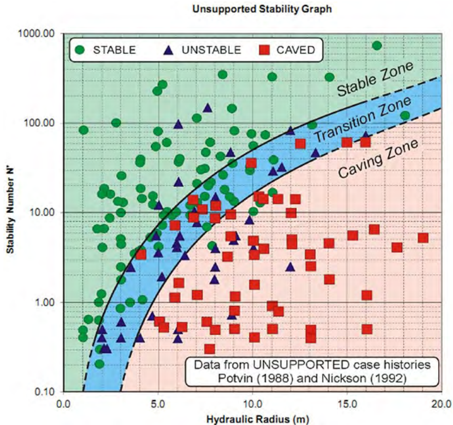
Figure 16-32 Unsupported case histories stability graph method chart.
