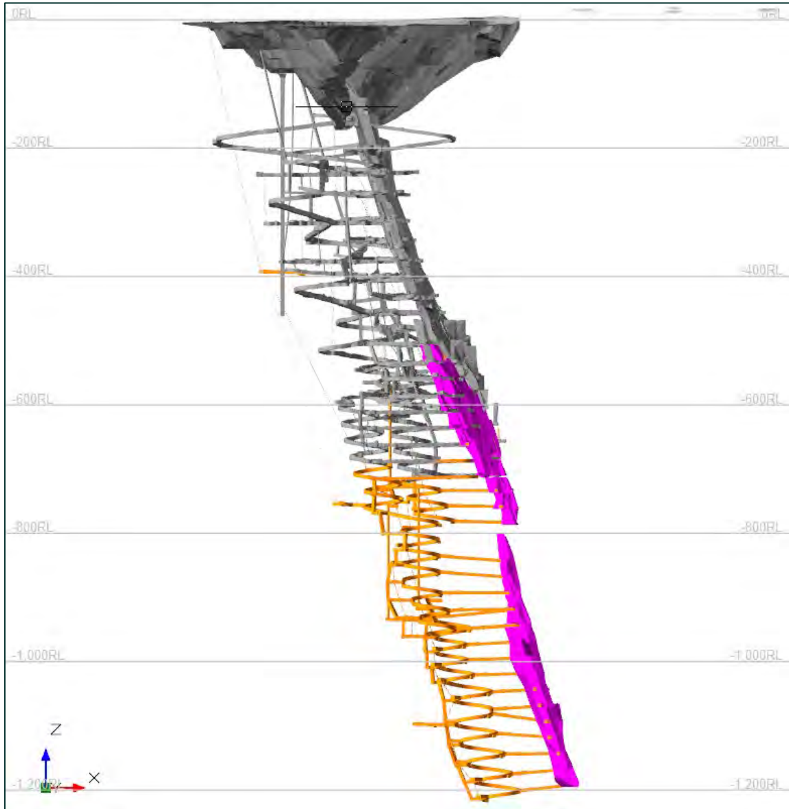
Figure 16-9 Big Bell Mineral Reserves showing existing pit and workings looking north. Source. Source: Westgold.
