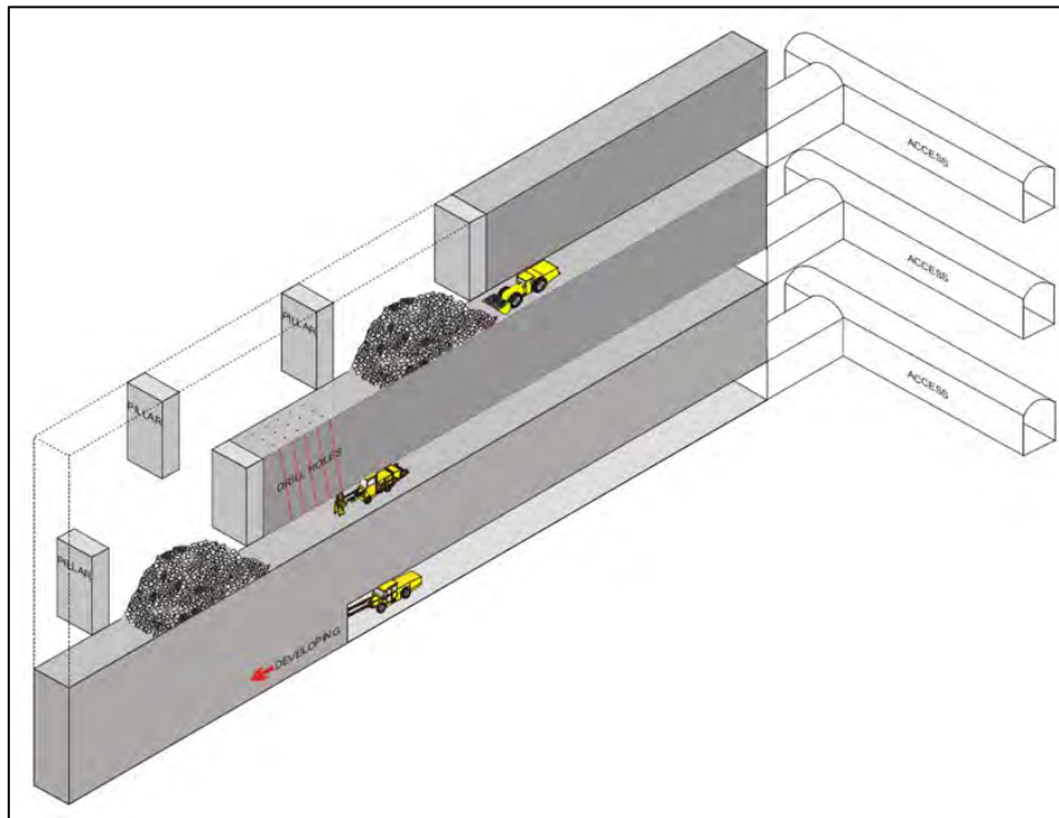
Figure 16-21 Uphole bench retreat example. Source: Westgold.
