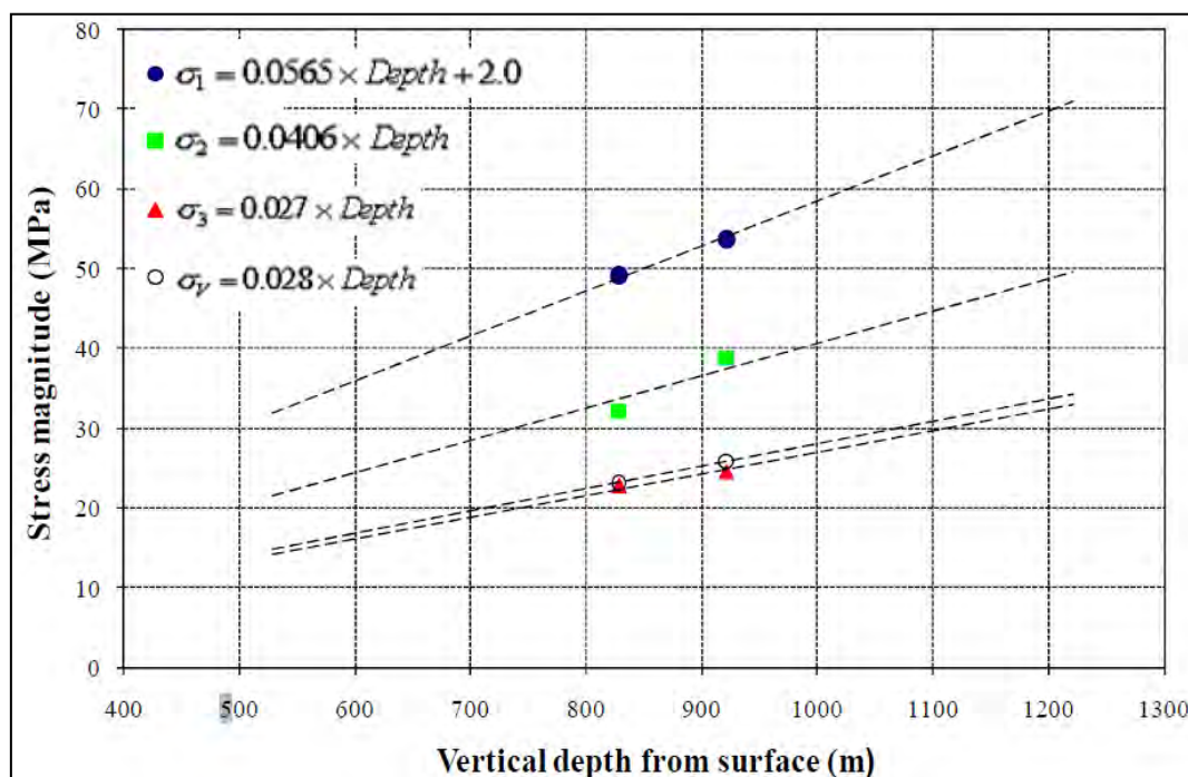
Figure 16-4 Relationship of principal stress at Big Bell with depth (Acoustic Emission results). Source: Westgold.
