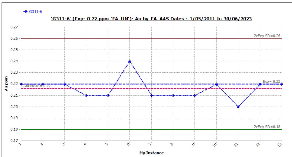
Figure 11-9 Standard G311-6: Outliers Included.
