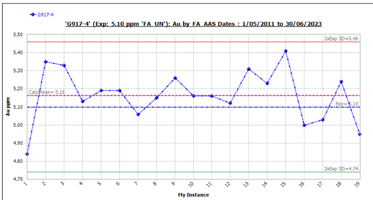
Figure 11-35 Standard G917-4: Outliers Included.
