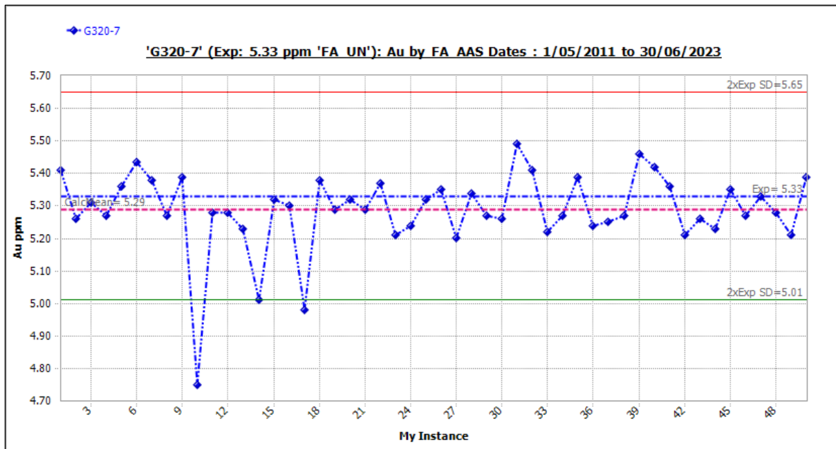
Figure 11-18 Standard G320-7: Outliers Included.
