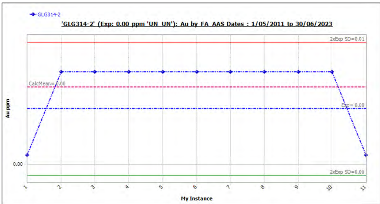
Figure 11-39 Standard GLG314-2: Outliers Included.
