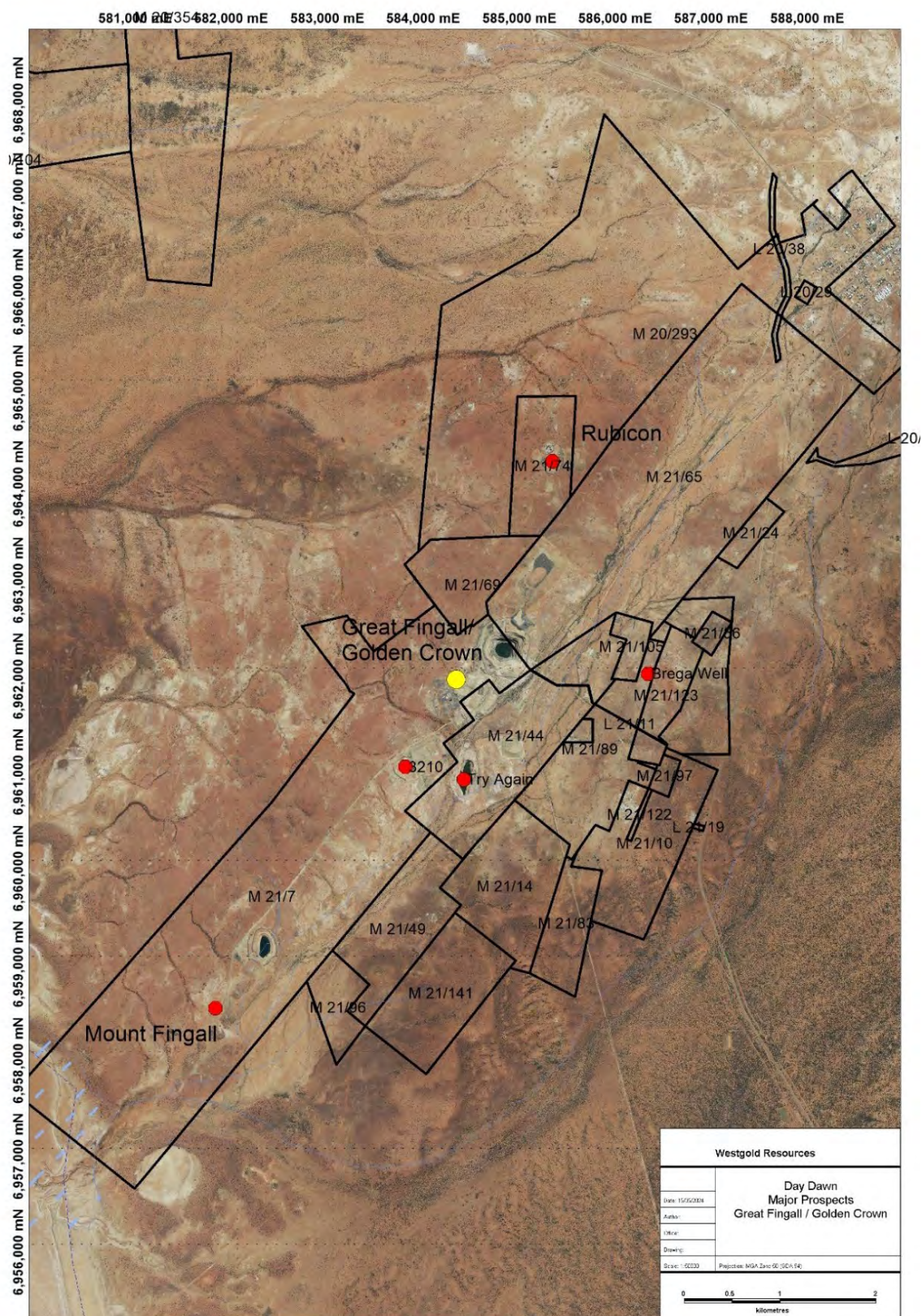
Figure 14-48 Great Fingall – Golden Crown location map. Source: Westgold.
