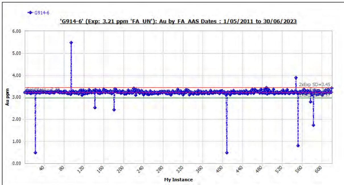
Figure 11-28 Standard G914-6: Outliers Included.
