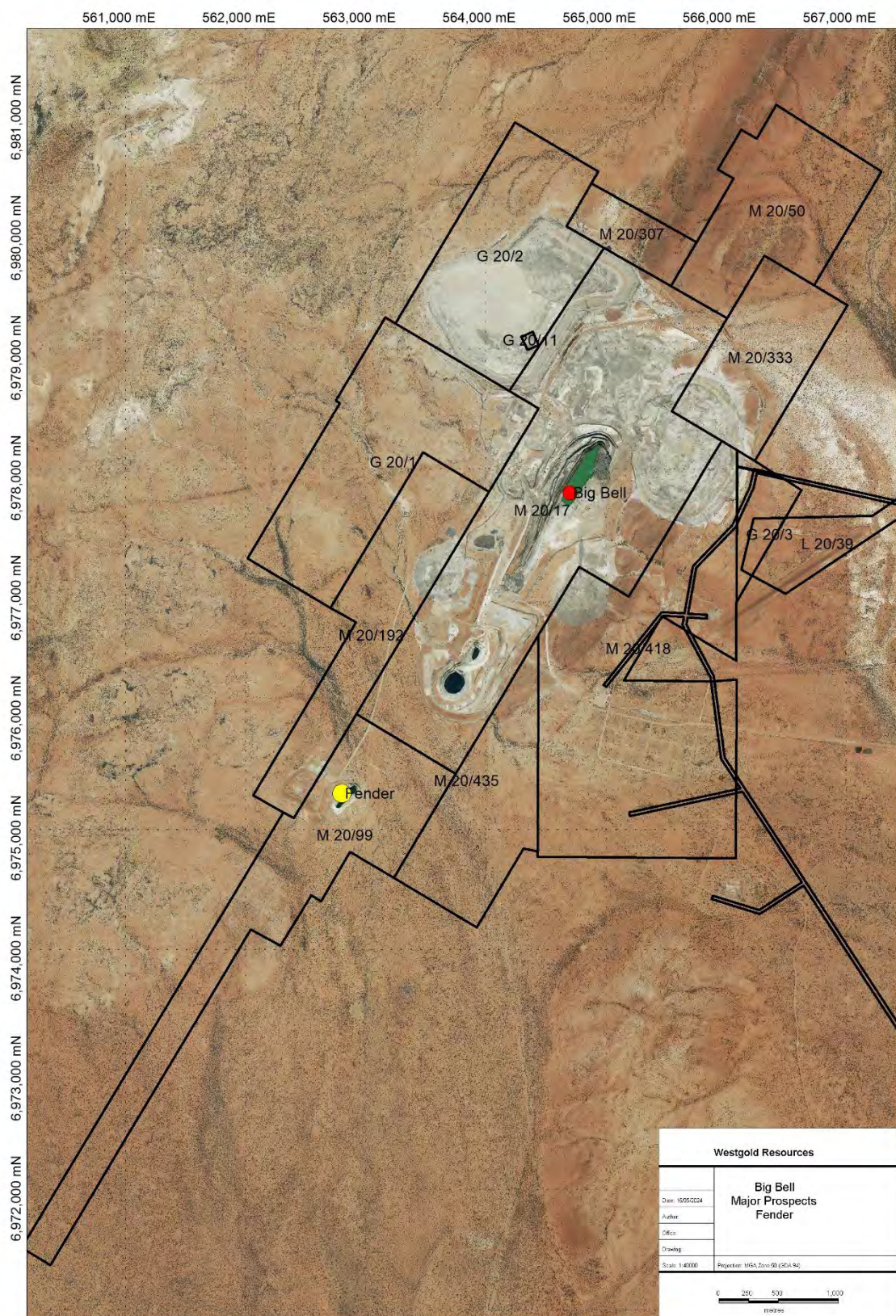
Figure 14-26 Fender location map. Source: Westgold.
