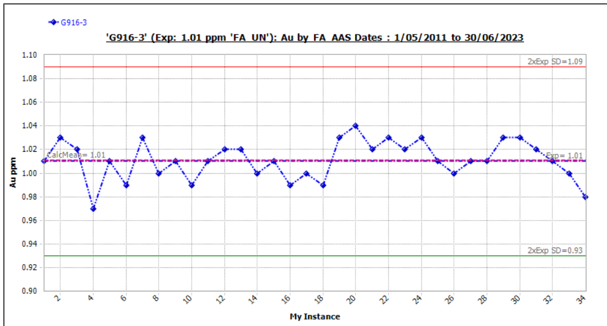
Figure 11-32 Standard G916-3: Outliers Included.
