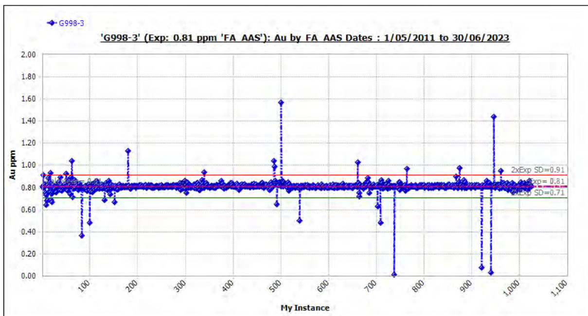
Figure 11-37 Standard G998-3: Outliers Included.
