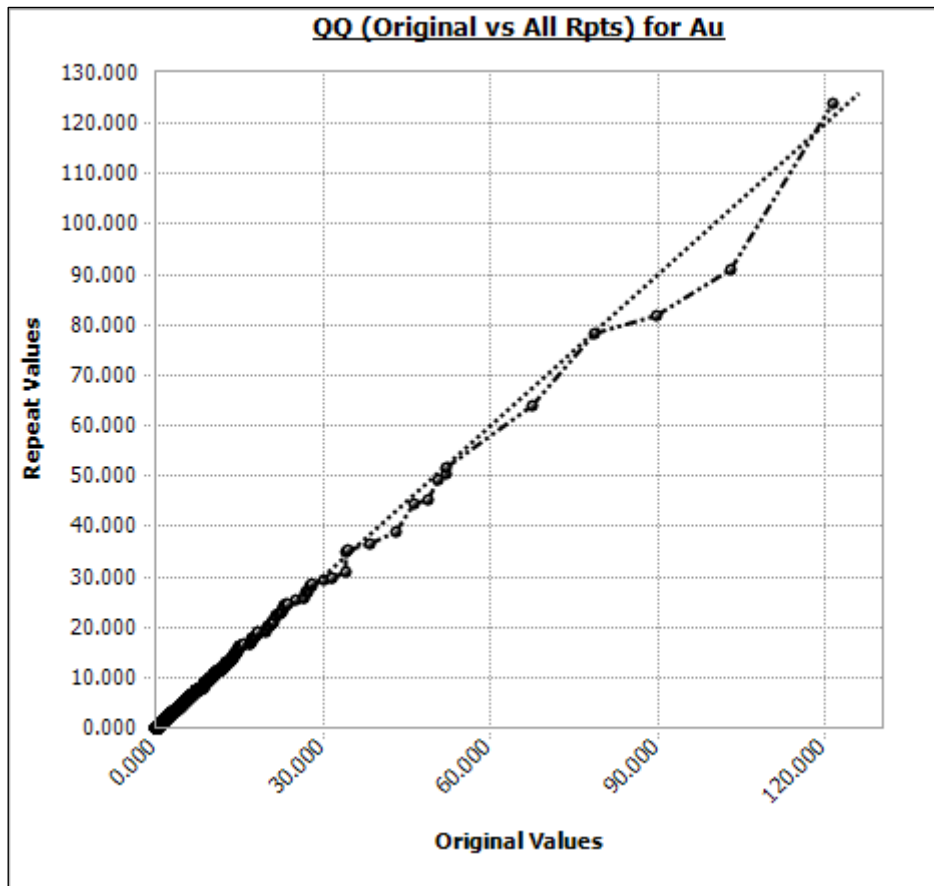
Figure 11-40 Q-Q Plot - Drillhole (Repeat Code) : Original v. All Rpts for Au ppm.
