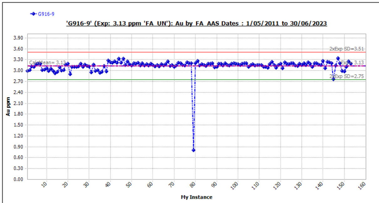
Figure 11-34 Standard G916-9: Outliers Included.
