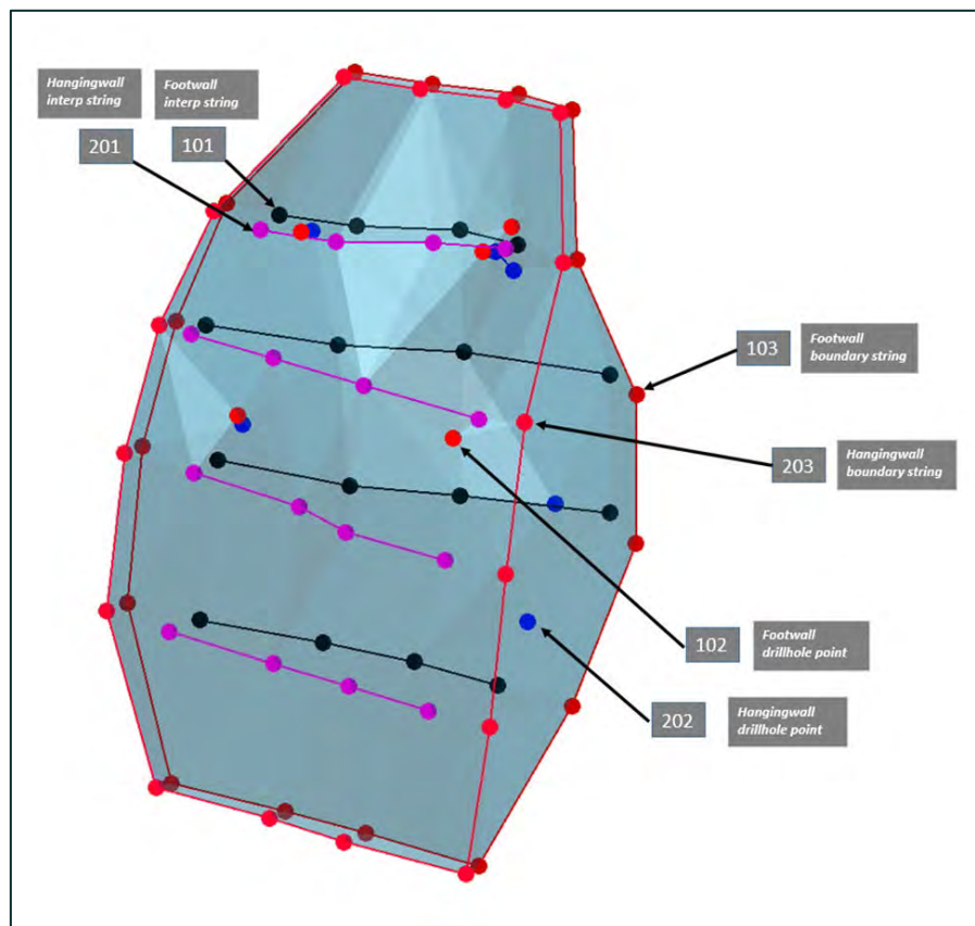
Figure 14-19 Example of hangingwall and footwall wireframe generation strings and points. Source: Westgold.
