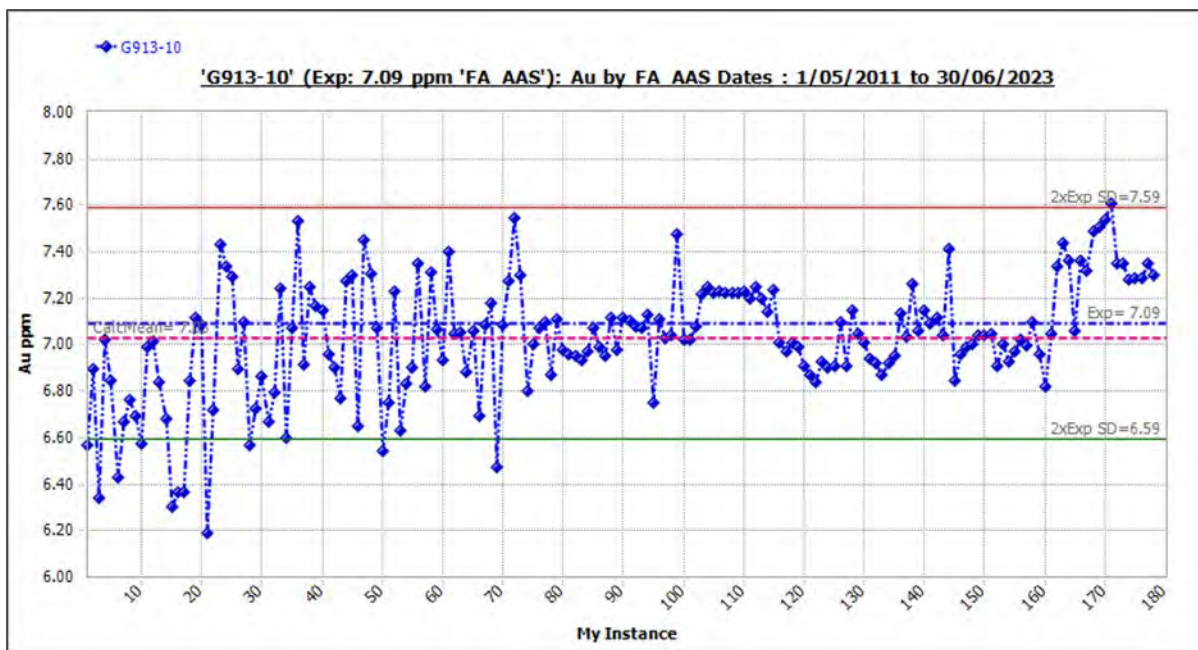
Figure 11-26 Standard G913-10: Outliers Included.
