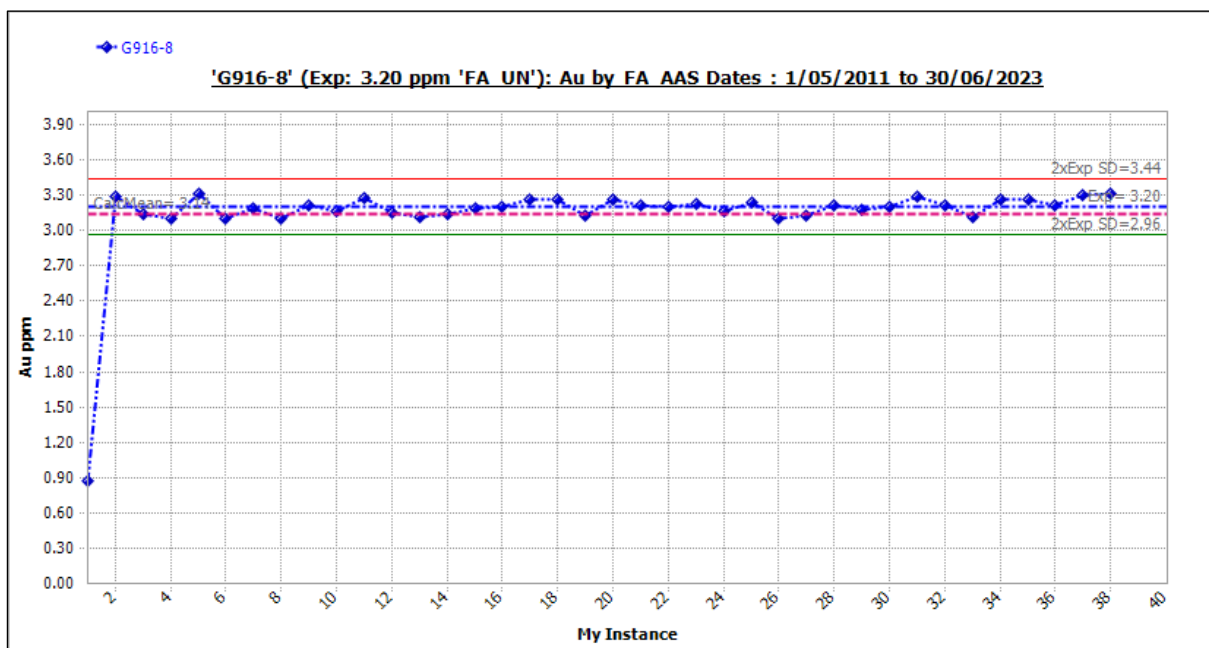
Figure 11-33 Standard G916-8: Outliers Included.
