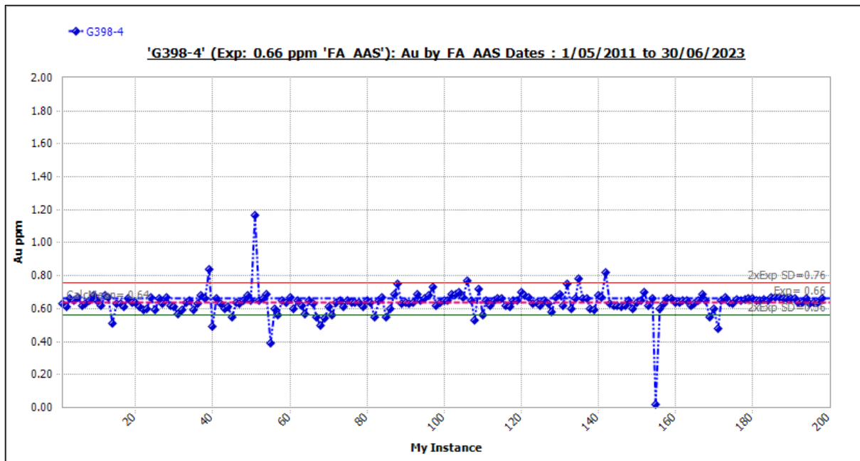
Figure 11-20 Standard G398-4: Outliers Included.
