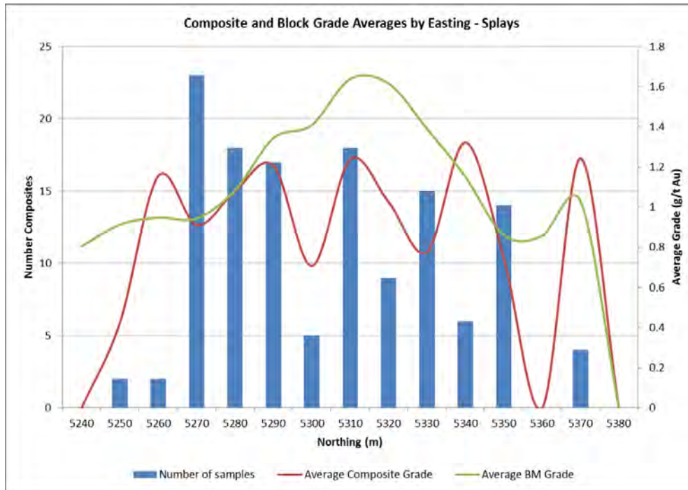
Figure 14-46 Composite and block grade averages by easting for (a) the 3210 main shear zone (object 3); (b) The 3210 footwall splays. Source: Westgold.
