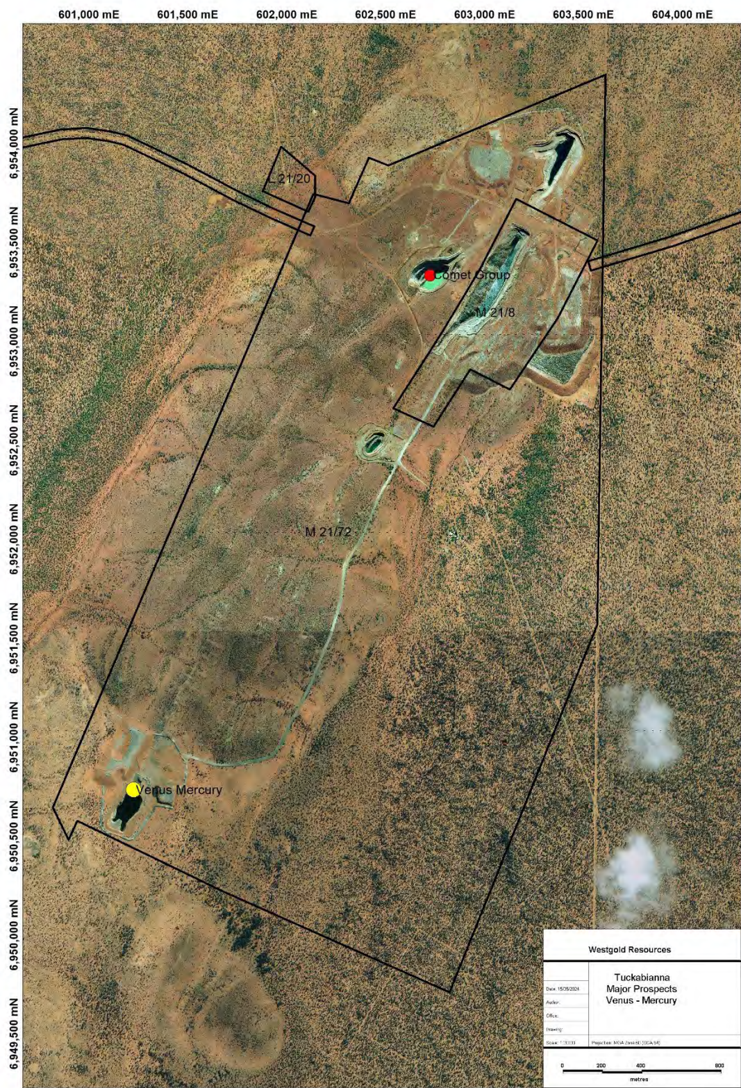
Figure 14-73 Venus - Mercury location map. Source: Westgold.
