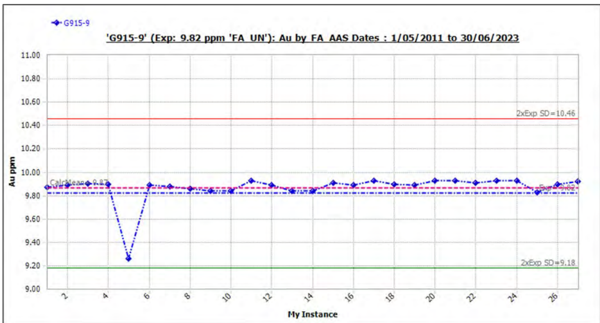
Figure 11-31 Standard G915-9: Outliers Included.
