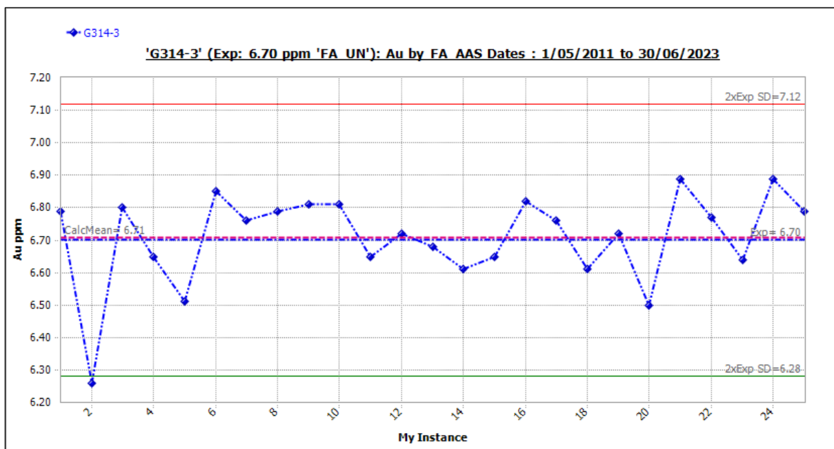
Figure 11-13 Standard G314-3: Outliers Included.
