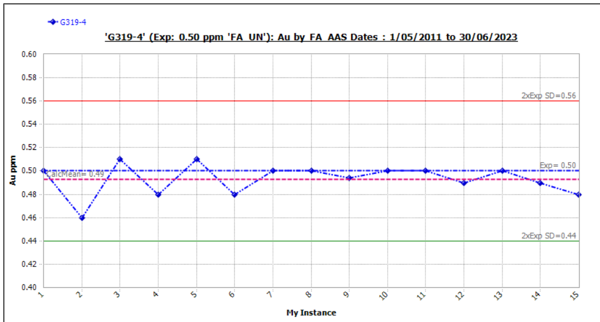
Figure 11-16 Standard G319-4: Outliers Included.
