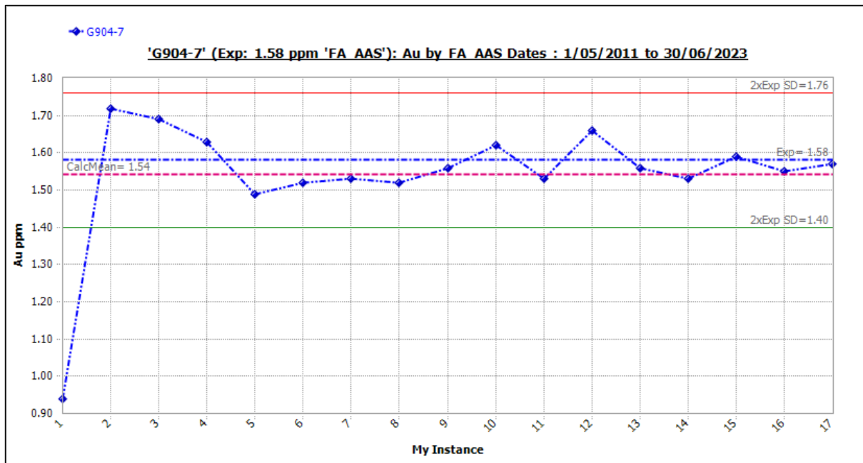
Figure 11-22 Standard G904-7: Outliers Included.
