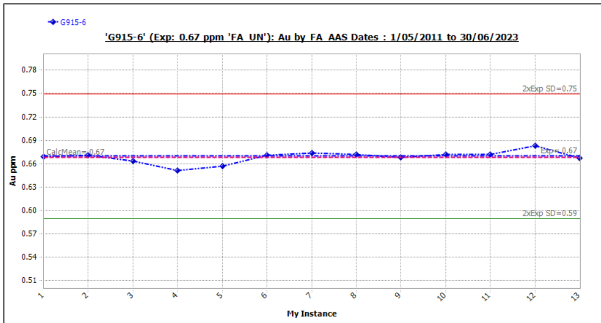
Figure 11-30 Standard G915-6: Outliers Included.
