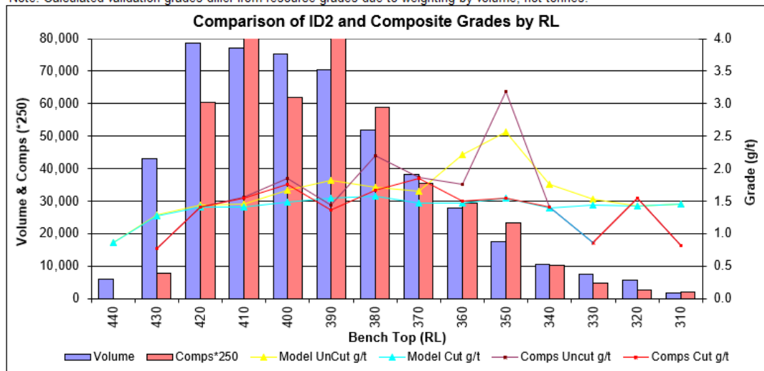
Figure 14-74 Model validation in the Venus - Mercury November 2011 MRE (all domains, validation by RL). Source: Westgold.
