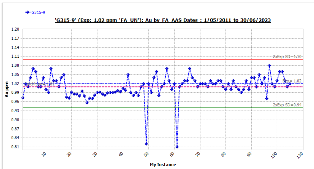
Figure 11-15 Standard G315-9: Outliers Included.
