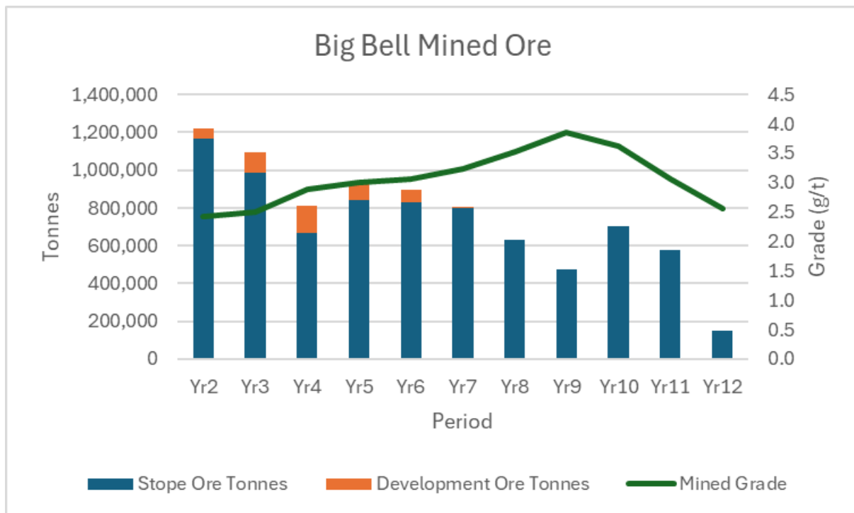
Figure 16-10 Big Bell Life of Mine schedule. Source: Westgold.
