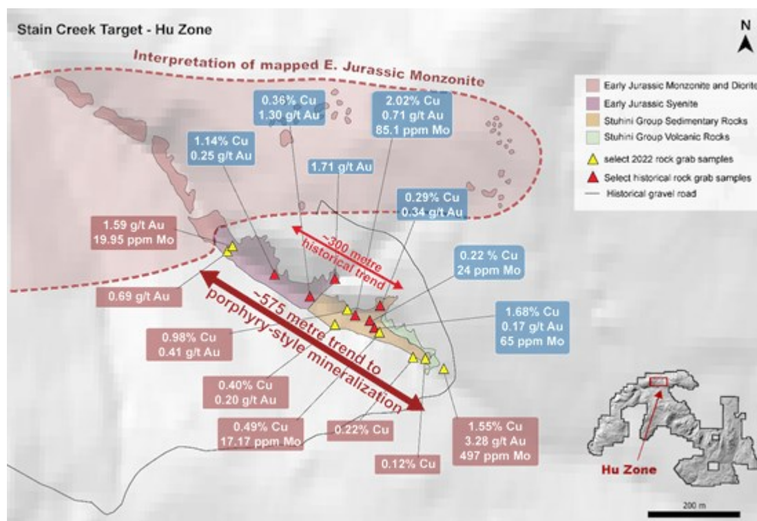
Figure 1. Select rock grab samples and compiled mapping from the Stain Creek target, within the eastern portion of the Hu Zone.
