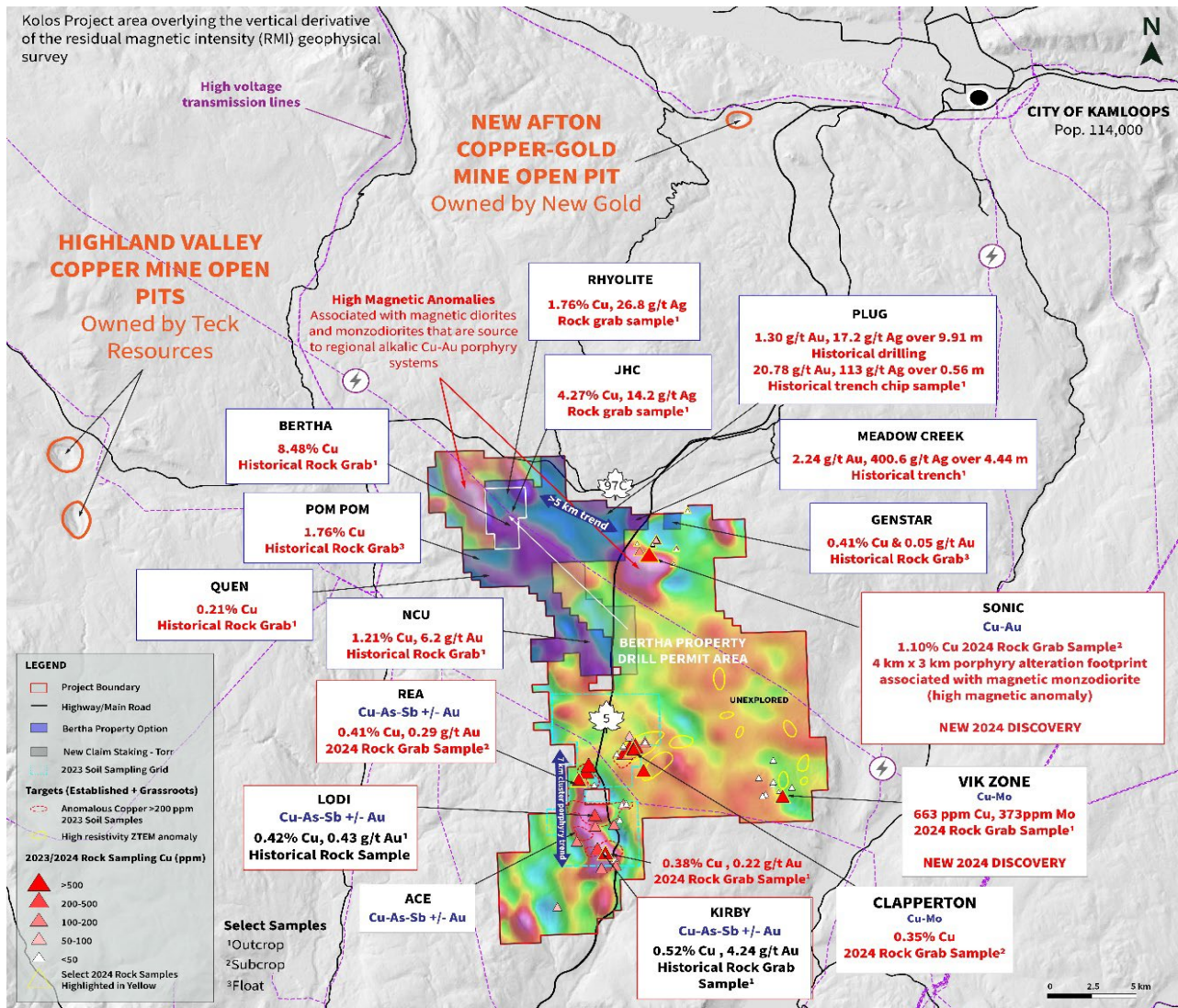
Figure 3. Soil and select rock grab sample results and target locations on the Kolos Project highlighting footprints to highly anomalous Cu in soil (>200 ppm), as well as new Bertha property option and drill permit location with annotated mineral occurrences overlying a regional RMI-VD geophysical survey.
