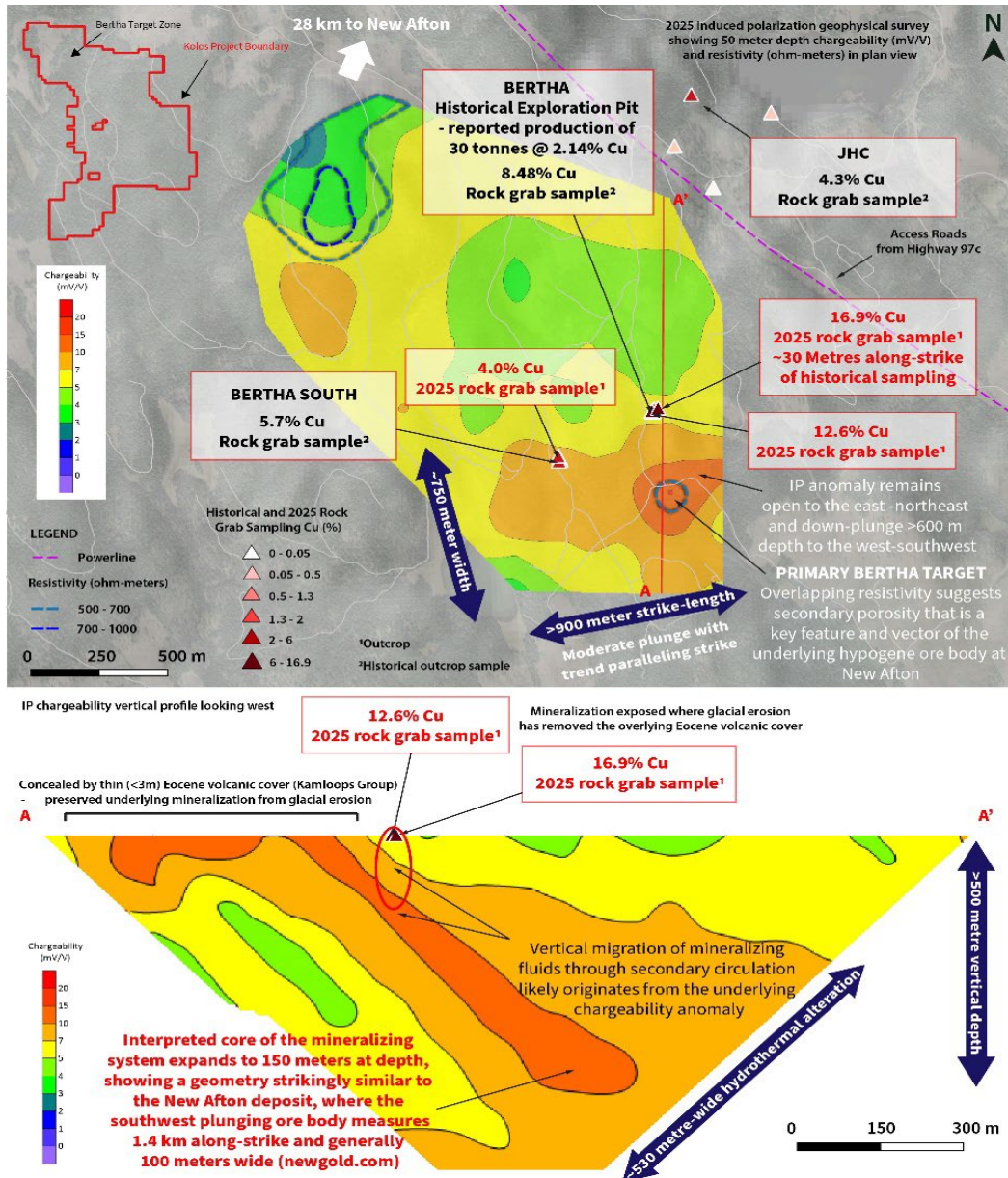
Figure 1. 2025 IP geophysical survey at 50 meters depth (plan view) with select annotated rock grab samples overlying chargeability and resistivity anomalies and depth profile in the Bertha Zone.
