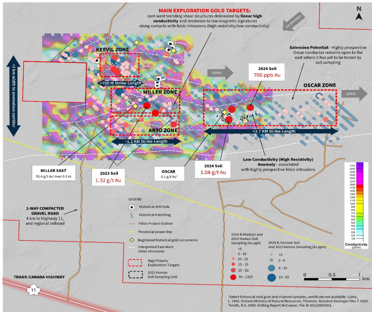
Figure 5. West Filion. A. VLF-EM inversion model displaying conductivity depth slice at 50 meters with annotated interpretations, historical gold occurrences with channel (Miller East) and rock grab sample (Oscar) results, and overlying 2023 humus and 2024 B-horizon soil sampling results.
