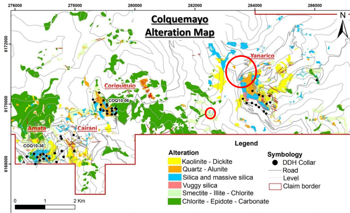
Figure 2 - Colquemayo alteration mapping: Three lithocaps (Amata-Cairani, Coripuquio and Yanarico) were explored between 2009 and 2014 by Rio Tinto and Buenaventura.
