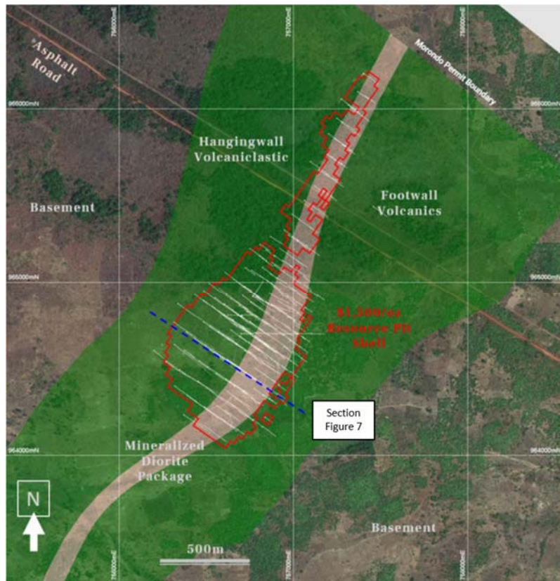
Figure 6: Geology of the Koné Deposit area
