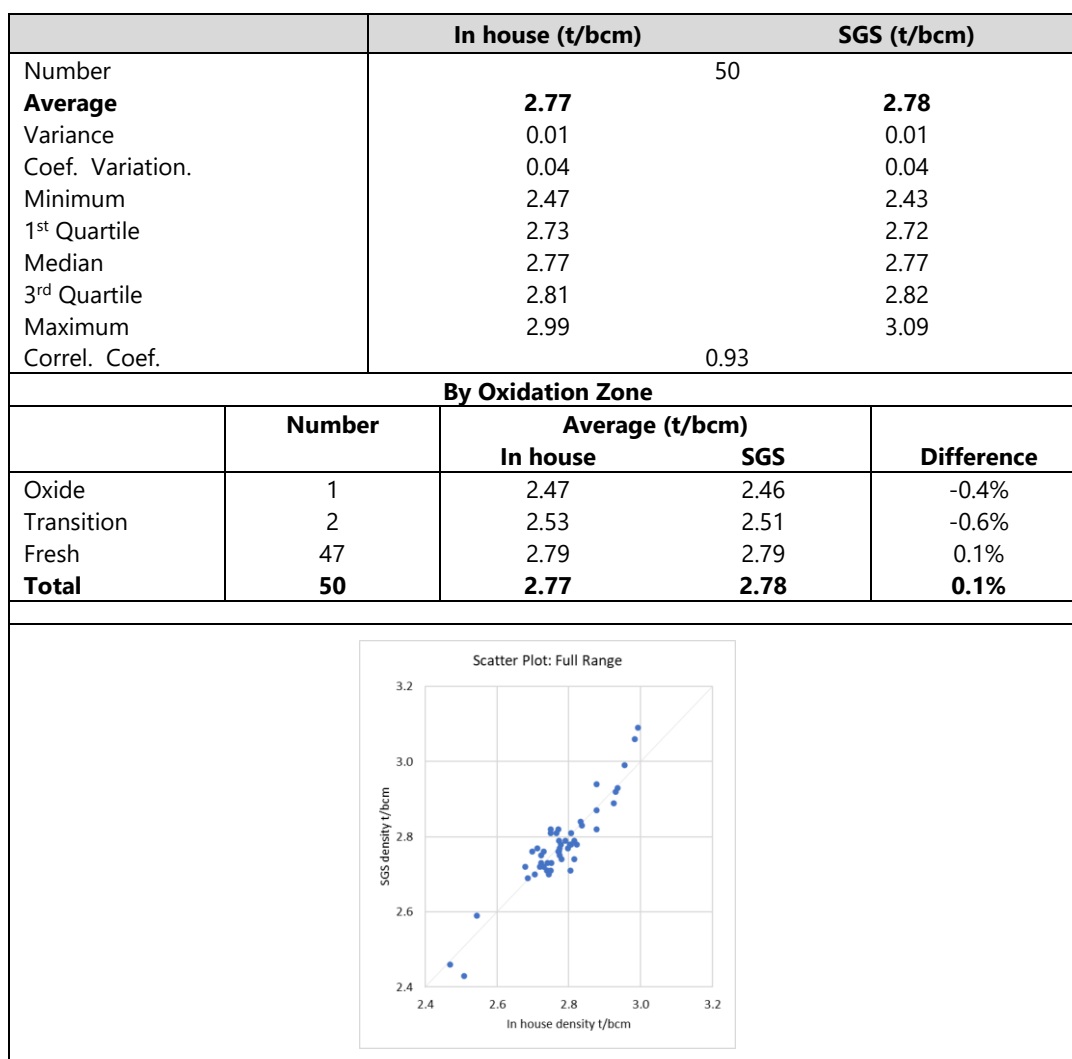
Figure 11-9 SGS versus in house paired density measurements
