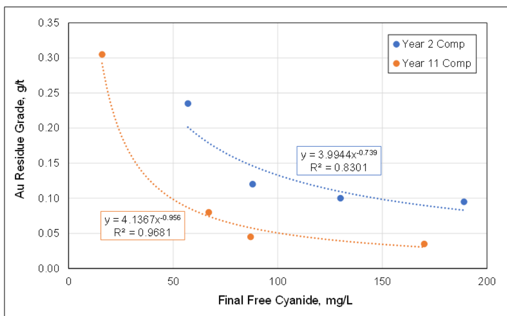
Figure 13-13 Relationship between Free Cyanide and g/t Au in residues
