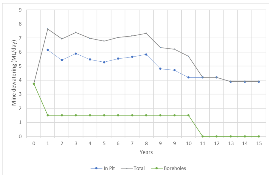
Figure 18-22 Dewatering Volumes
