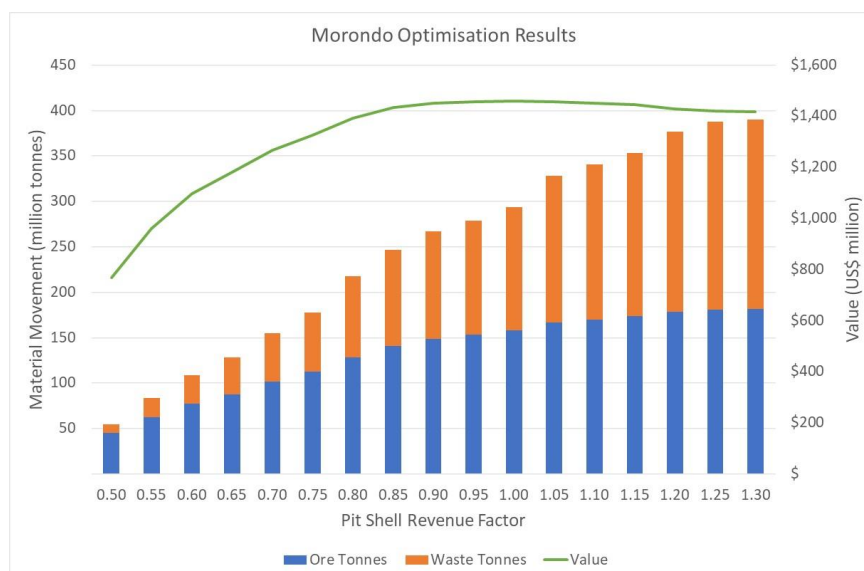
Figure 15-2 Results of Koné Optimisation Study
