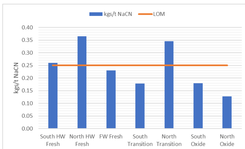
Figure 13-9 Summary of Sodium Cyanide Consumptions
