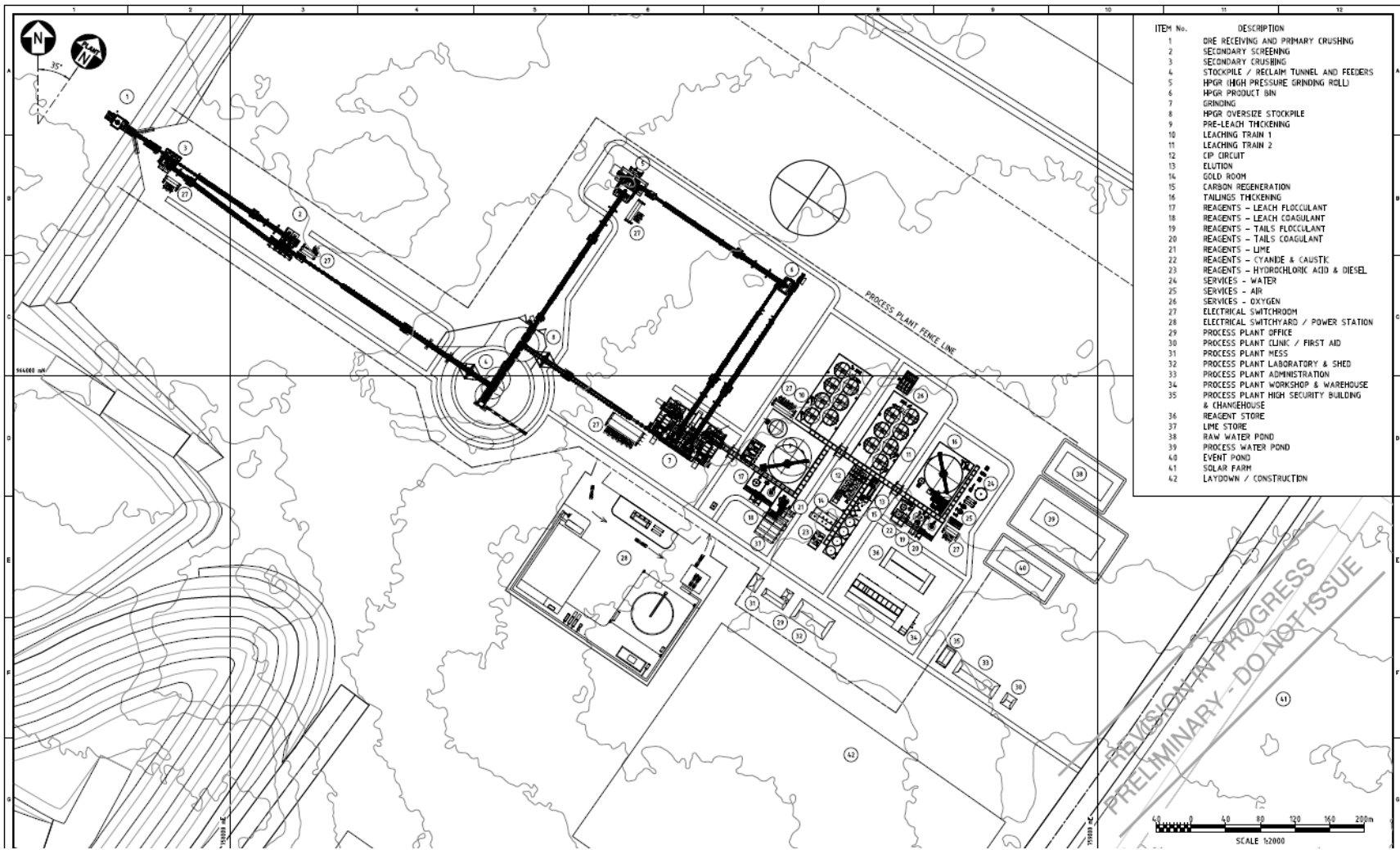
Figure 17-3 Plant Layout
