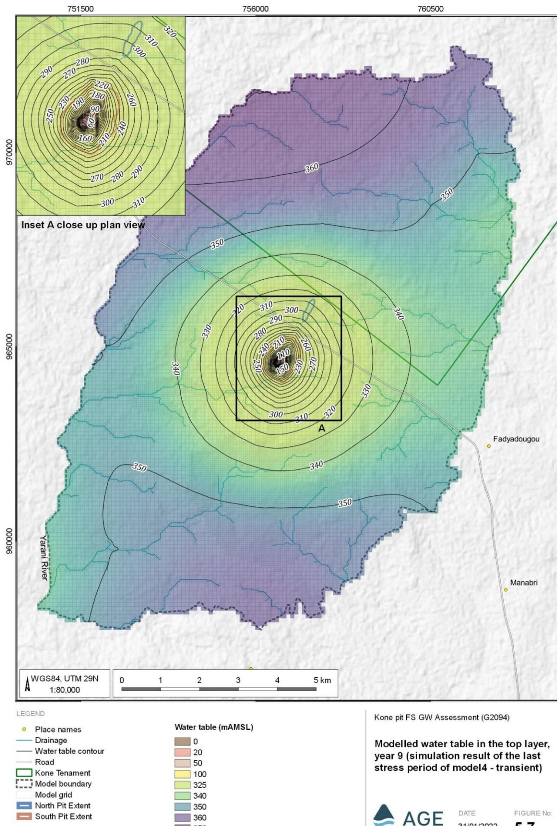
Figure 18-14 Post mining Water Table
