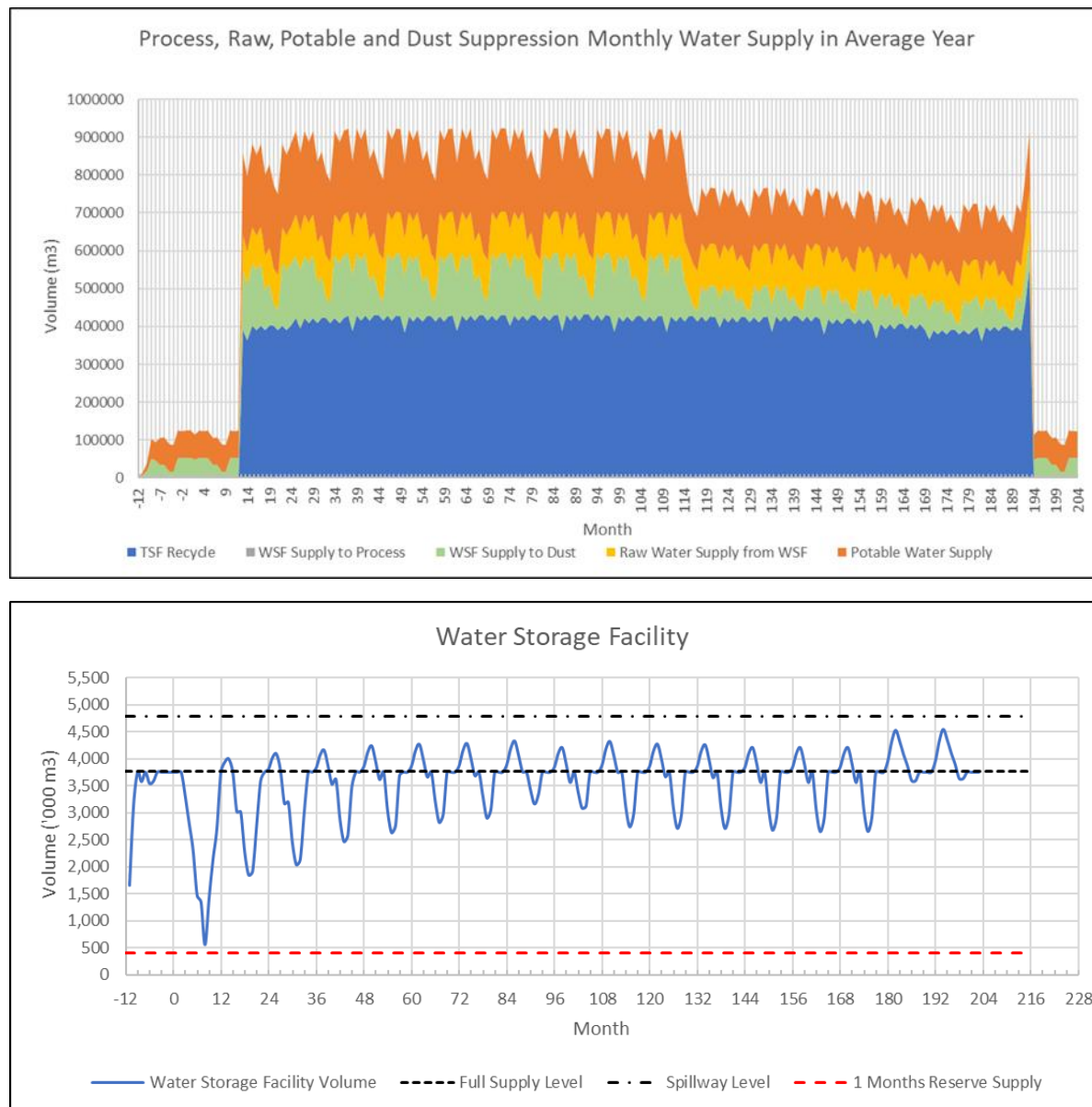
Figure 18-24 Water Balance Results (Average Conditions)
