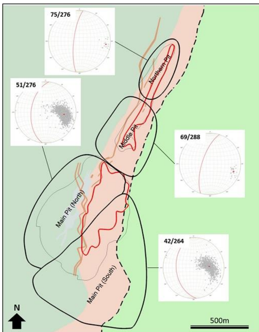
Figure 7-18 Correlation between the dip of the foliation and the strike of the host rocks
