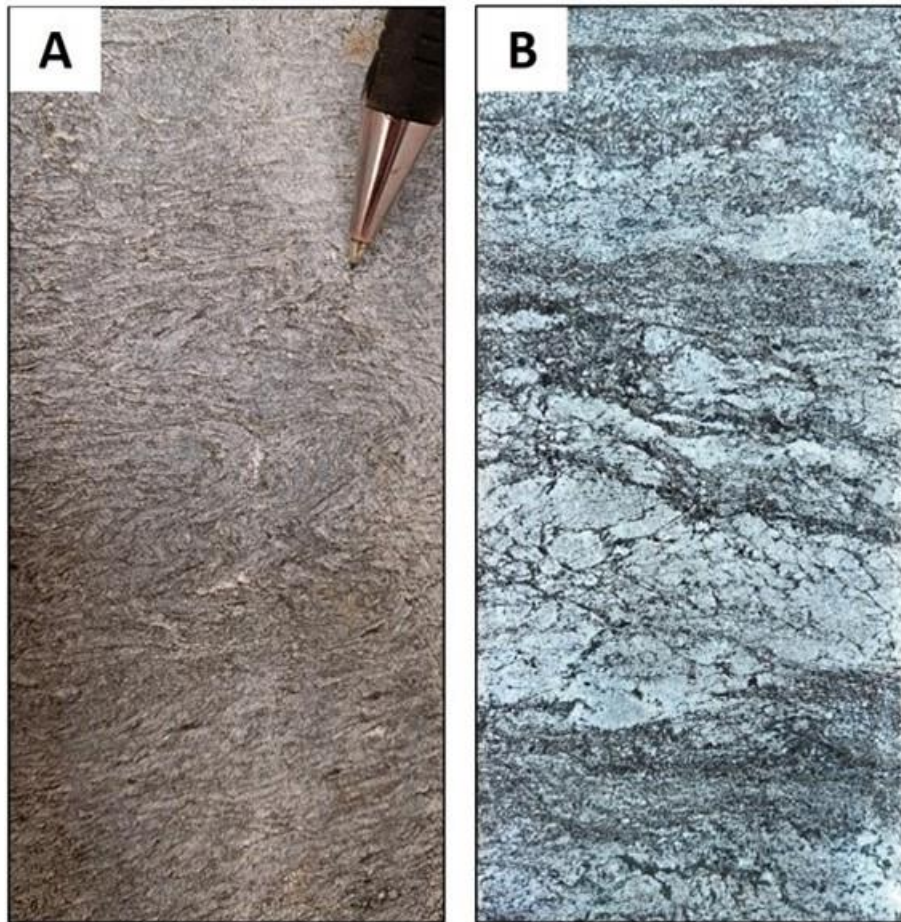
Figure 7-16 Ductile shear within diorite
