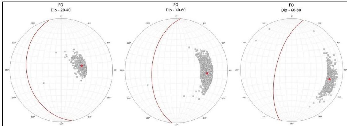
Figure 7-19 Stereo-nets of foliations
