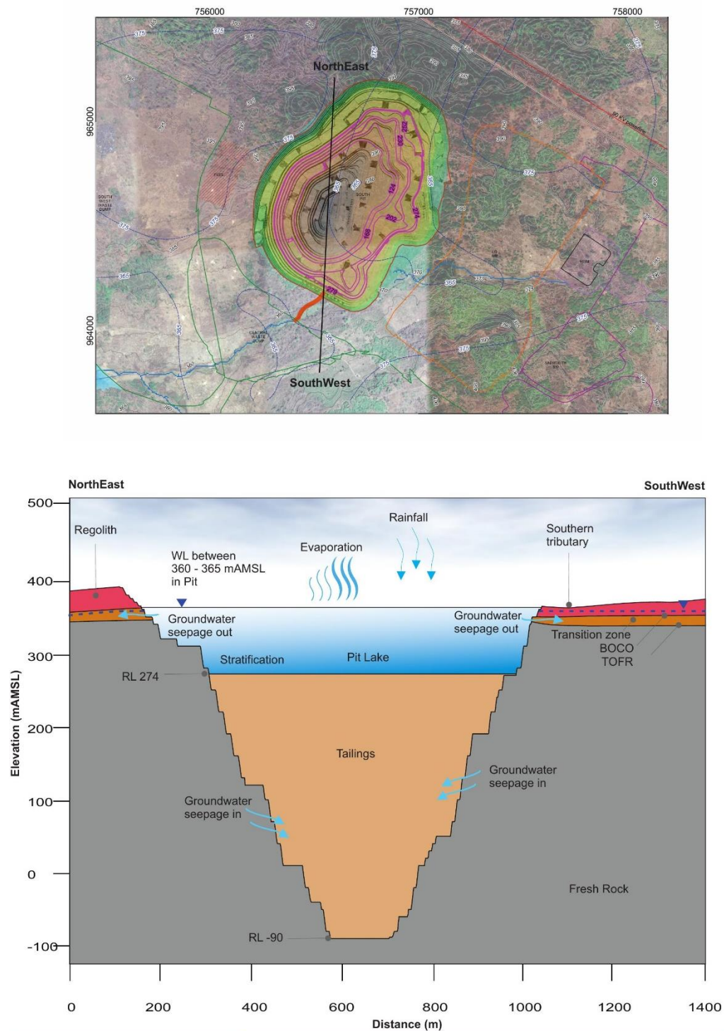
Conceptual pit hydrogeology model 17- 25 y post closure
