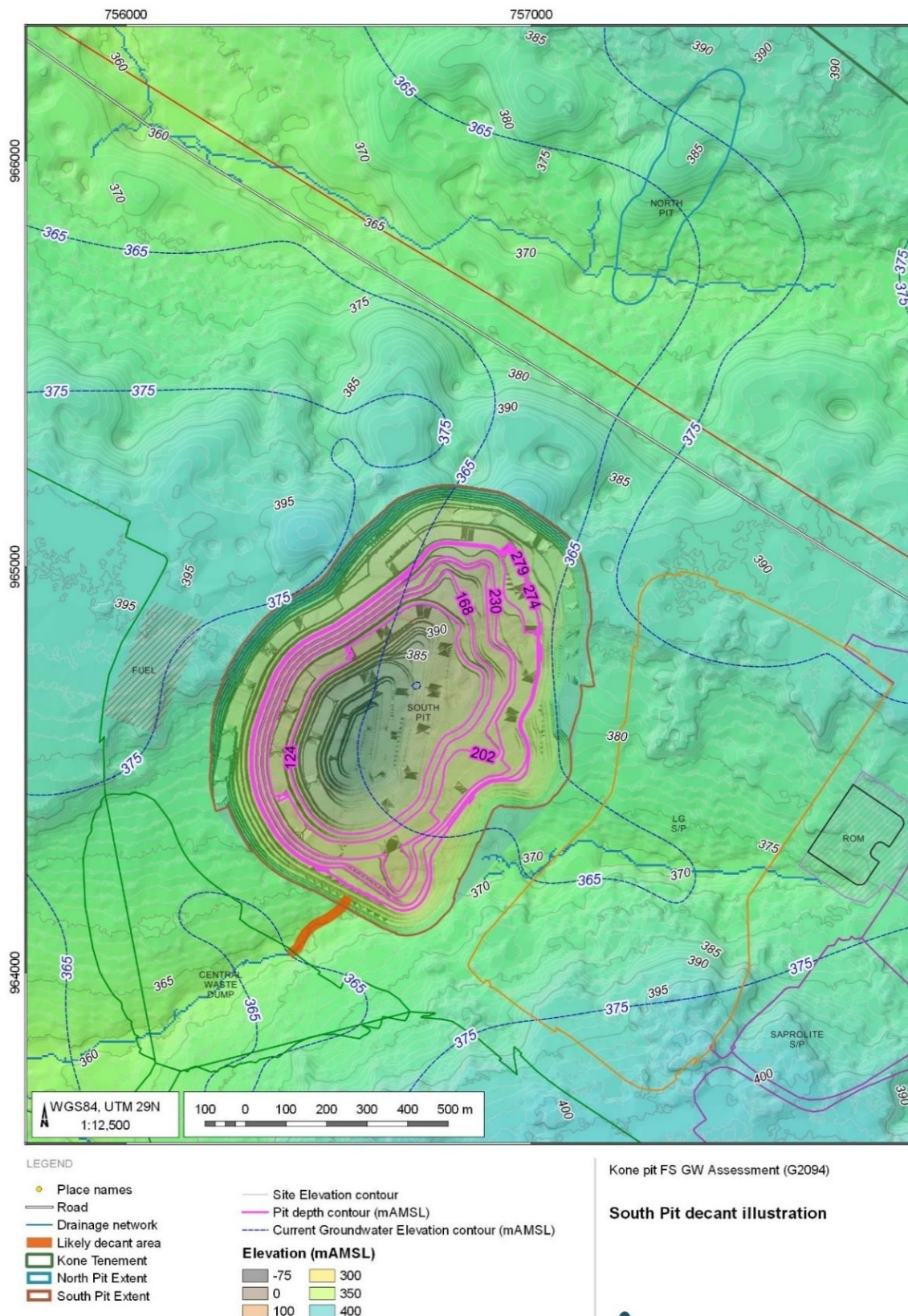
Figure 18-17 South Pit decant
