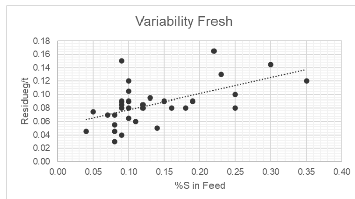
Figure 13-2 Fresh Samples Head Sulphur and Residue Gold Grade
