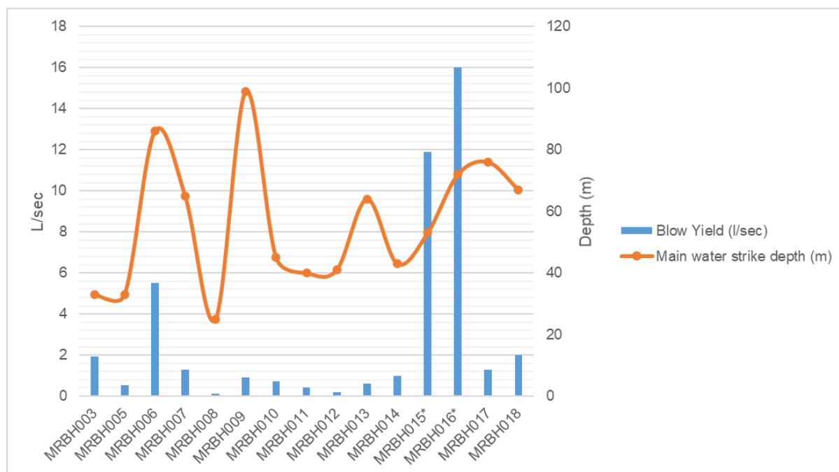
Figure 18-8. Blow Yields Observed During Drilling
