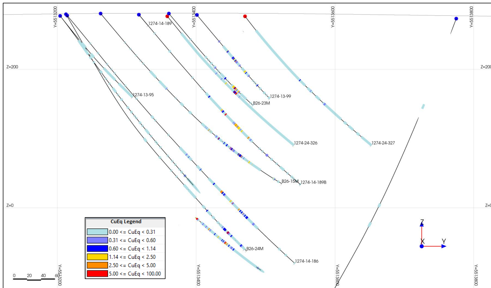
Figure 10-5 Typical Cross-Section (652,700 mE) with CuEq Colors
