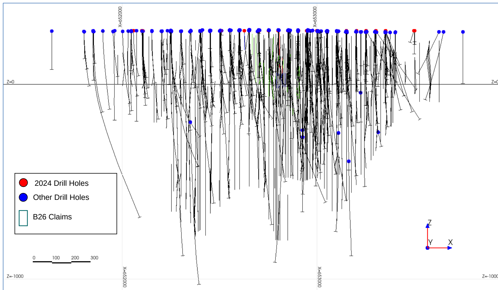
Figure 10-4 Longitudinal View to the North of the Drill Holes in the B26 Mineralization Area
