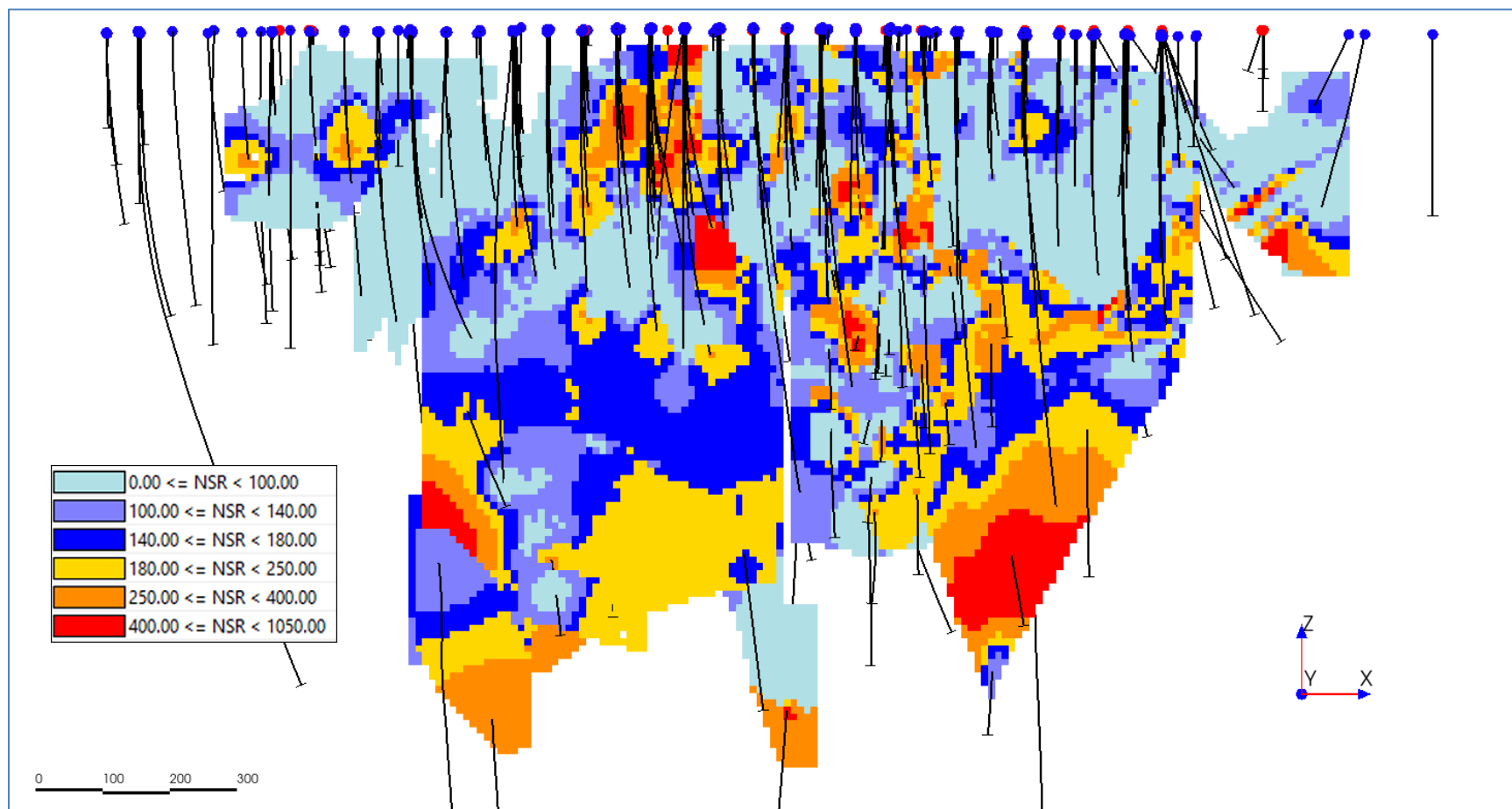
Figure 14-18 Block Model Resource Estimates with Overlay of Cu, Zn, Ag Zones
