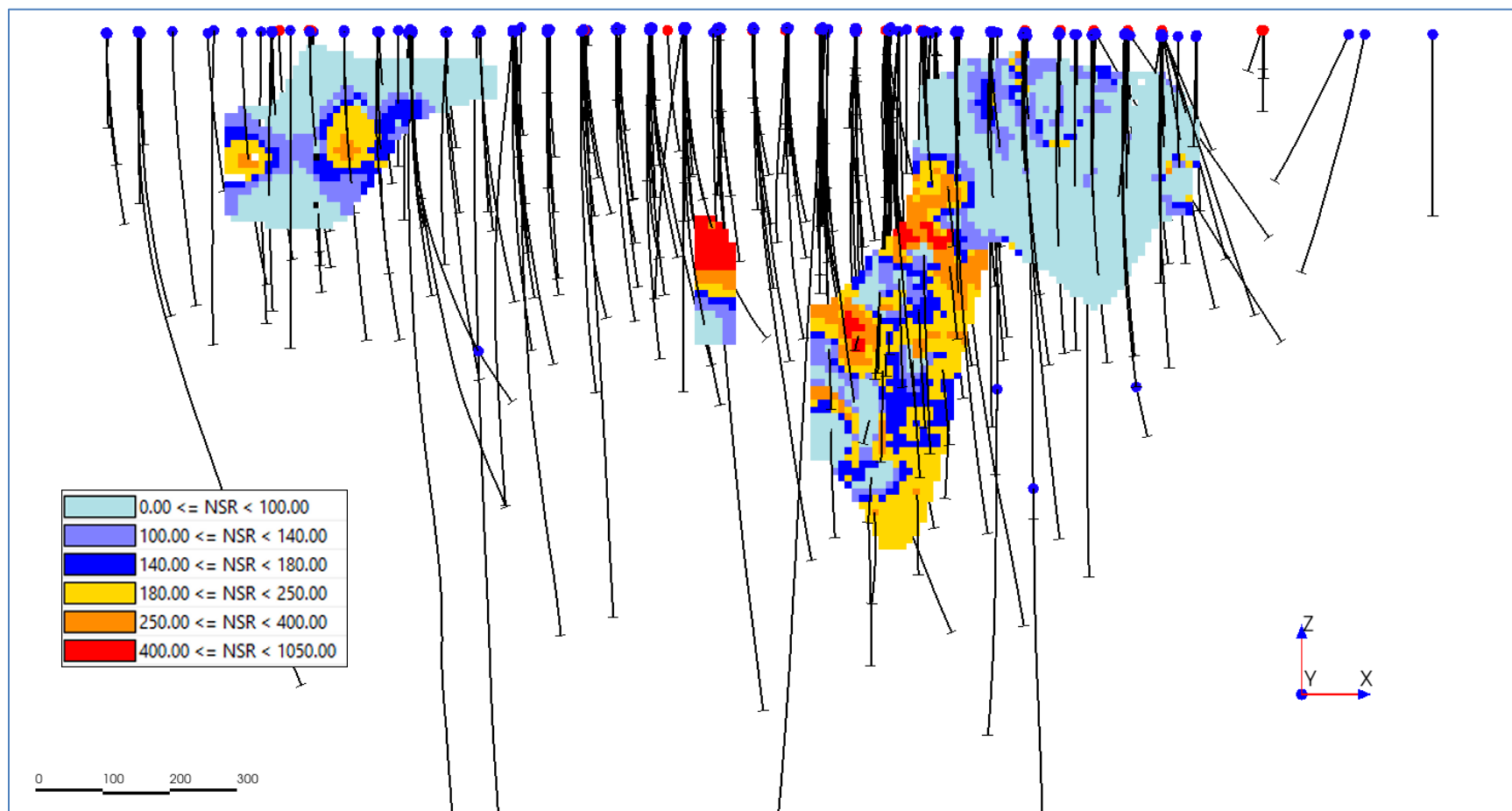
Figure 14-16 Longitudinal View to the North Showing the Blocks of the Zn Zone
