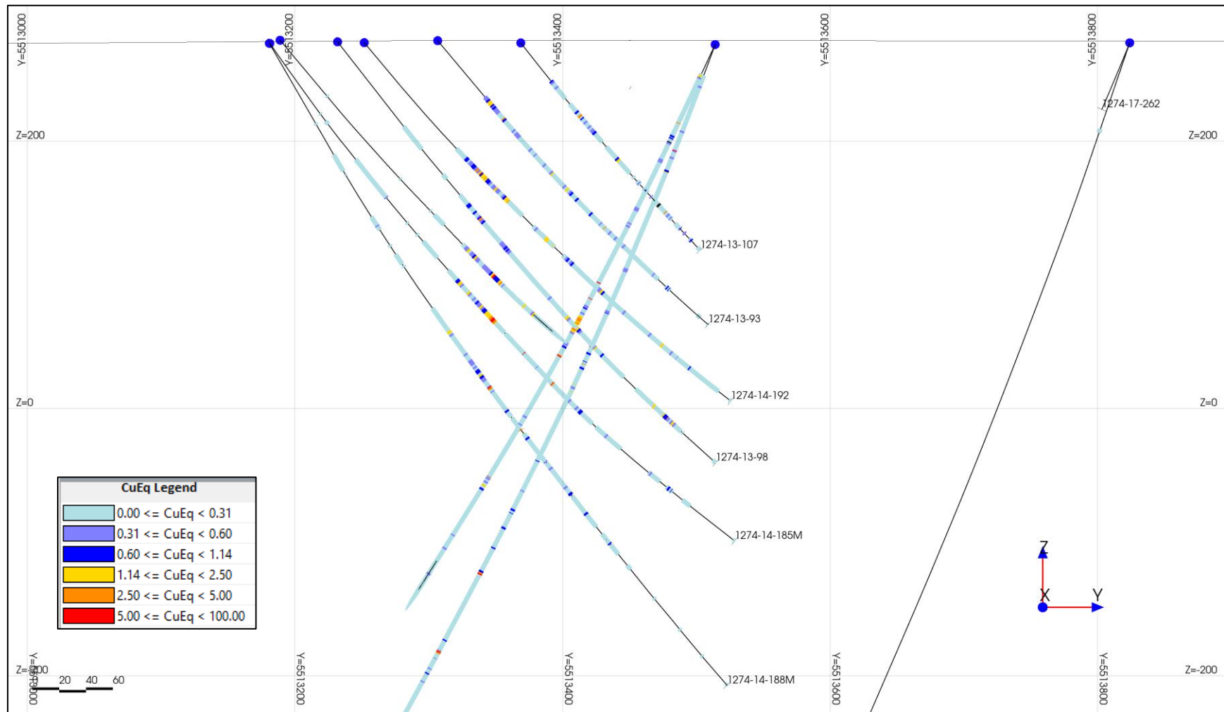
Figure 10-6 Typical Cross-Section (653,100 mE) with CuEq Colors
