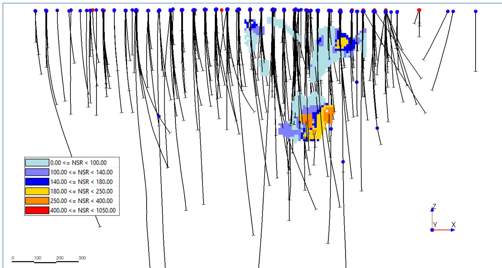
Figure 14-17 Longitudinal View to the North Showing the Blocks of the Ag Zone
