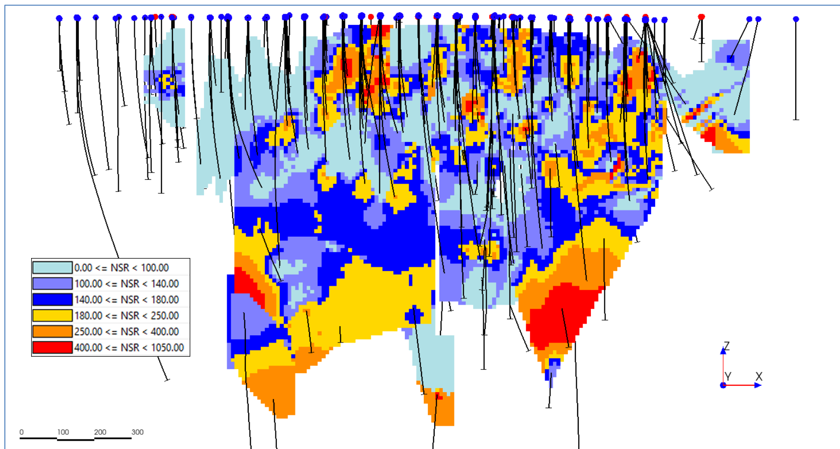
Figure 14-15 Longitudinal View to the North Showing the Blocks of the Cu Zone
