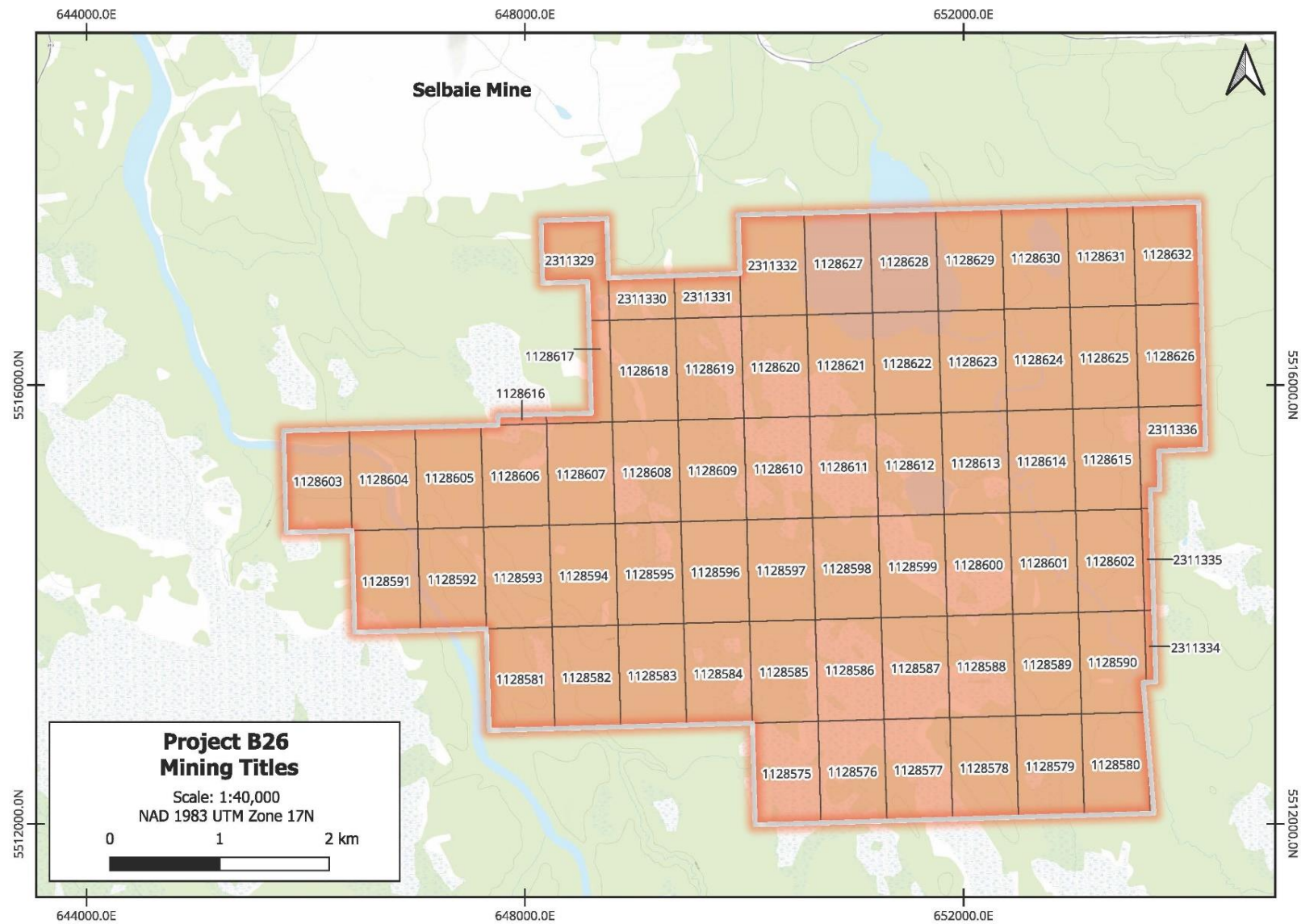
Figure 4-2 Location of the B26 Brouillan Mining Claims
