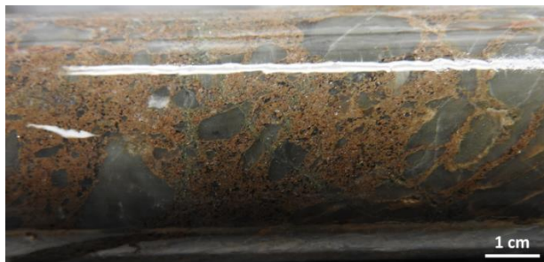
Figure 7-38 Sphalerite-Pyrite-Galena-Ag Breccia in the Aphyric Rhyolite, Drill Hole 1274-17-249 at 500 m
