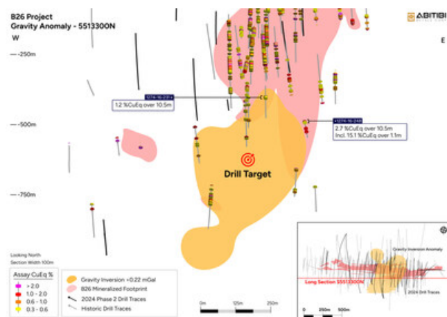
Figure 2: Gravity Anomaly 5513300N (CNW Group/Abitibi Metals Corp.)
