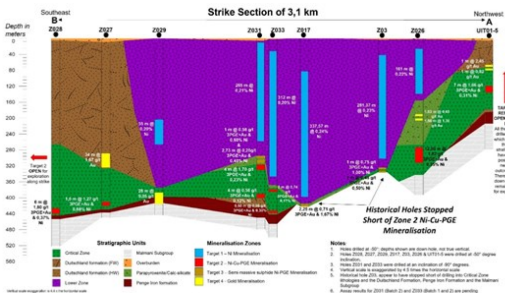
Figure 3: Cross-section along lines A – B demonstrating the continuity of Ni-Cu-PGE mineralisation within Zone 2 beneath the Lower Uitloop body. The central portion of the section highlights consistent intersections of semi-massive Ni-PGE mineralisation. Notably, historical boreholes Z03 and Z017 were terminated prematurely, before intersecting the full extent of the Ni-Cu-PGE mineralisation package.
