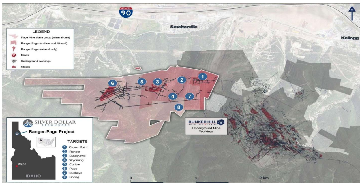
Figure 3: Ranger-Page claim groups, underground mine workings, and new target areas
