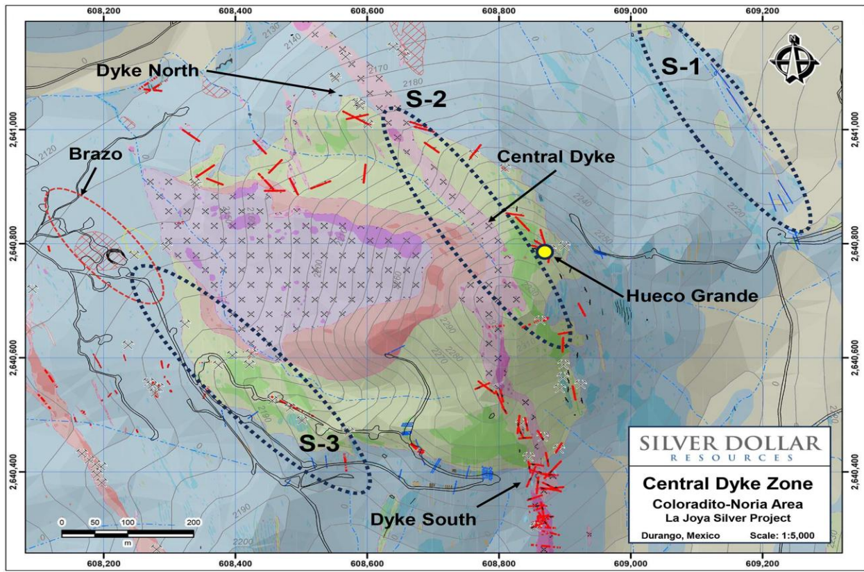
Figure 8: Coloradito-Noria geology, MAG anomalies, and target areas
