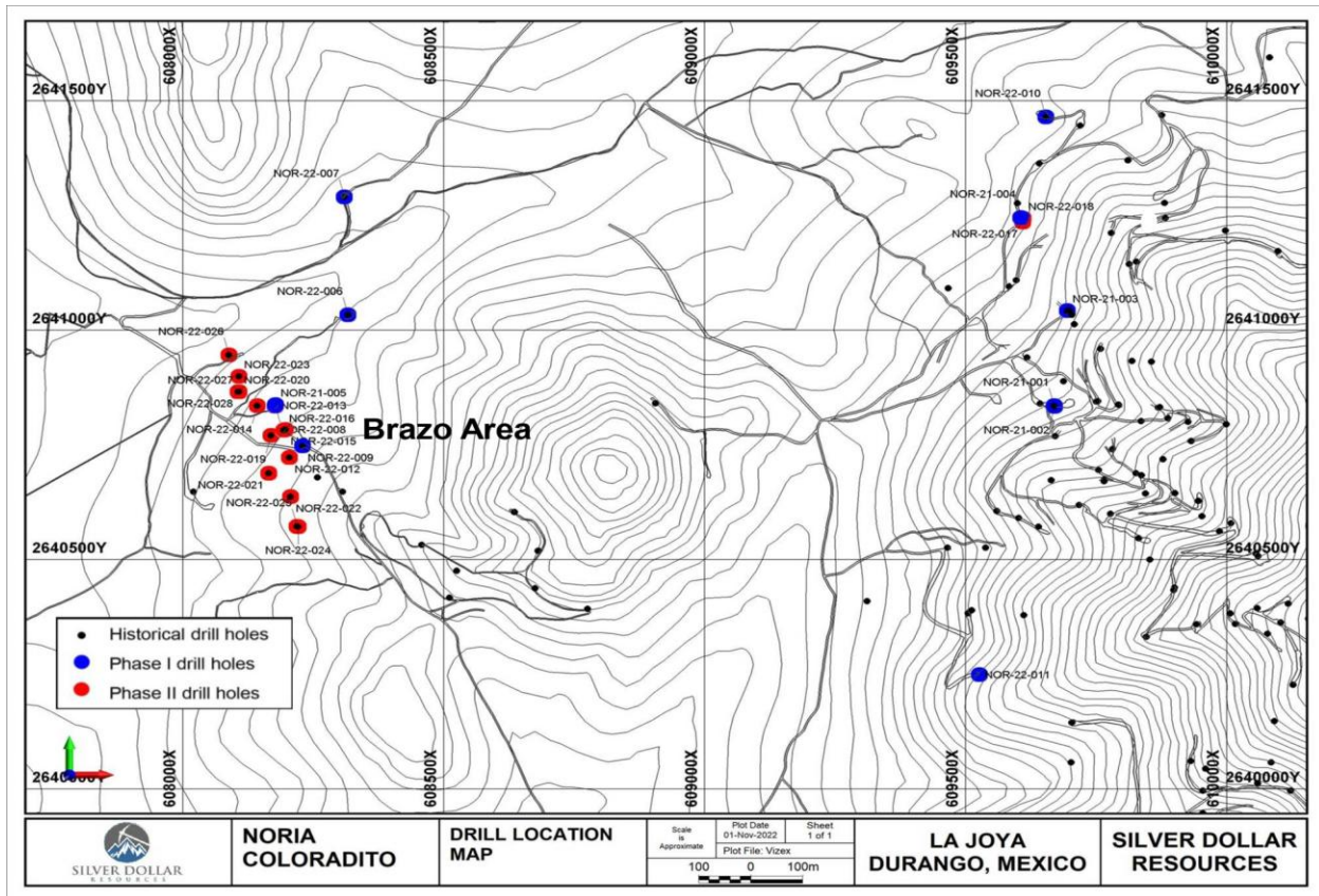
Figure 7: Location of Silver Dollar's Brazo discovery and Phase I and II drill holes
