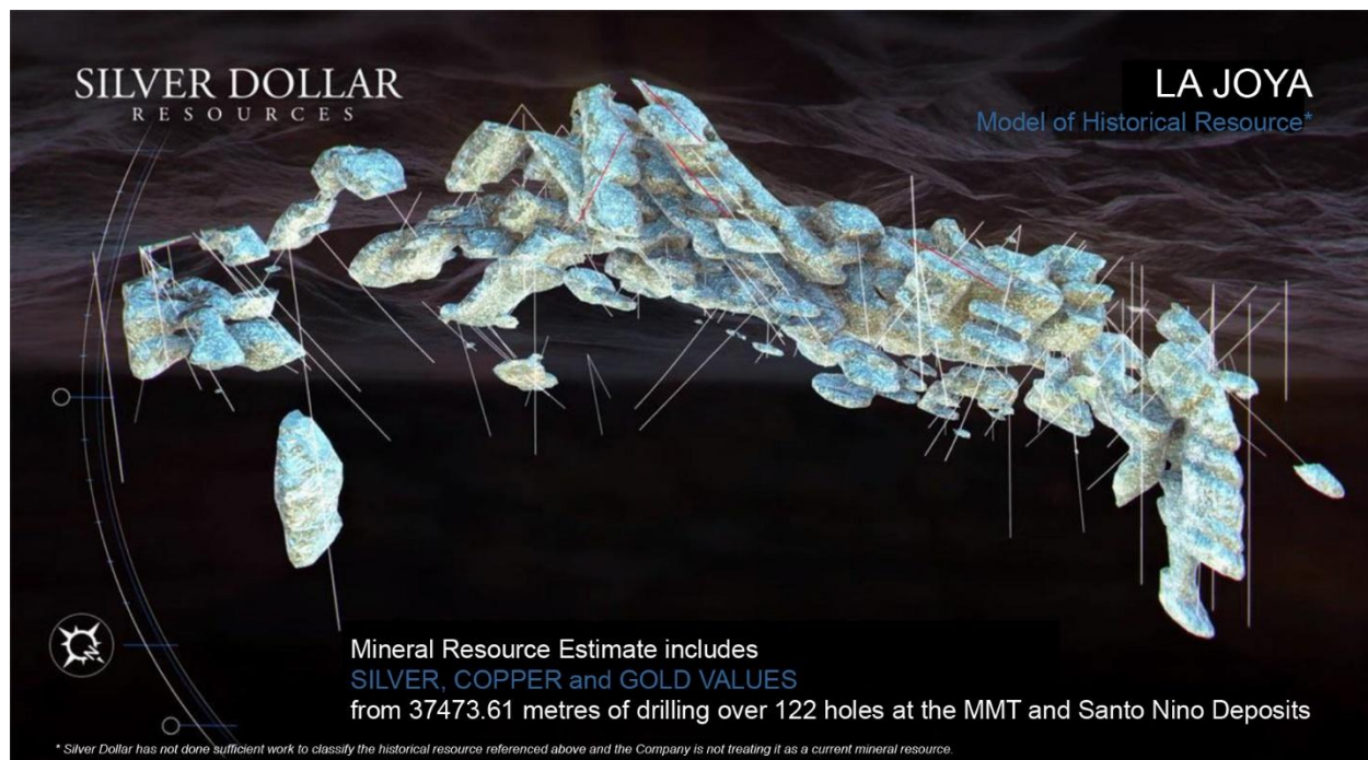
Figure 6: Model of historical mineral resources for the MMT and Santo Nino deposits
