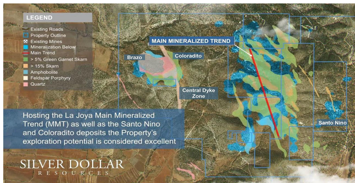
Figure 5: Planview of the MMT, Santo Nino and Coloradito deposits, and Brazo and Central Dyke zones
