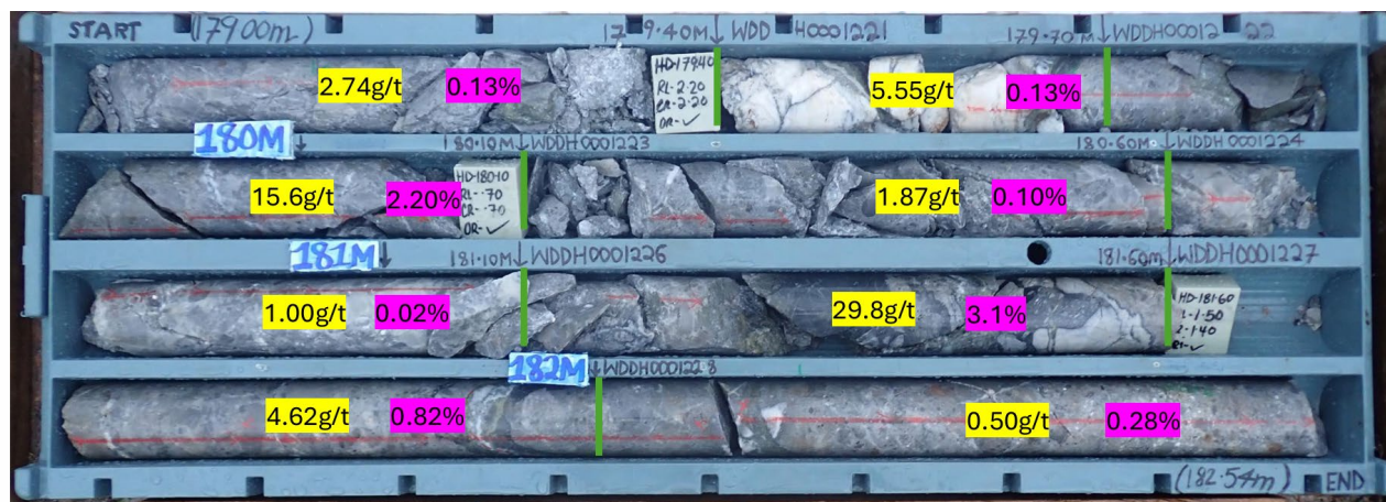
Figure 2: WDG-12 core from 179.0–182.54 m (Zone 2) showing quartz–sulphide breccia with strong gold and copper grades up to 29.8 g/t Au and 3.1% Cu.
