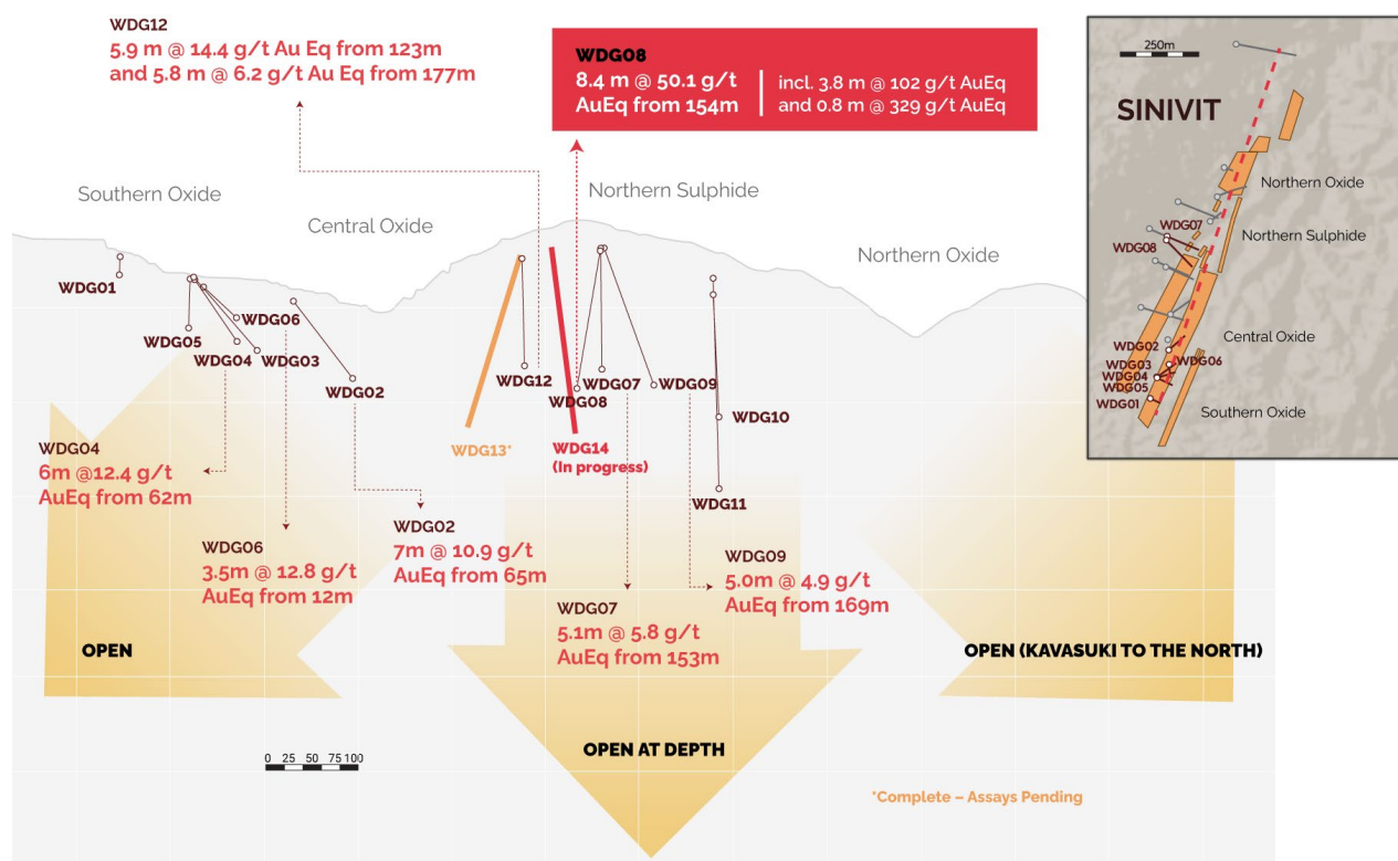
Figure 5: Long section through the Sinivit target area showing drilling completed to-date with key intervals.
