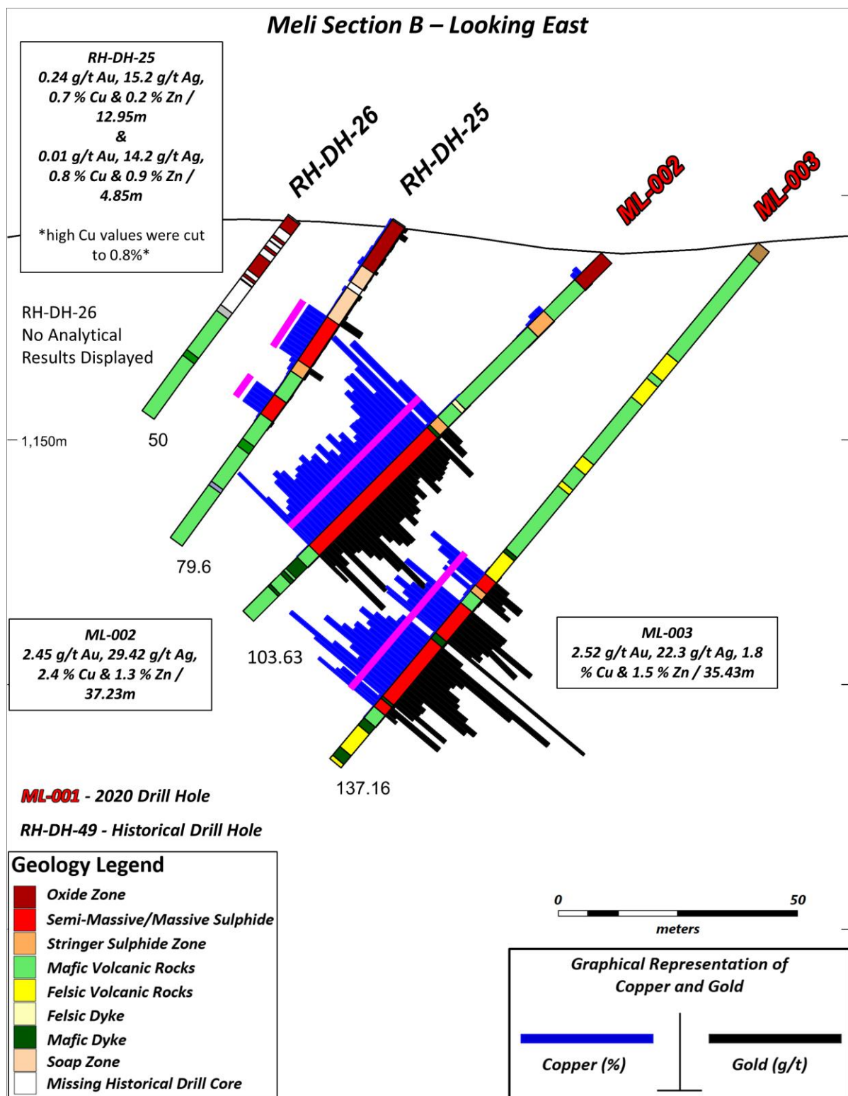
Figure 10-3 Meli diamond drill section B
