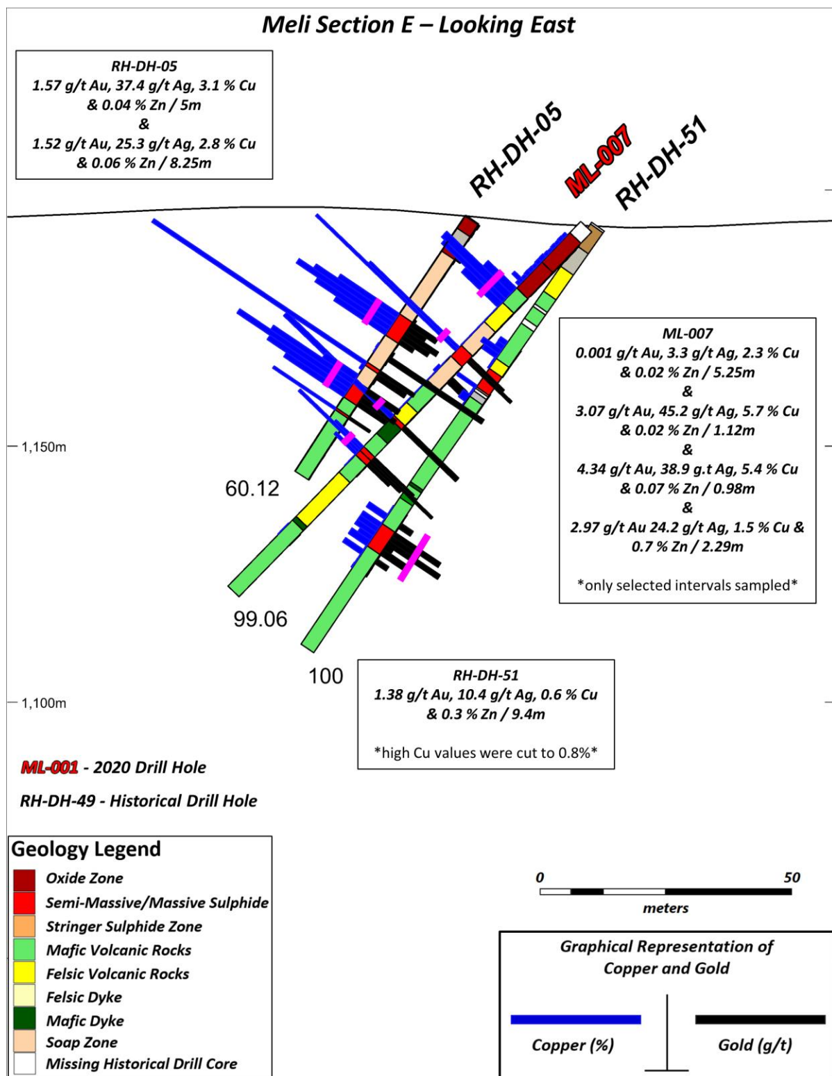
Figure 10-6 Meli diamond drill section E
