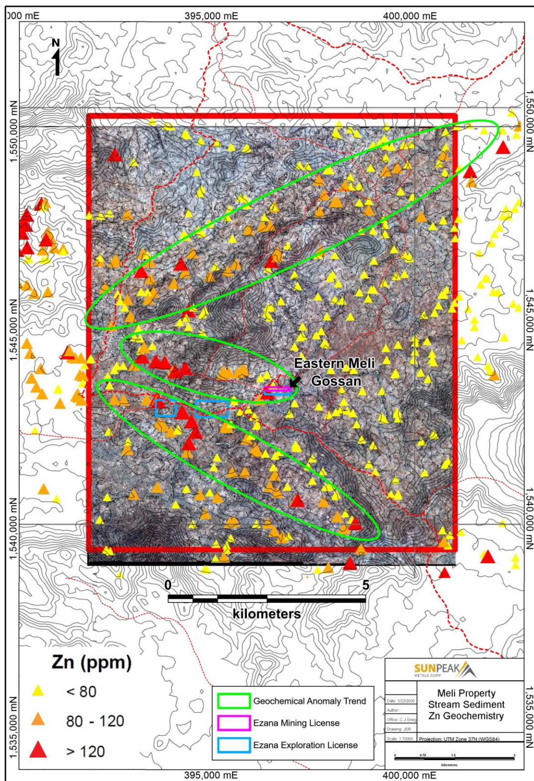
Figure 6-1 Meli concession area stream sediment Zn geochemistry (source: Ezana private report)
