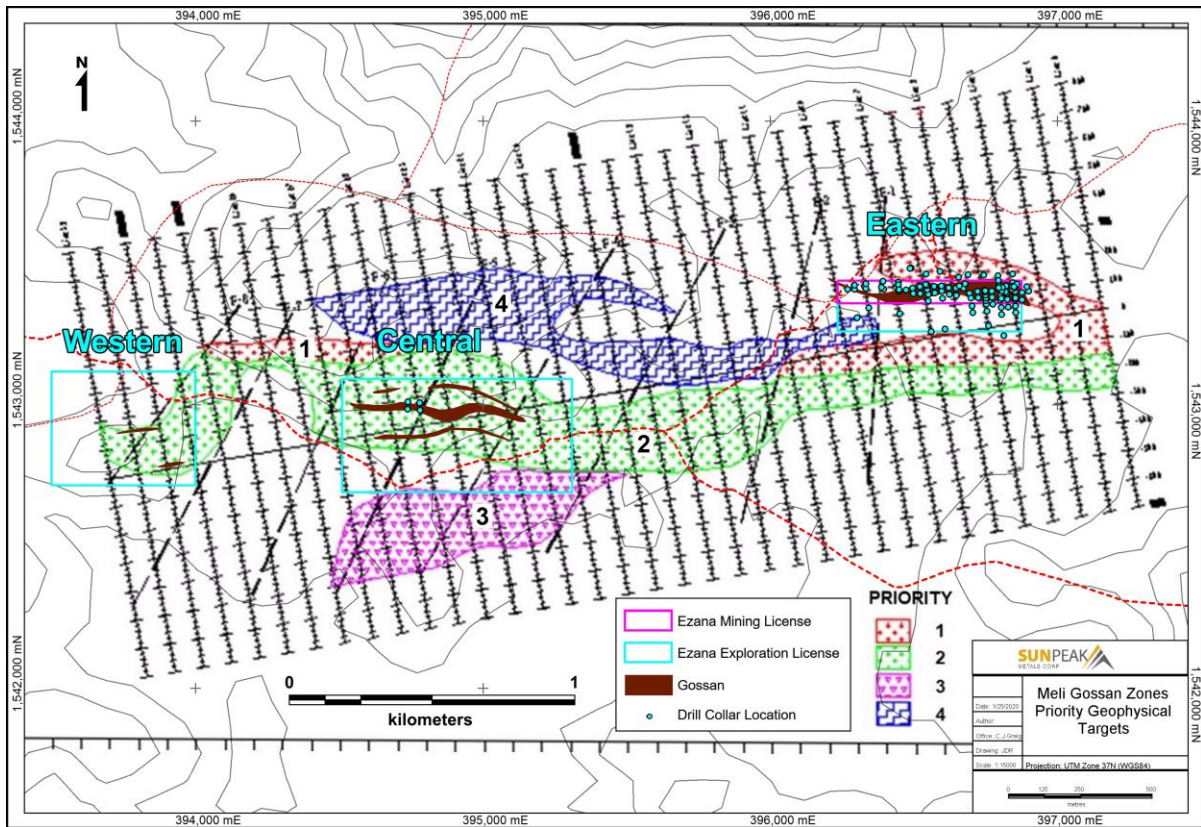
Figure 6-8 Priority geophysical targets in the area of Meli gossan zones (source: Lul Earth Sciences, 2007)
