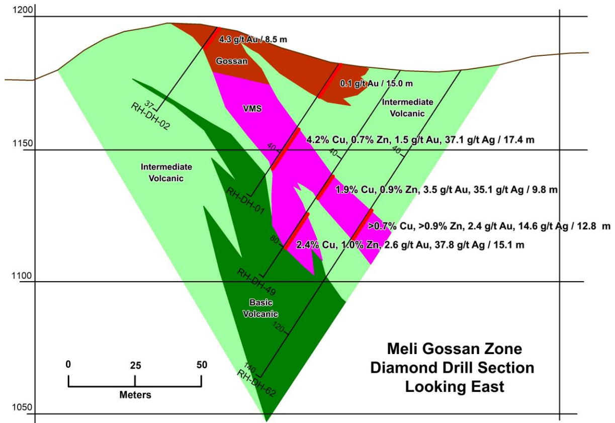
Figure 6-9 Eastern Meli gossan zone drill section looking east (source: Ezana private company report)
