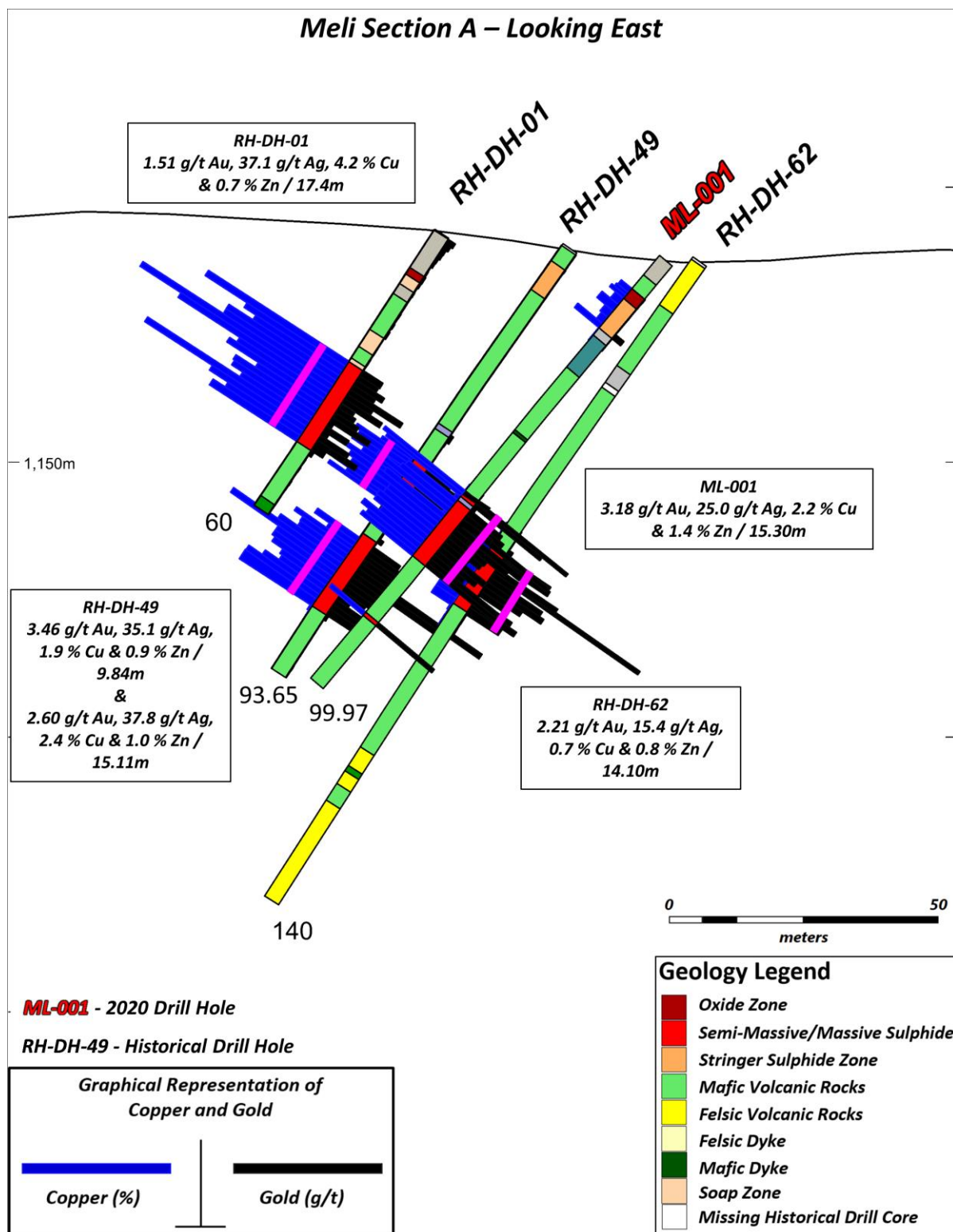
Figure 10-2 Meli diamond drill section A
