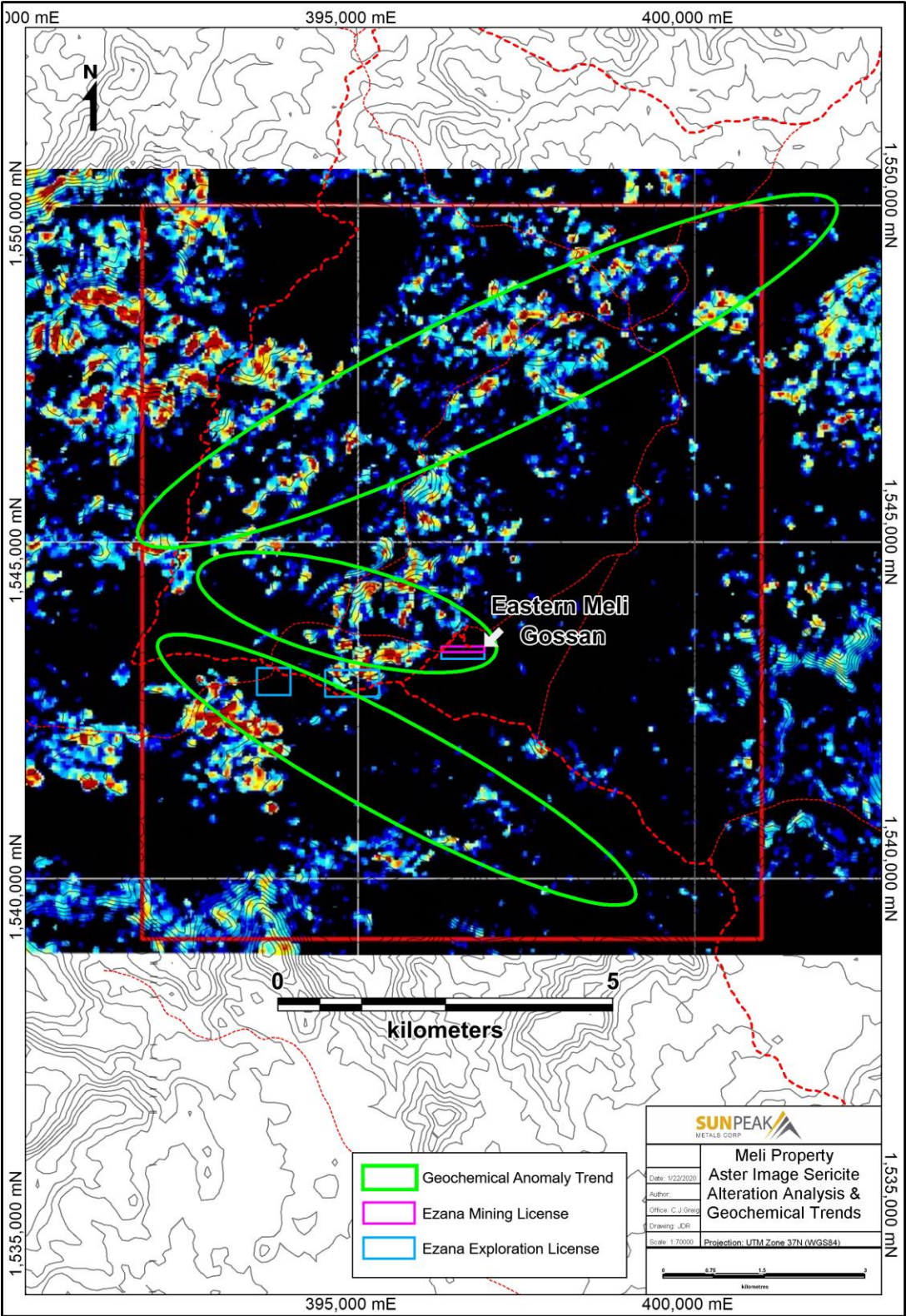
Figure 9-1 Aster image sericite analysis with anomalous geochemical trends
