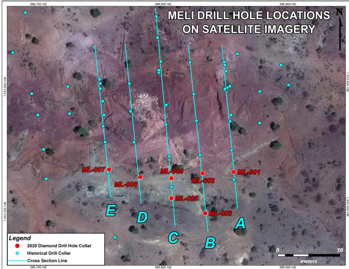
Figure 10-1 Meli Eastern gossan drill hole collar locations and cross section lines
