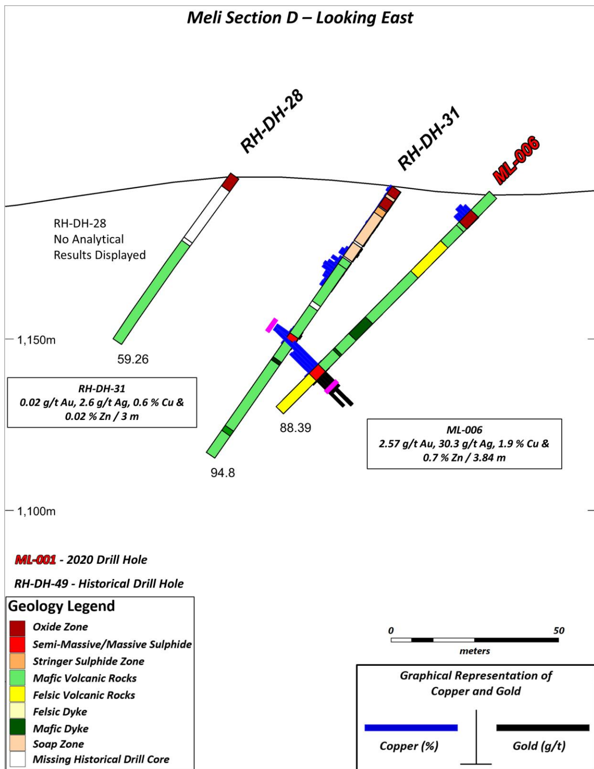
Figure 10-5 Meli diamond drill section D
