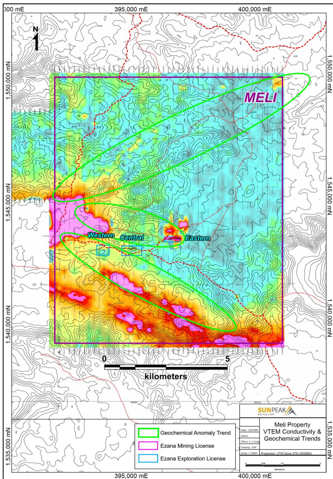
Figure 9-3 Meli concession with mineral showing areas and VTEM conductor anomalies (warmer colours represent higher conductivity)
