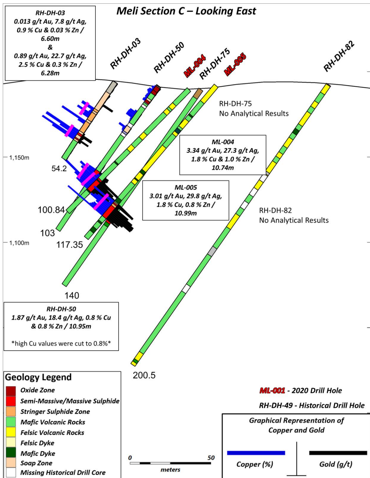
Figure 10-4 Meli diamond drill section C
