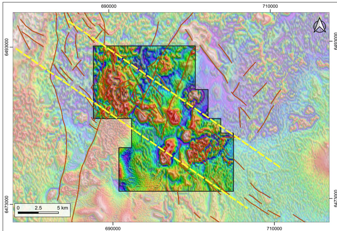
Figure 3: Mendooran targets on total magnetic intensity map with reduced-to-pole filters. Regional magmatic complex situated on the under-cover extension of the northern MVB coincident with corridor of northwest trending magnetic features (Yellow) interpreted to represent potential intrusive related copper-gold targets. Figure shows exploration license (Black lines) with the structural interpretation (Red lines).
