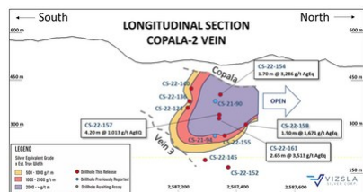
Figure 2: Longitudinal Section of the Copala 2 vein. (CNW Group/Vizsla Silver Corp.)
