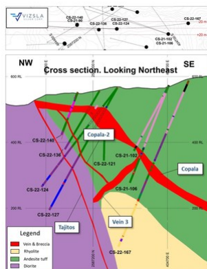
Figure 3: Cross section showing Tajitos, Copala and Copala 2 veins. (CNW Group/Vizsla Silver Corp.)
