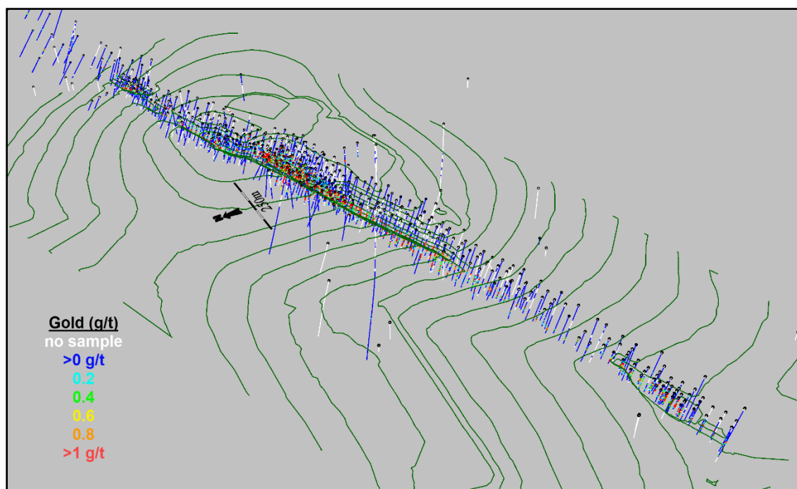
Figure 14.5: Isometric View of Gold Data in Drilling following Treatment of Unsampled Intervals
