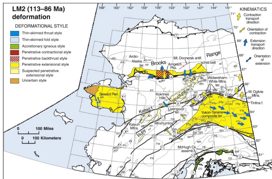
Figure 7.3: West-Central Alaska Deformation 113–86 Ma
