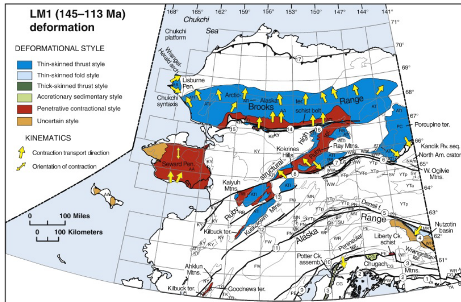
Figure 7.2: West-Central Alaska Deformation 145–113 Ma
