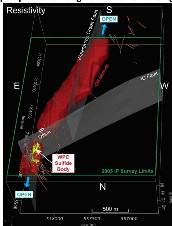
Figure 9.15: South-looking View of the <30-ohm IP resistivity anomaly looking from Waterpump Creek through the Last Hurrah target area
