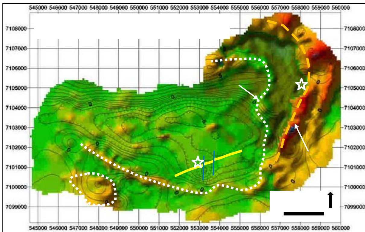
Figure 6.2: Total Field Magnetics (Aerodat, 1984) and Regional Gravity Survey (Edcon, 1983)
