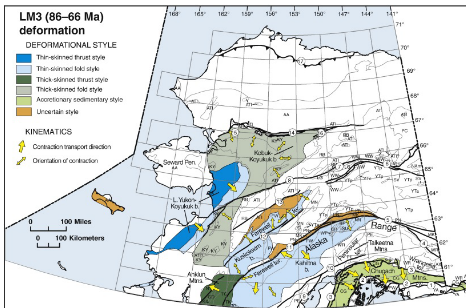
Figure 7-4: West-Central Alaska Deformation 86–66 Ma
