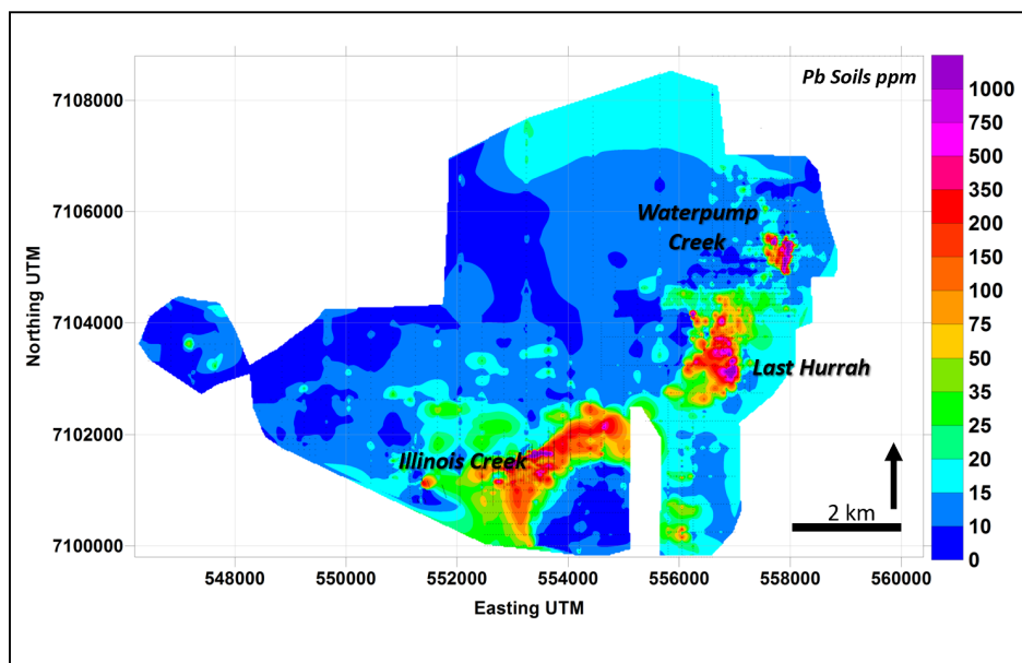
Figure 9.1: Lead Soil Geochemistry – Illinois Creek Property
