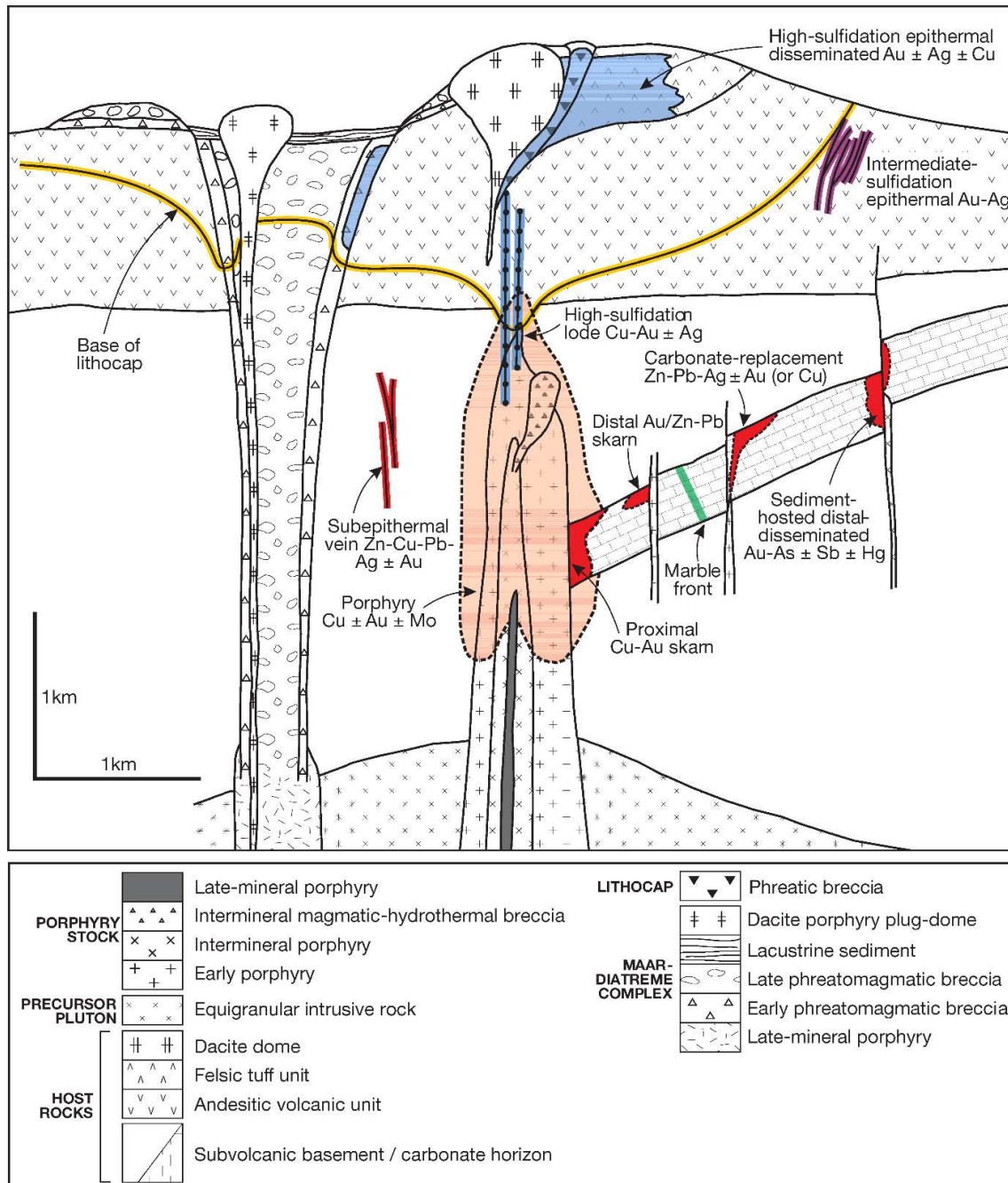
Figure 12: Deposit Model
