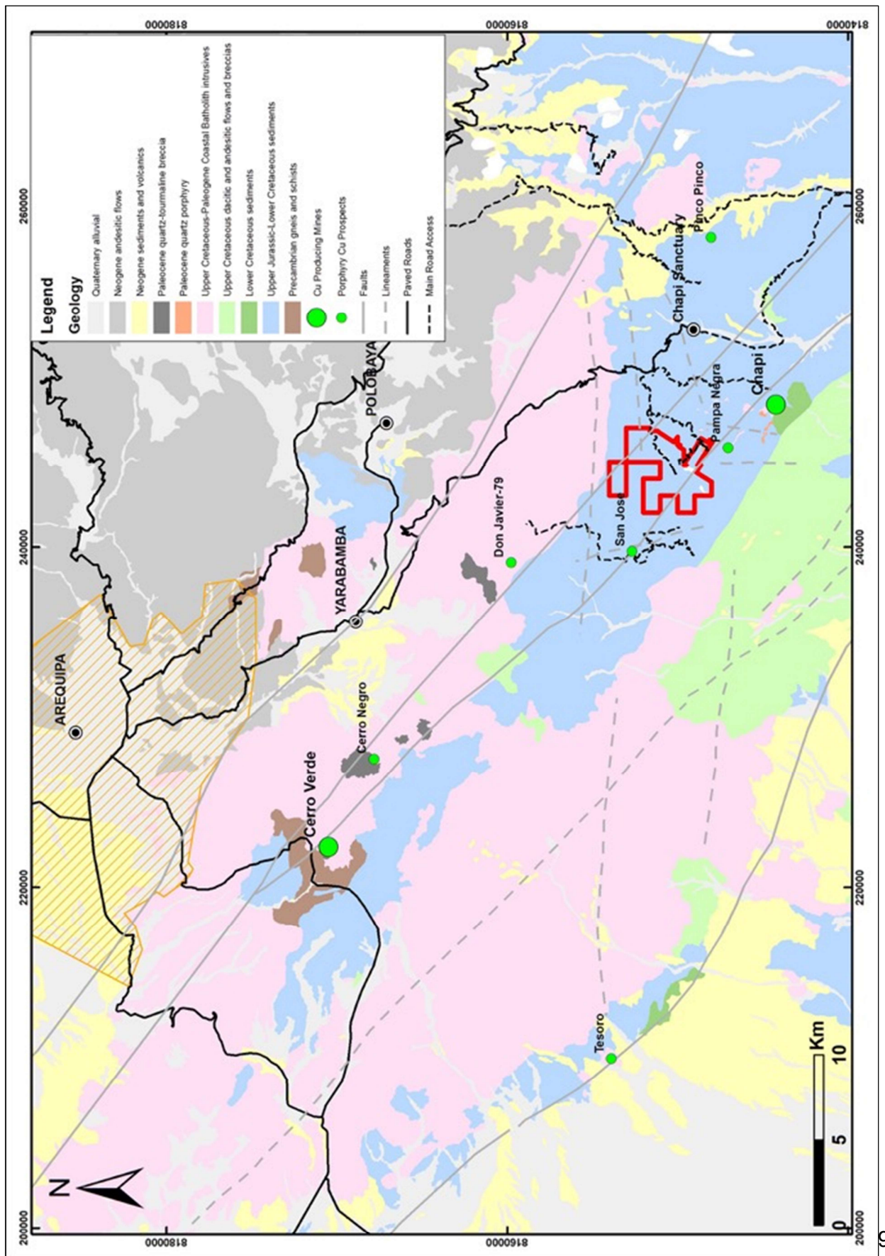
Figure 7: Geology
