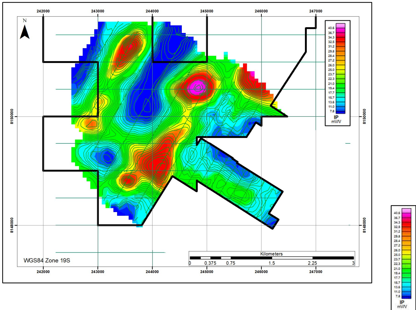
Figure 15: Chargeability at Surface
